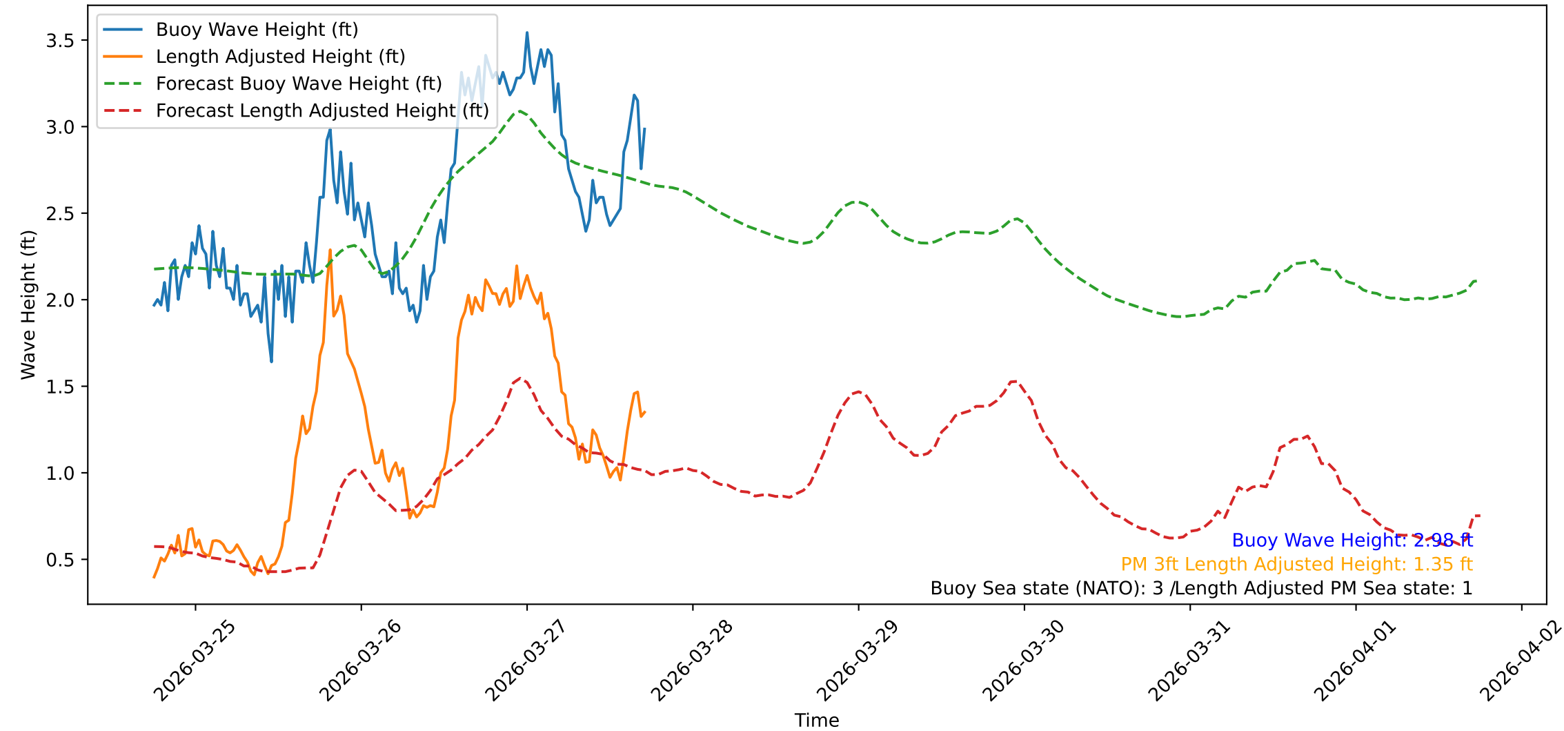
Wave Heights over Time for Green Beach at 2026-03-27 17:51:08
