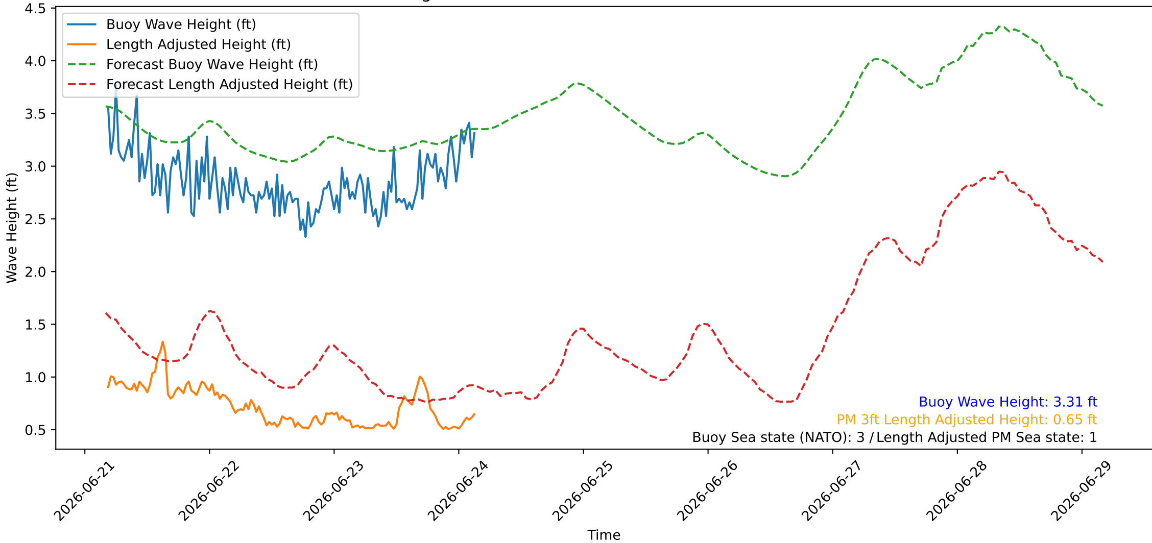
Wave Heights over Time for Red Beach at 2026-06-24 04:00:45
