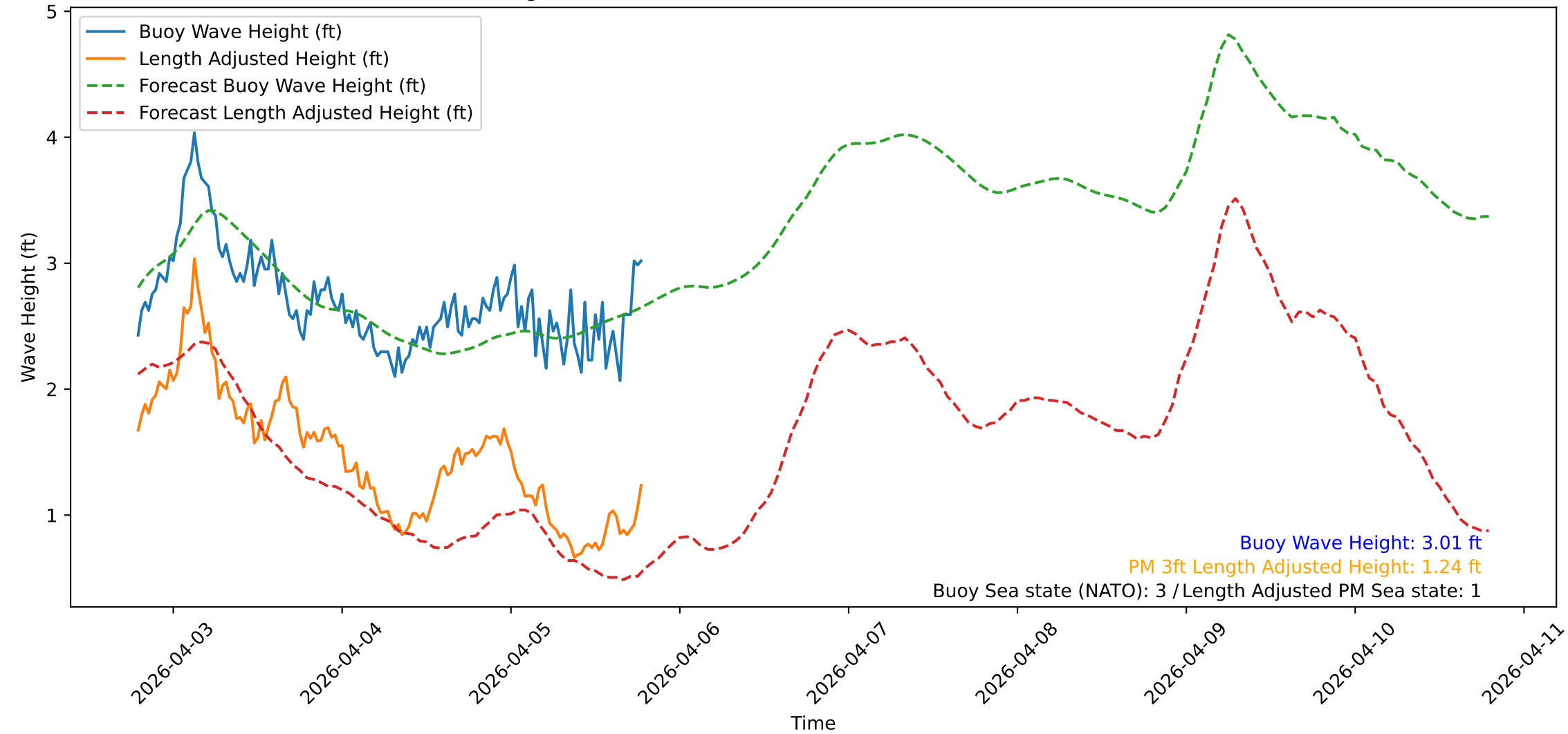
Wave Heights over Time for Oceanside Harbor at 2026-04-05 19:10:33
