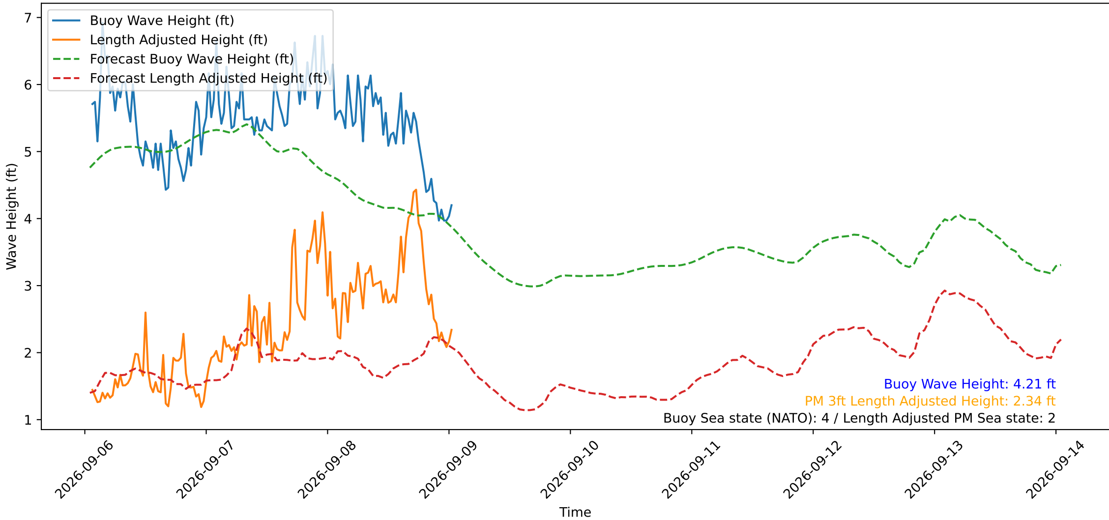
Wave Heights over Time for Red Beach at 2026-09-09 01:20:50
