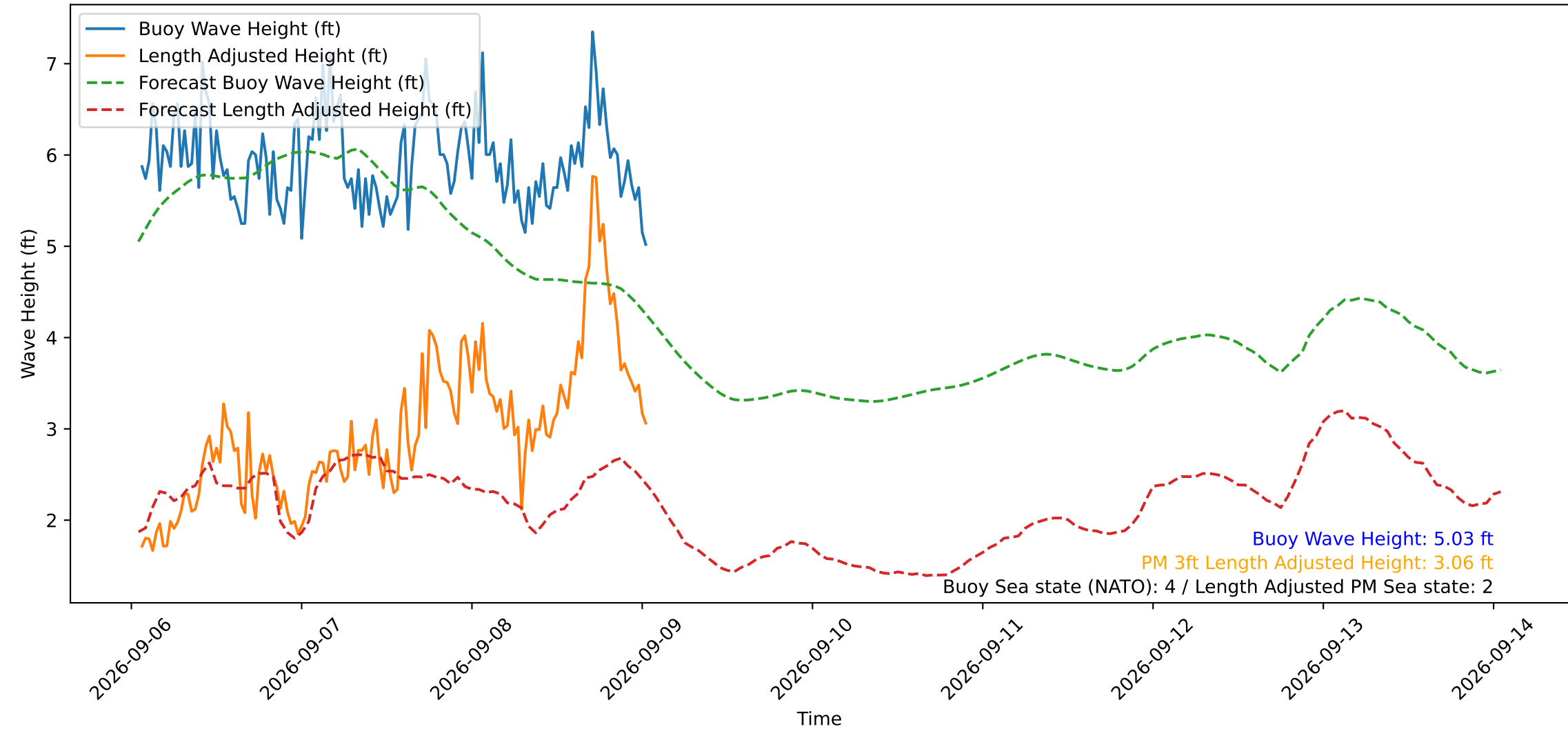
Wave Heights over Time for Oceanside Harbor at 2026-09-09 01:20:29
