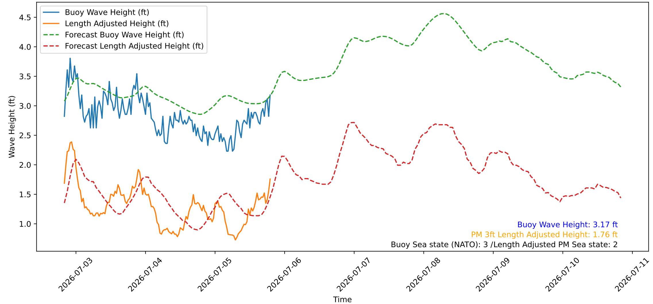
Wave Heights over Time for Red Beach at 2026-07-05 19:40:46
