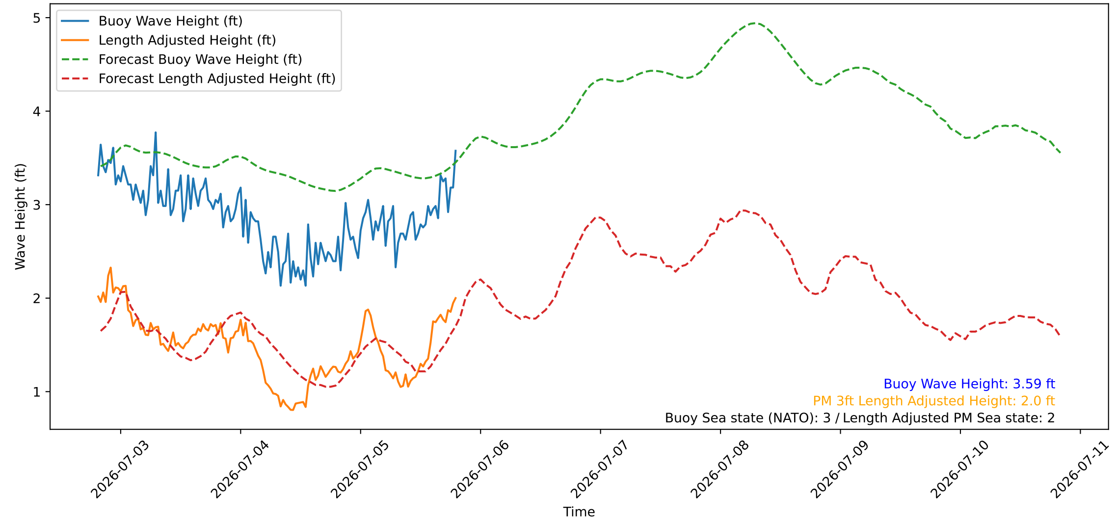
Wave Heights over Time for Oceanside Harbor at 2026-07-05 19:40:27
