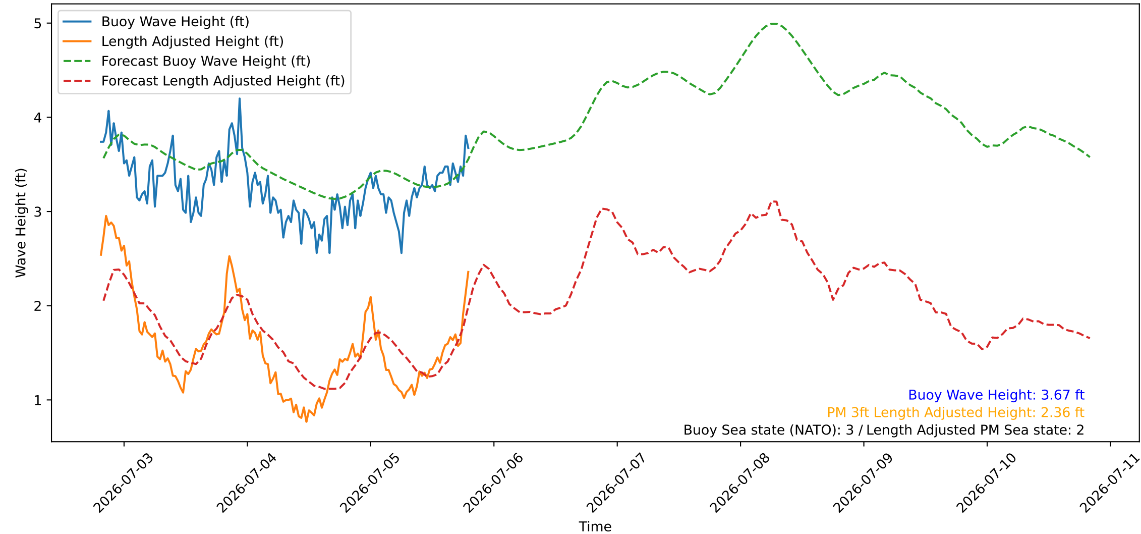
Wave Heights over Time for Green Beach at 2026-07-05 19:41:09
