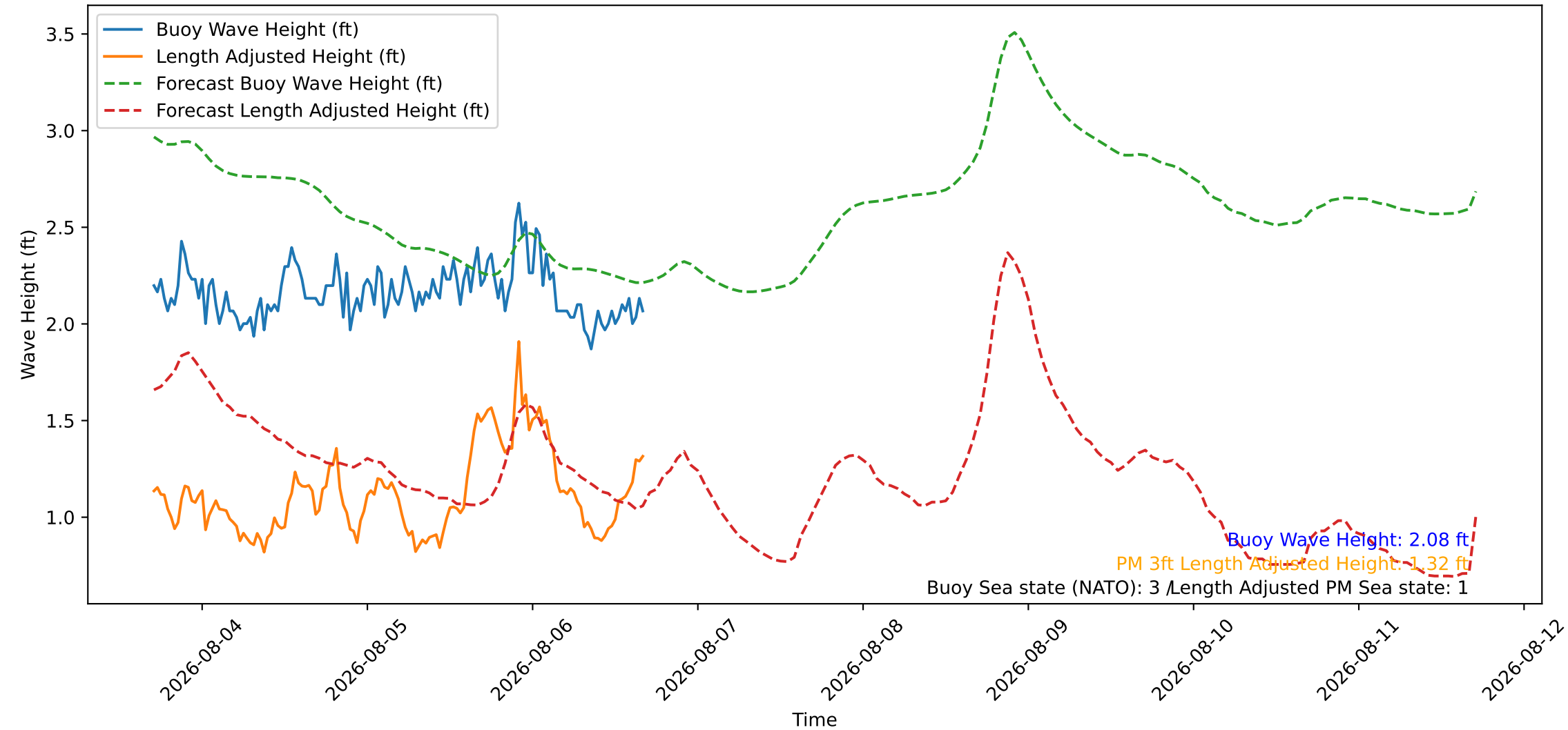
Wave Heights over Time for Green Beach at 2026-08-06 16:51:09
