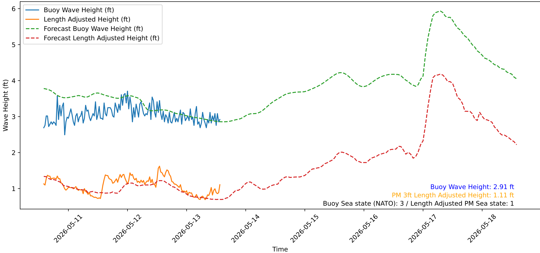
Wave Heights over Time for Oceanside Harbor at 2026-05-13 14:10:31
