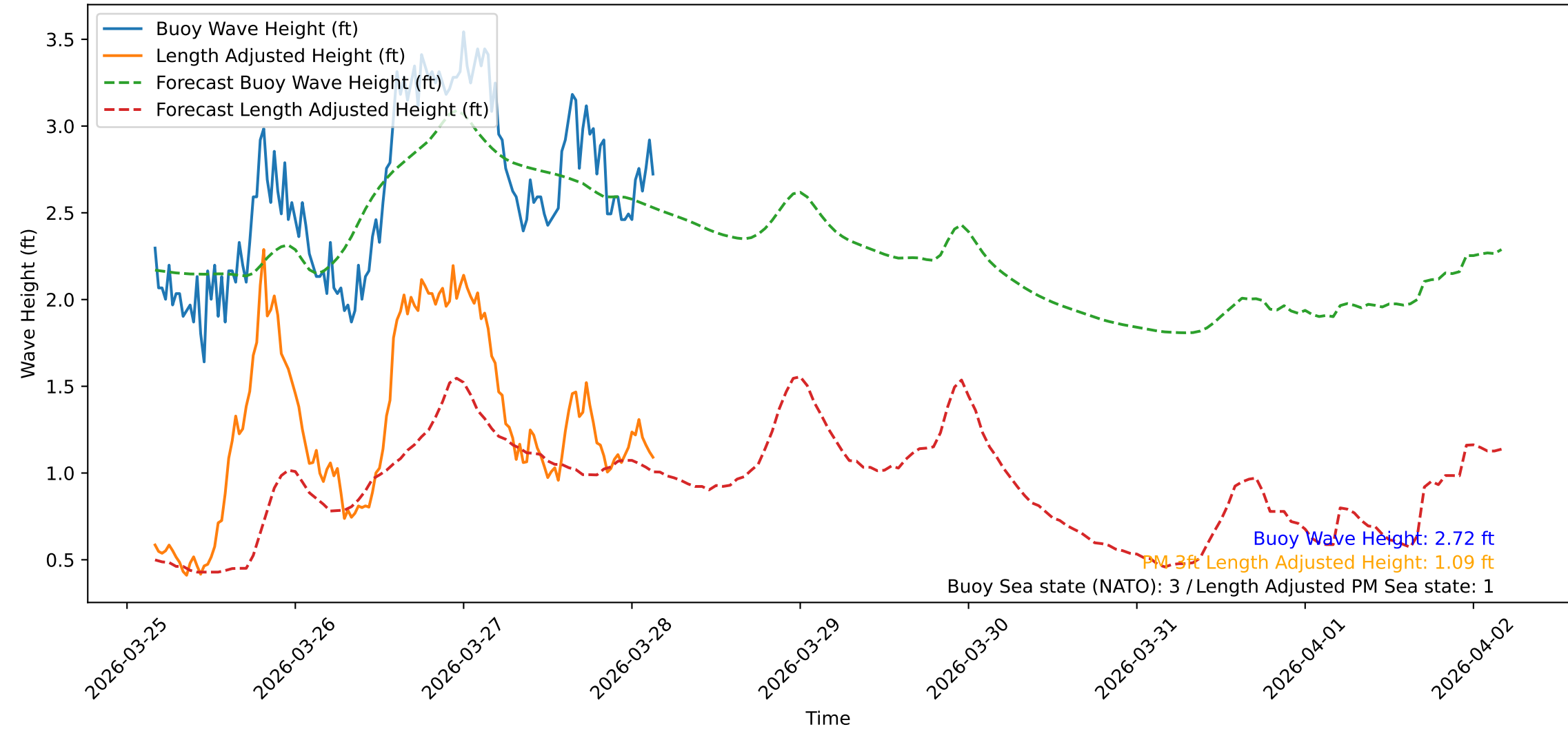
Wave Heights over Time for Green Beach at 2026-03-28 03:51:09
