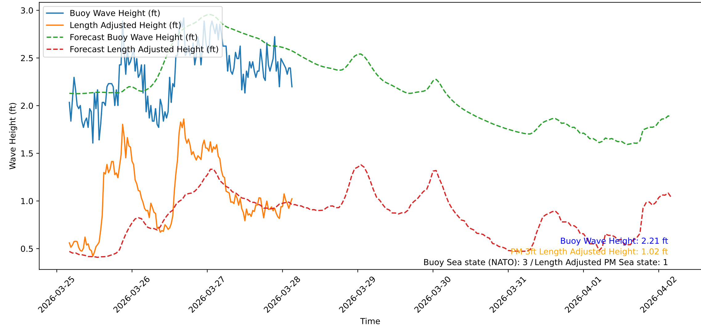
Wave Heights over Time for Oceanside Harbor at 2026-03-28 03:50:31
