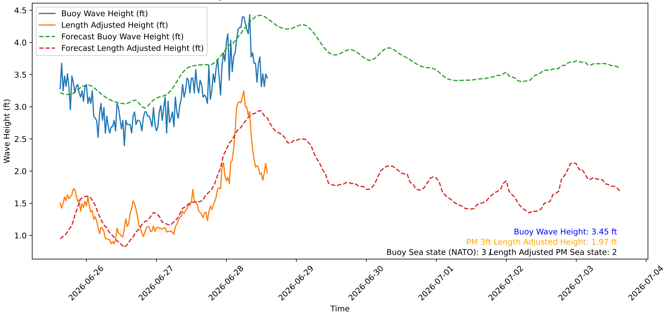
Wave Heights over Time for Oceanside Harbor at 2026-06-28 14:50:26
