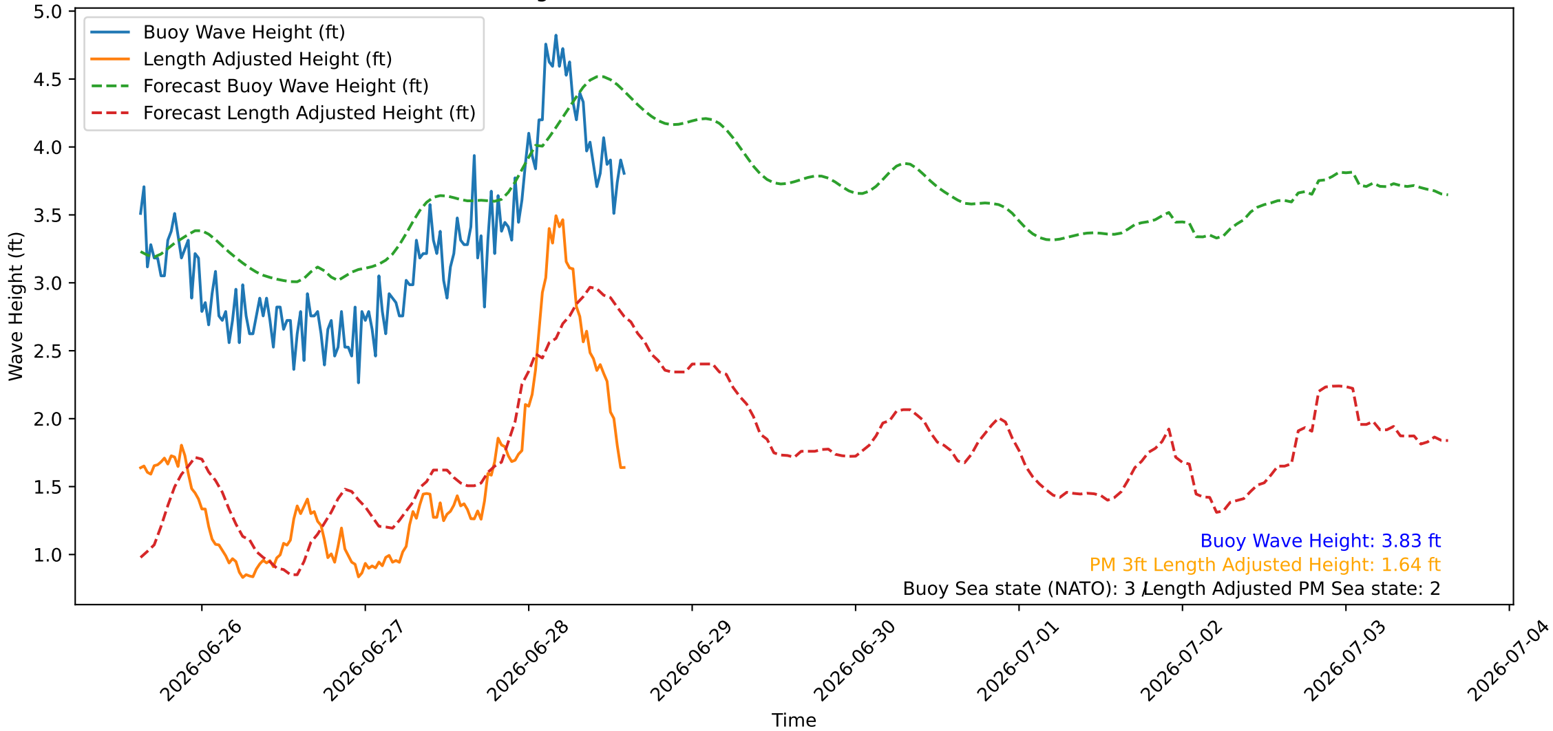
Wave Heights over Time for Green Beach at 2026-06-28 14:51:09
