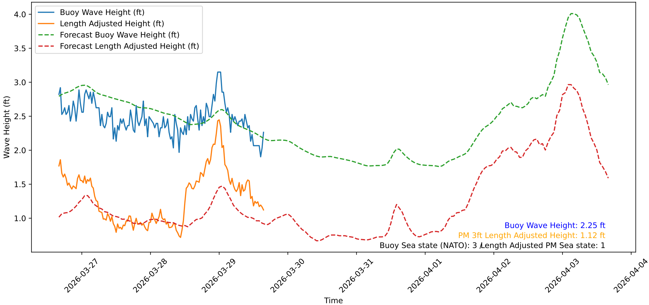
Wave Heights over Time for Oceanside Harbor at 2026-03-29 16:00:31
