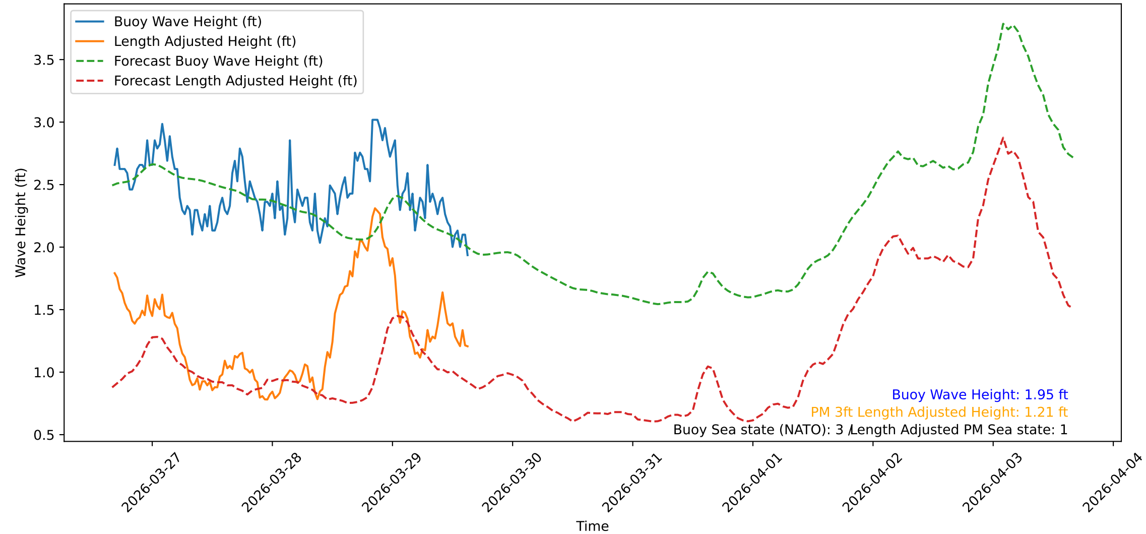
Wave Heights over Time for Red Beach at 2026-03-29 16:00:46
