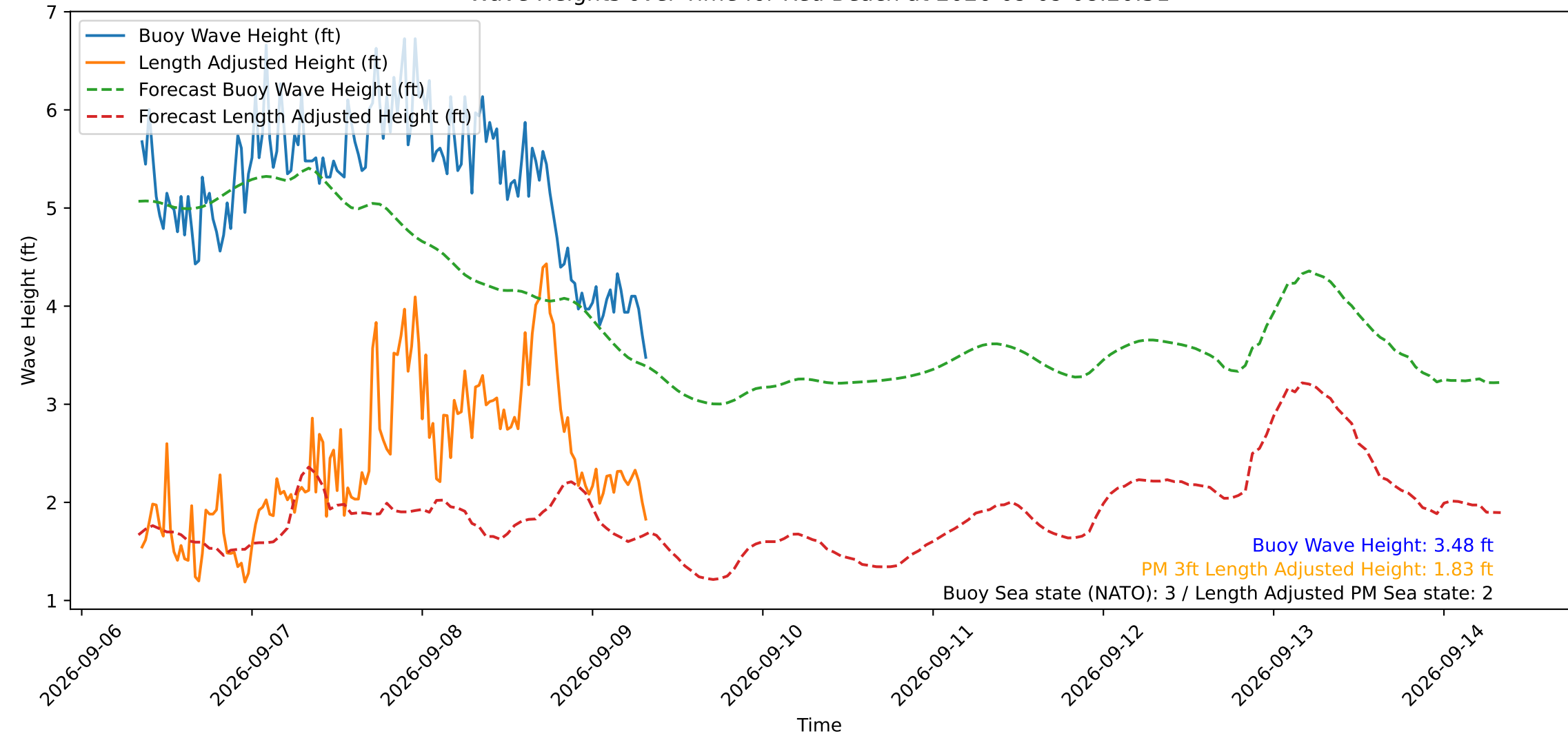
Wave Heights over Time for Red Beach at 2026-09-09 08:20:51
