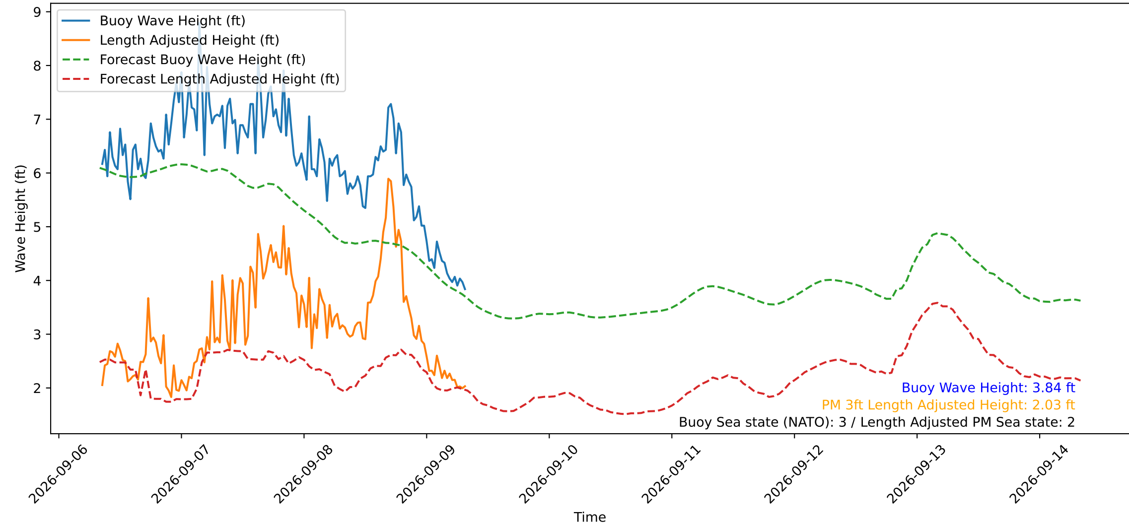
Wave Heights over Time for Green Beach at 2026-09-09 08:21:15
