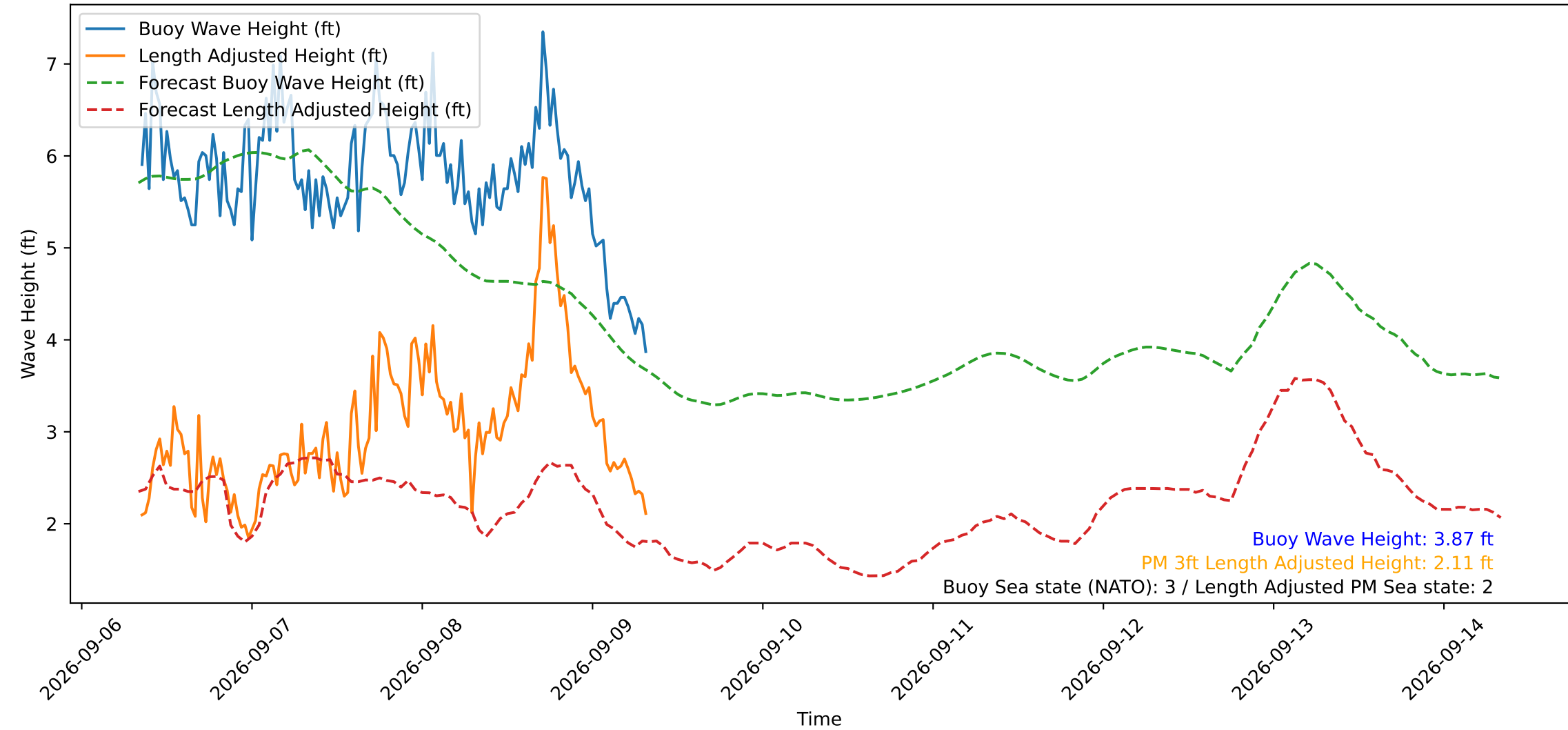
Wave Heights over Time for Oceanside Harbor at 2026-09-09 08:20:30
