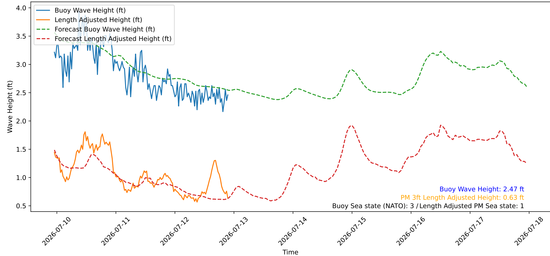
Wave Heights over Time for Red Beach at 2026-07-12 22:40:45
