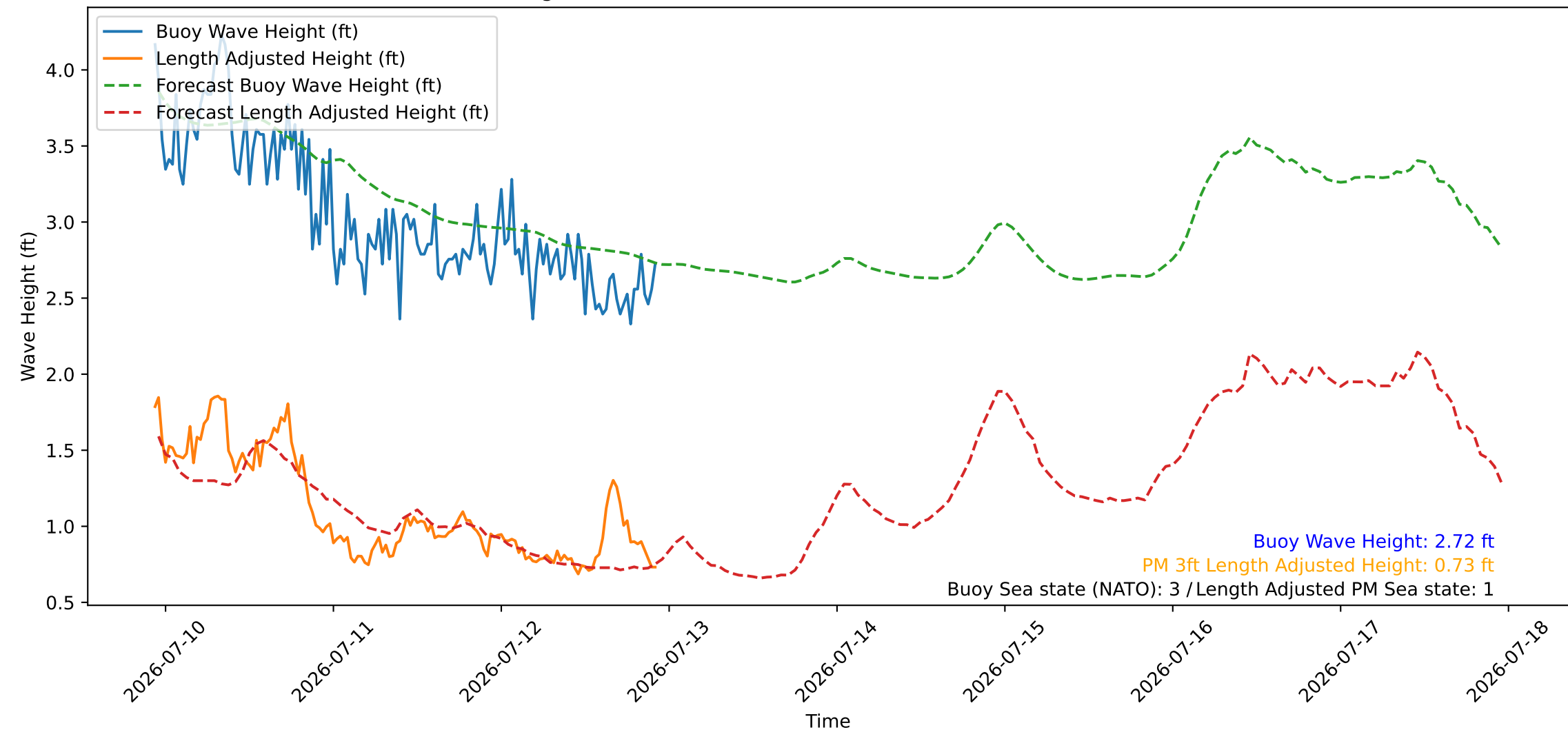
Wave Heights over Time for Oceanside Harbor at 2026-07-12 22:40:26
