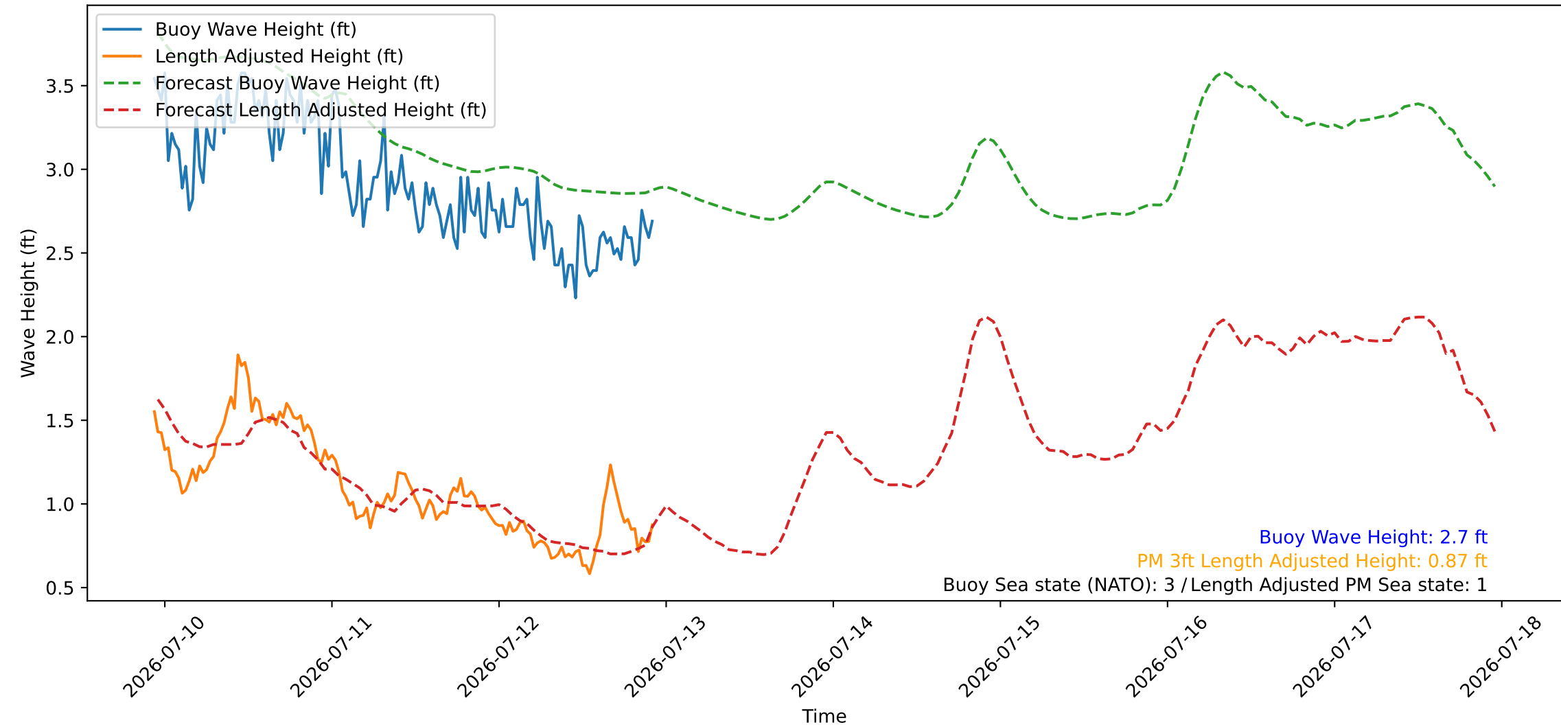
Wave Heights over Time for Green Beach at 2026-07-12 22:41:08
