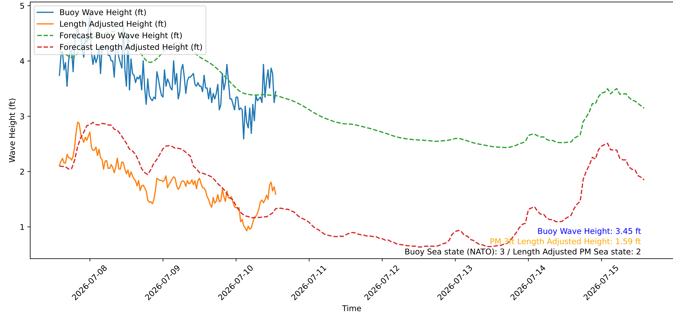
Wave Heights over Time for Red Beach at 2026-07-10 13:50:48
