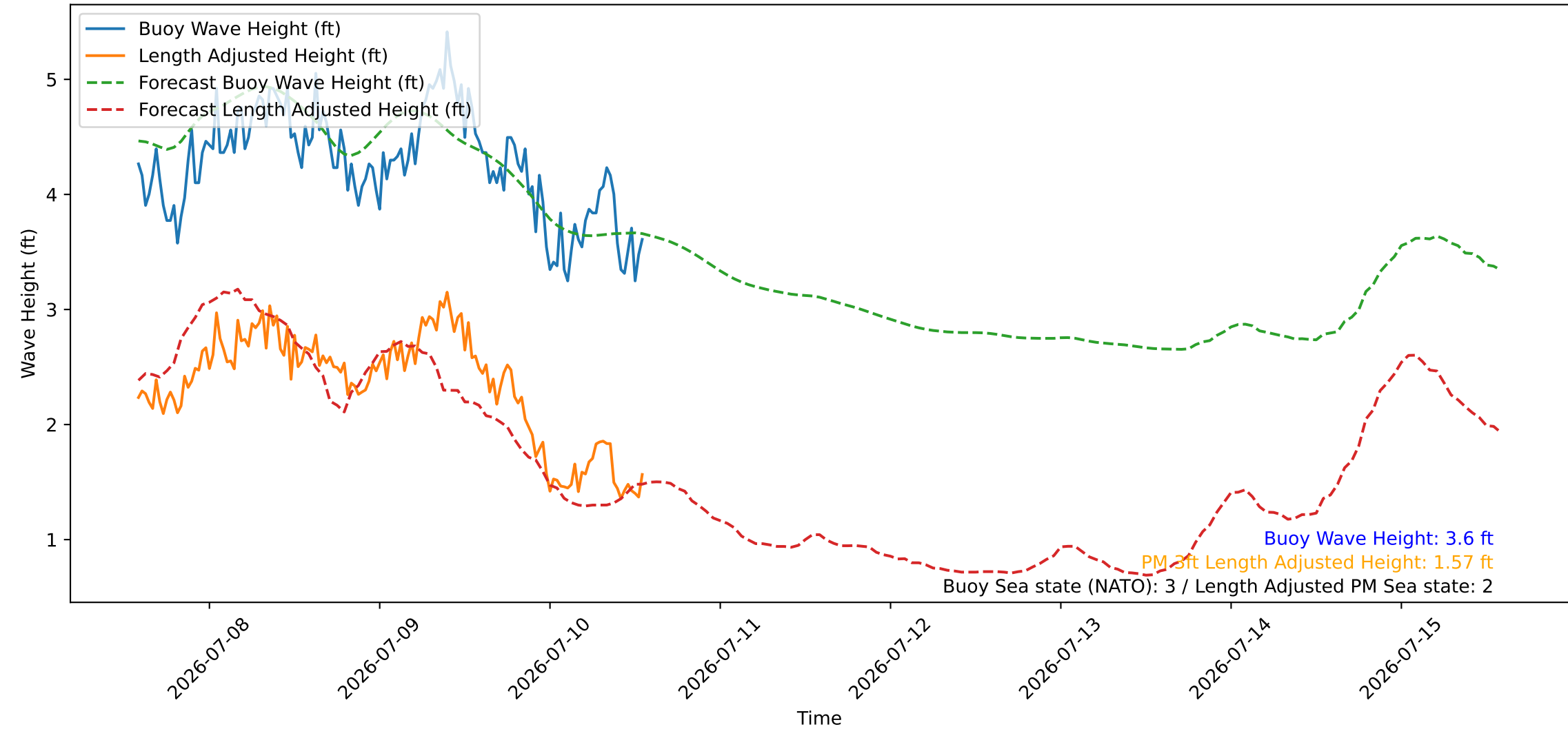
Wave Heights over Time for Oceanside Harbor at 2026-07-10 13:50:26
