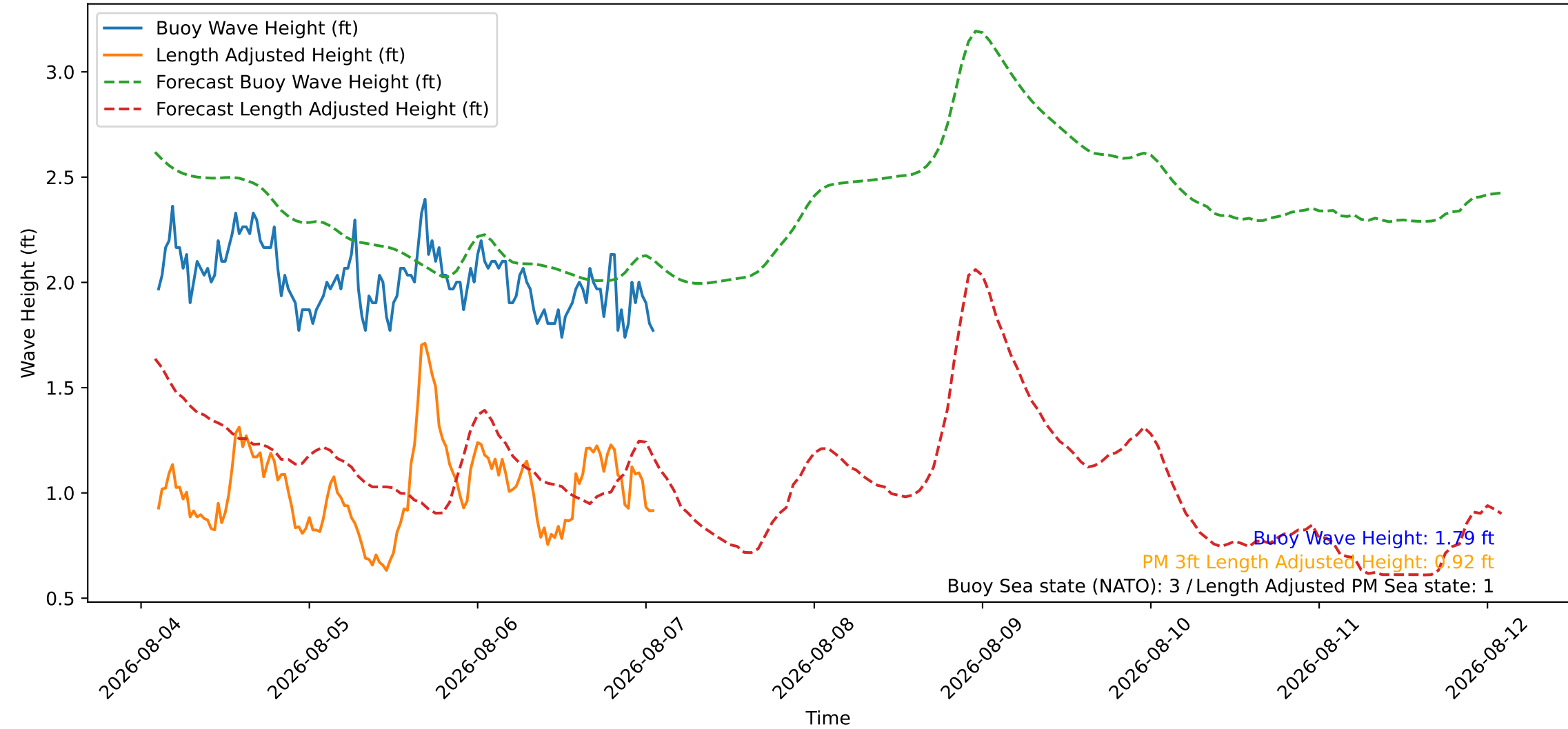
Wave Heights over Time for Red Beach at 2026-08-07 02:00:45
