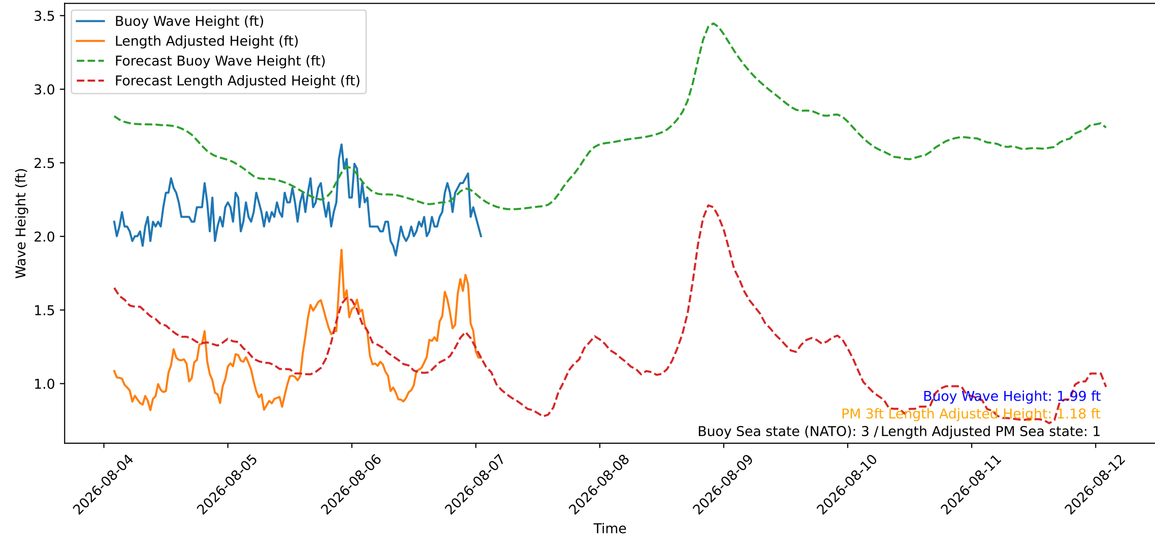
Wave Heights over Time for Green Beach at 2026-08-07 02:01:07
