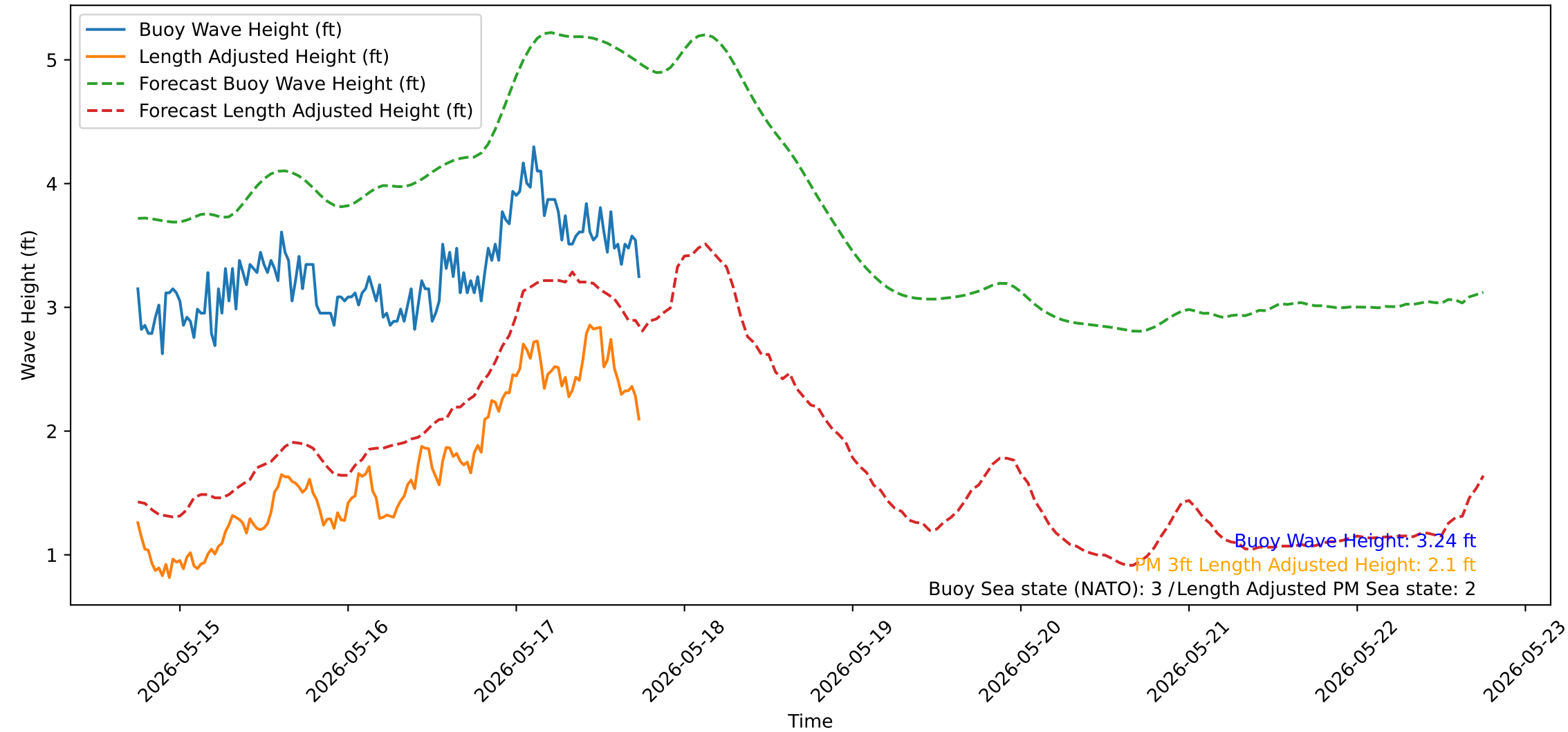
Wave Heights over Time for Oceanside Harbor at 2026-05-17 18:10:32
