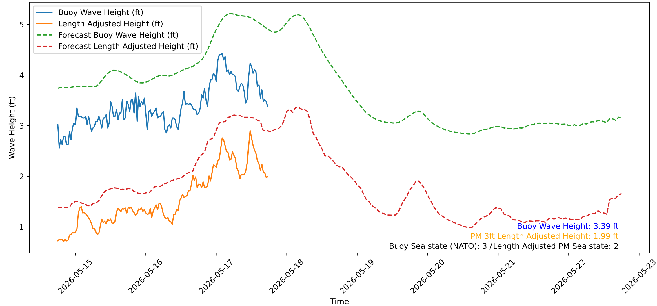
Wave Heights over Time for Green Beach at 2026-05-17 18:11:14
