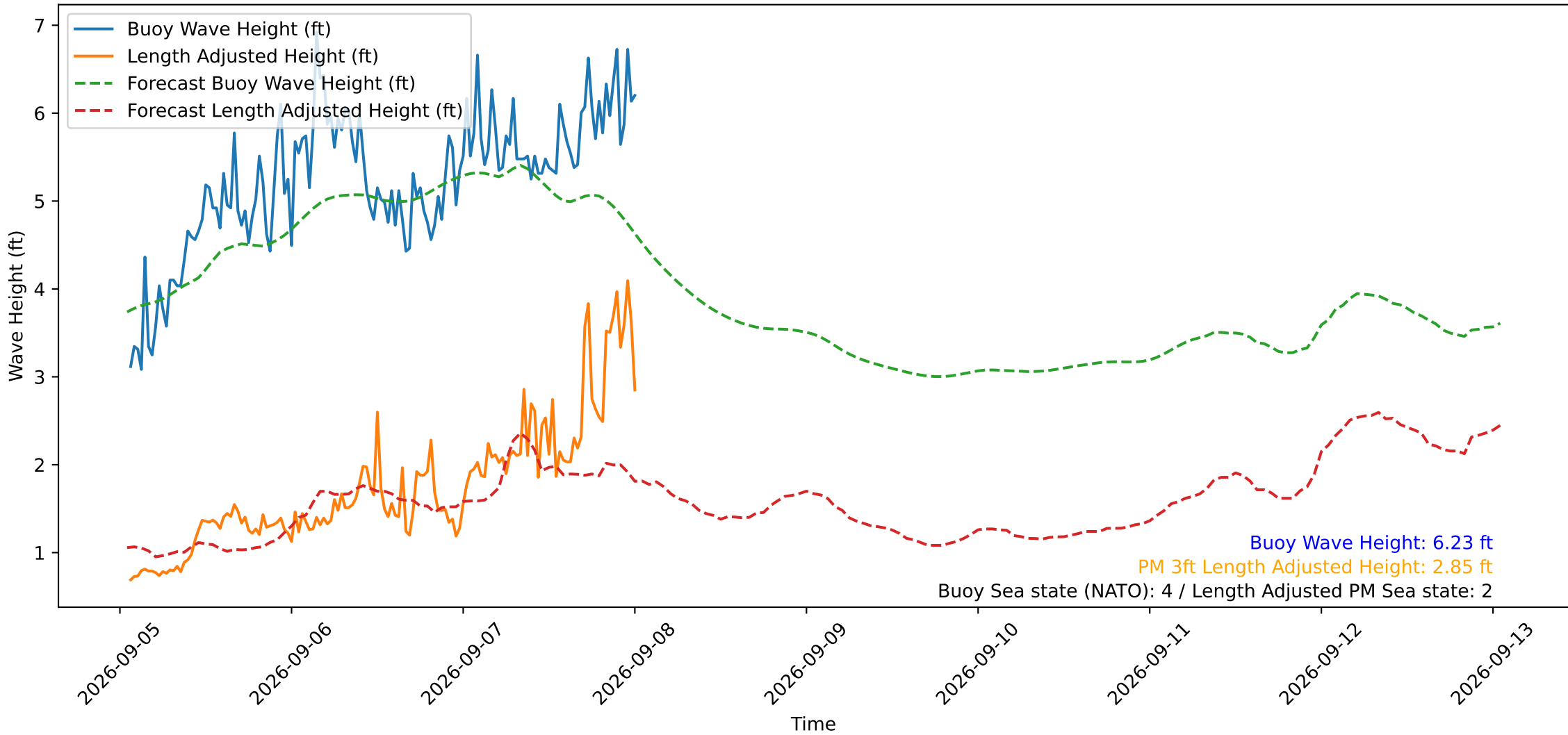
Wave Heights over Time for Red Beach at 2026-09-08 01:00:49
