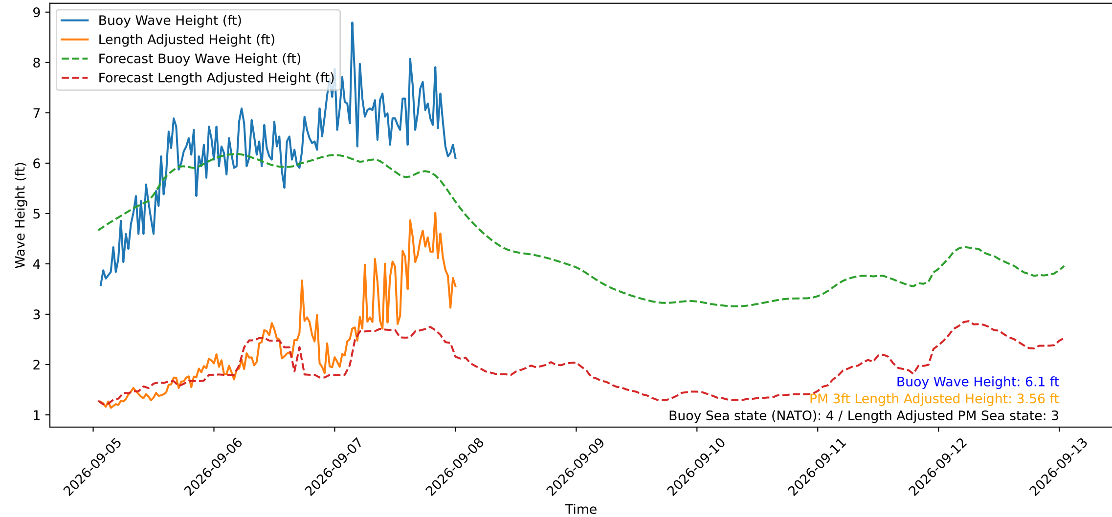
Wave Heights over Time for Green Beach at 2026-09-08 01:01:11
