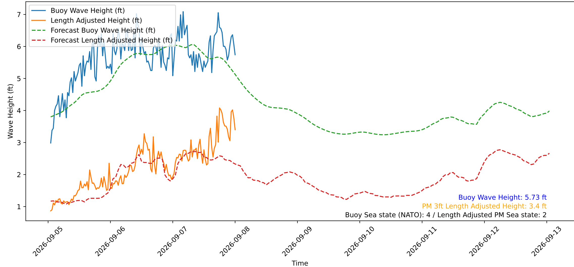
Wave Heights over Time for Oceanside Harbor at 2026-09-08 01:00:29
