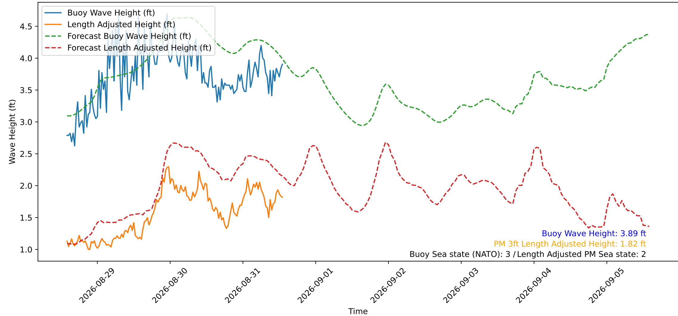
Wave Heights over Time for Red Beach at 2026-08-31 13:50:49
