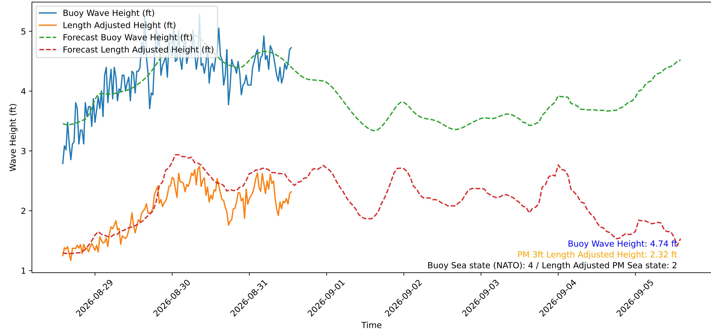
Wave Heights over Time for Oceanside Harbor at 2026-08-31 13:50:29
