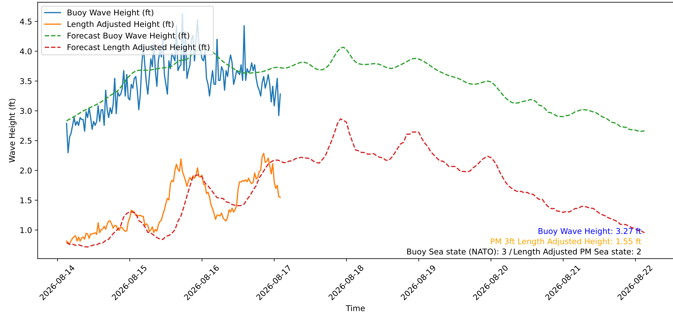
Wave Heights over Time for Oceanside Harbor at 2026-08-17 02:50:26
