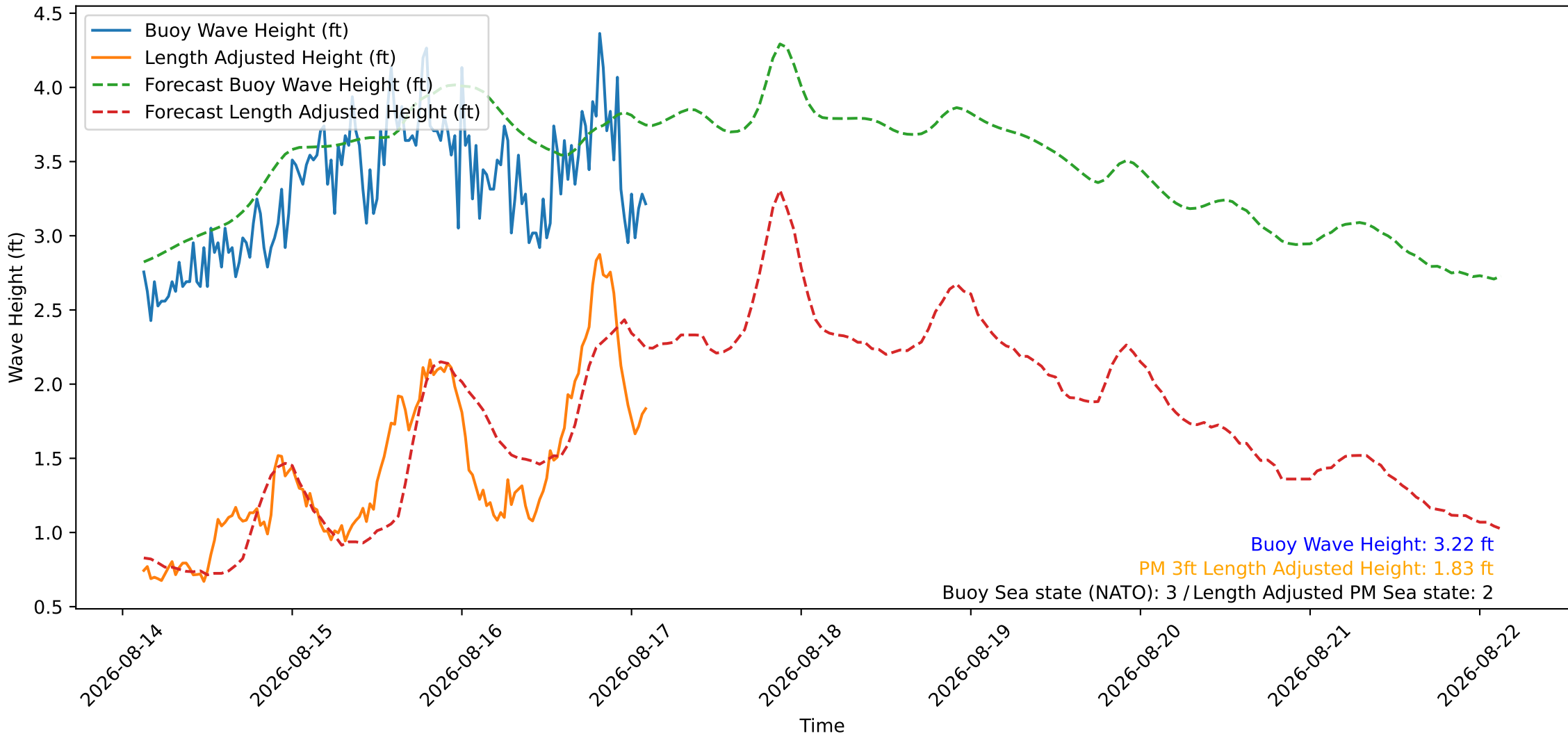
Wave Heights over Time for Green Beach at 2026-08-17 02:51:11
