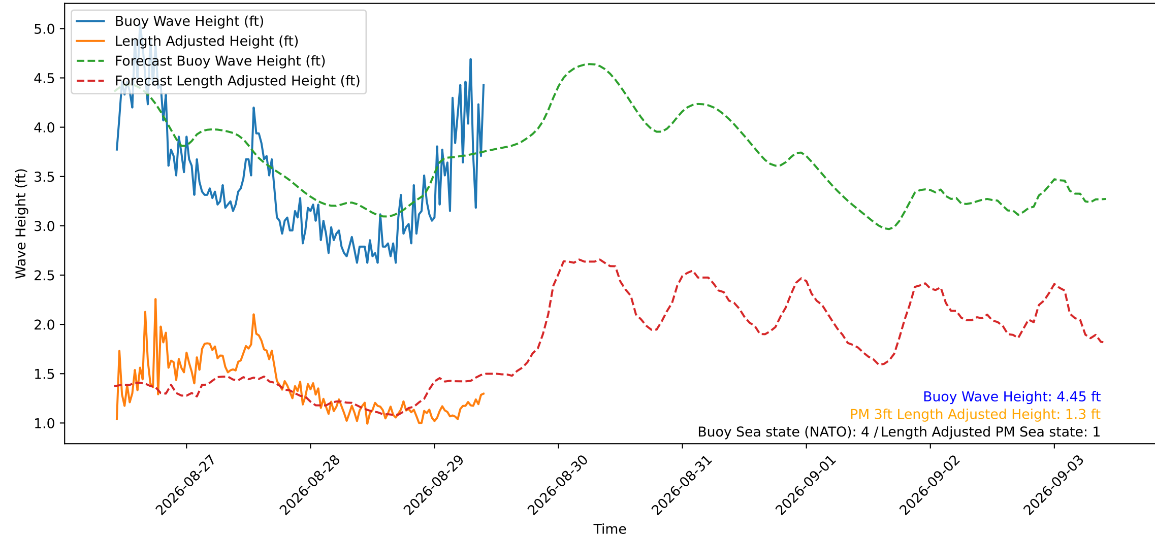
Wave Heights over Time for Red Beach at 2026-08-29 10:10:48
