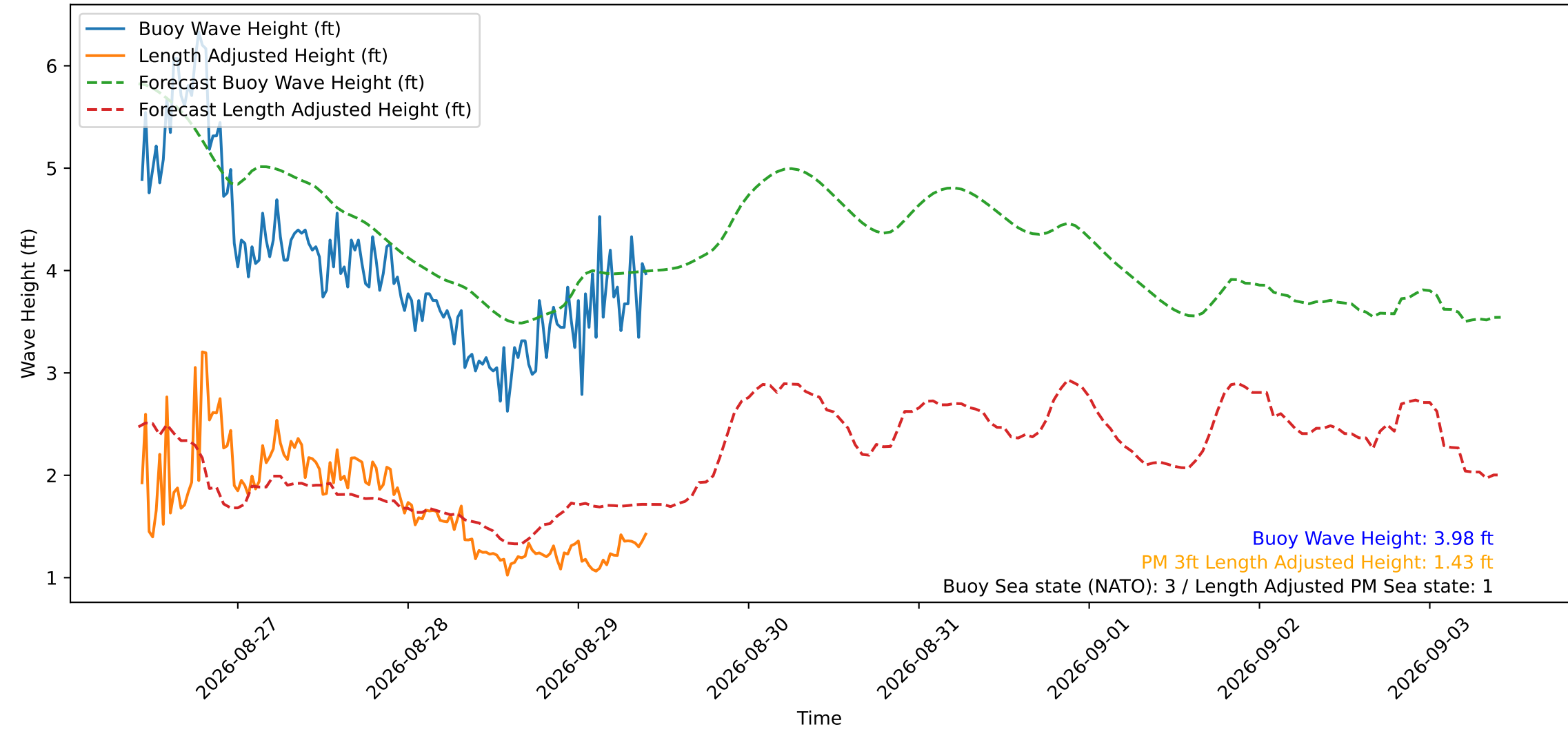
Wave Heights over Time for Green Beach at 2026-08-29 10:11:10
