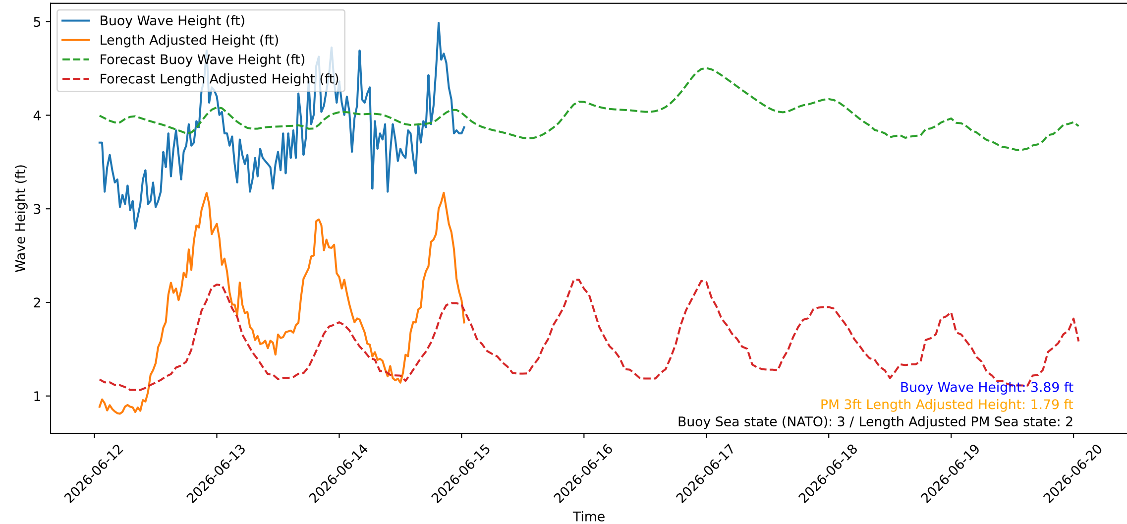
Wave Heights over Time for Oceanside Harbor at 2026-06-15 01:10:26
