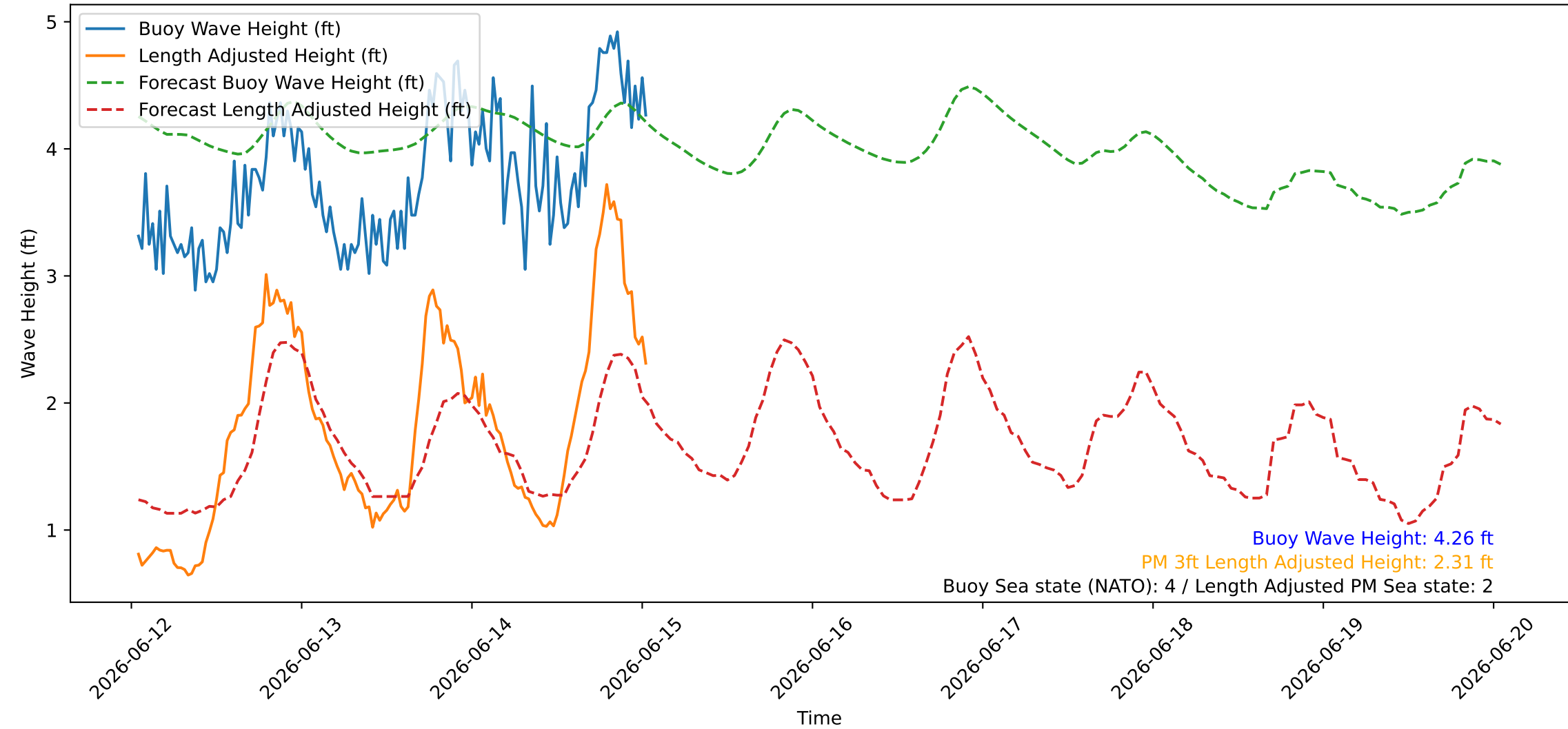
Wave Heights over Time for Green Beach at 2026-06-15 01:11:08
