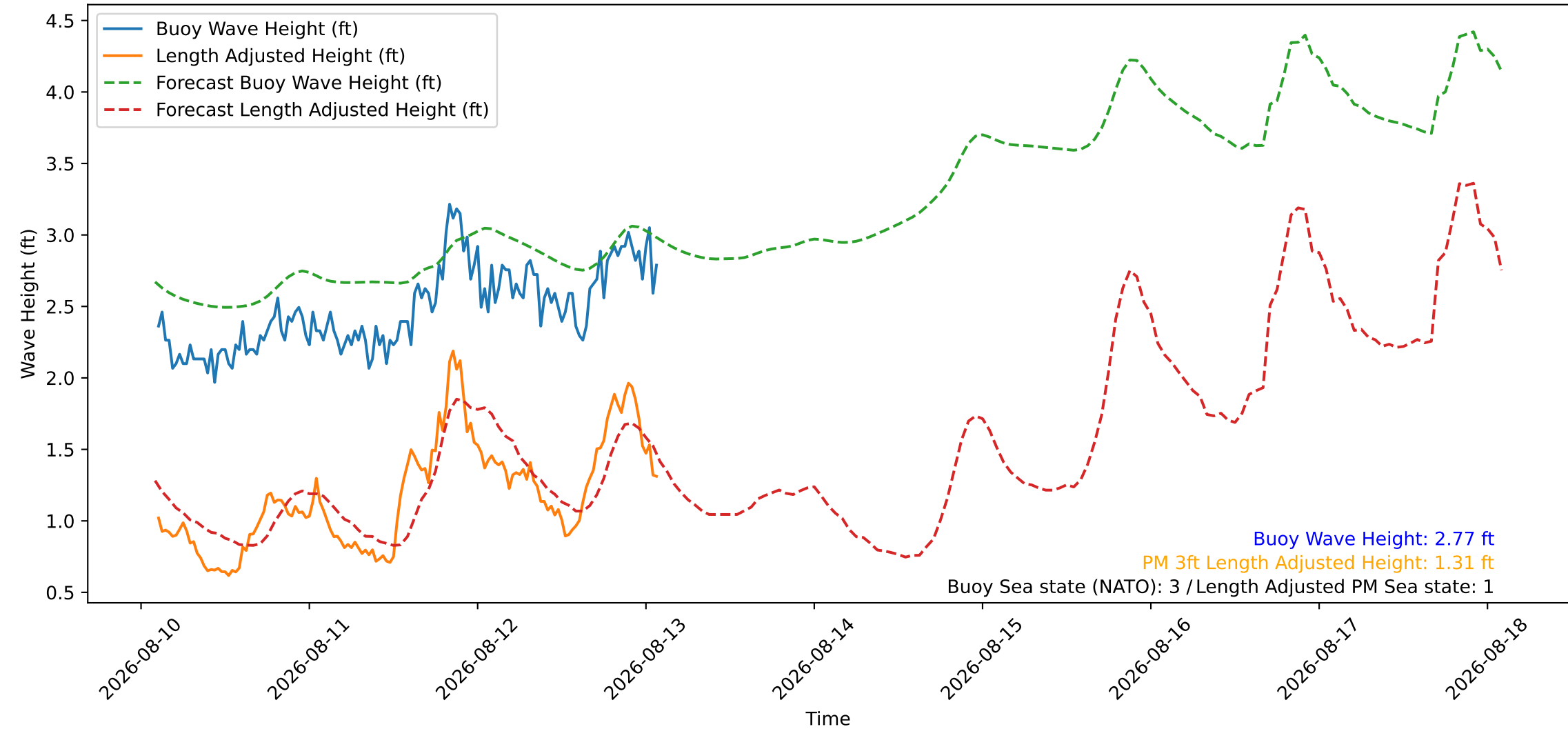
Wave Heights over Time for Green Beach at 2026-08-13 02:21:08
