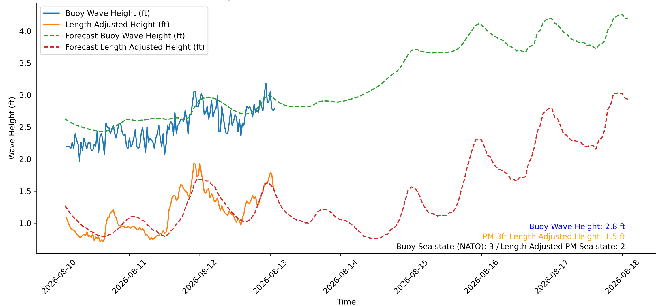
Wave Heights over Time for Oceanside Harbor at 2026-08-13 02:20:26
