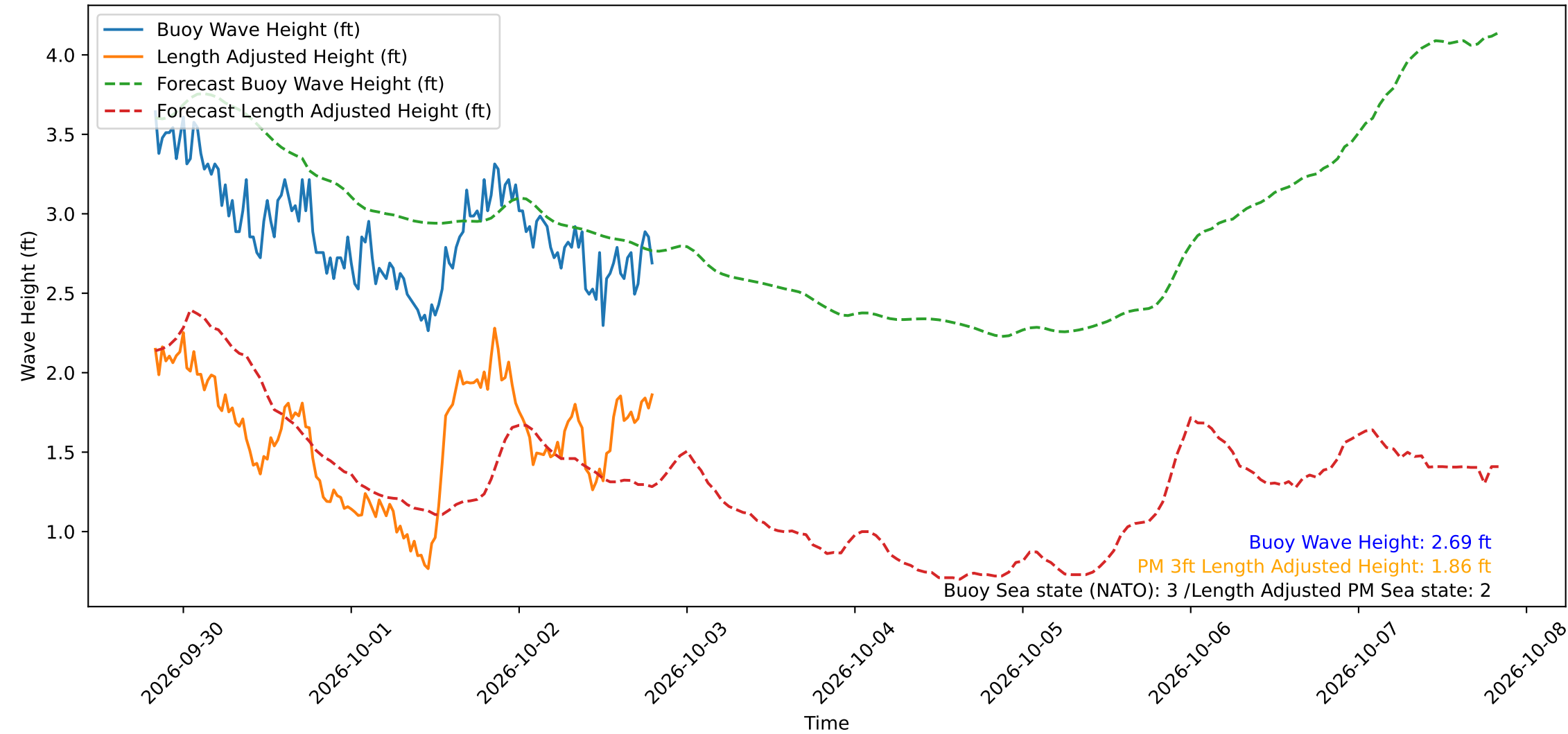
Wave Heights over Time for Oceanside Harbor at 2026-10-02 19:50:29
