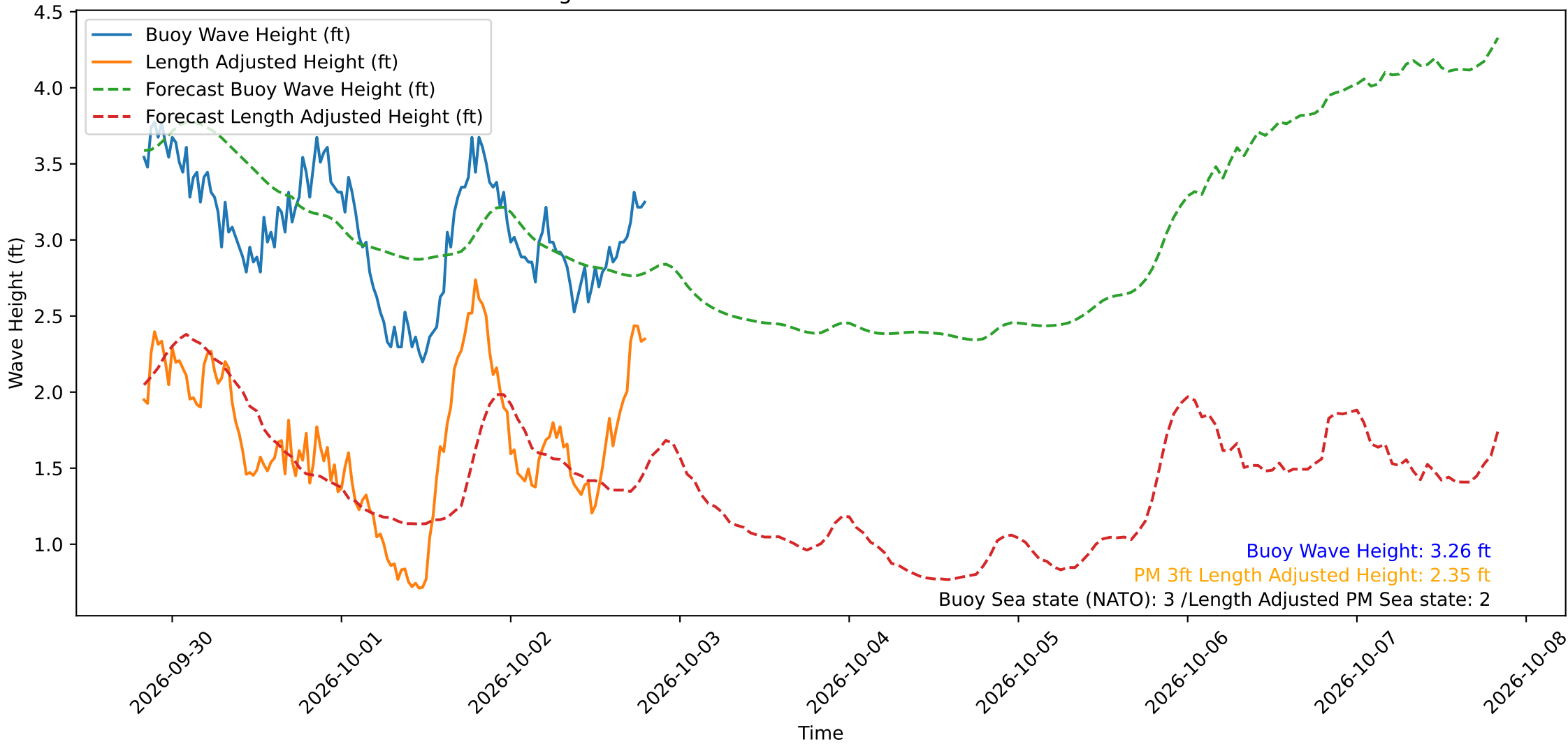
Wave Heights over Time for Green Beach at 2026-10-02 19:51:13
