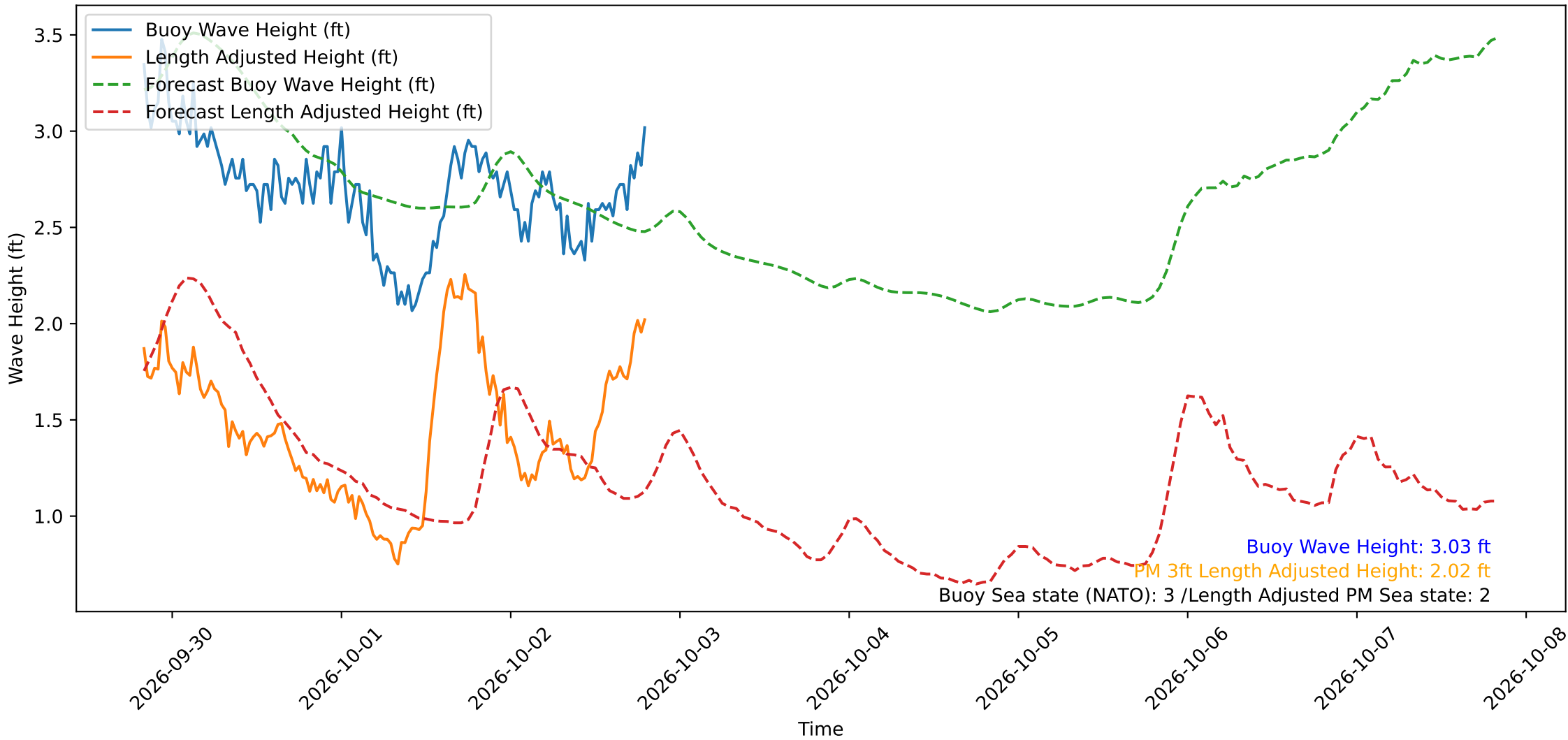
Wave Heights over Time for Red Beach at 2026-10-02 19:50:50
