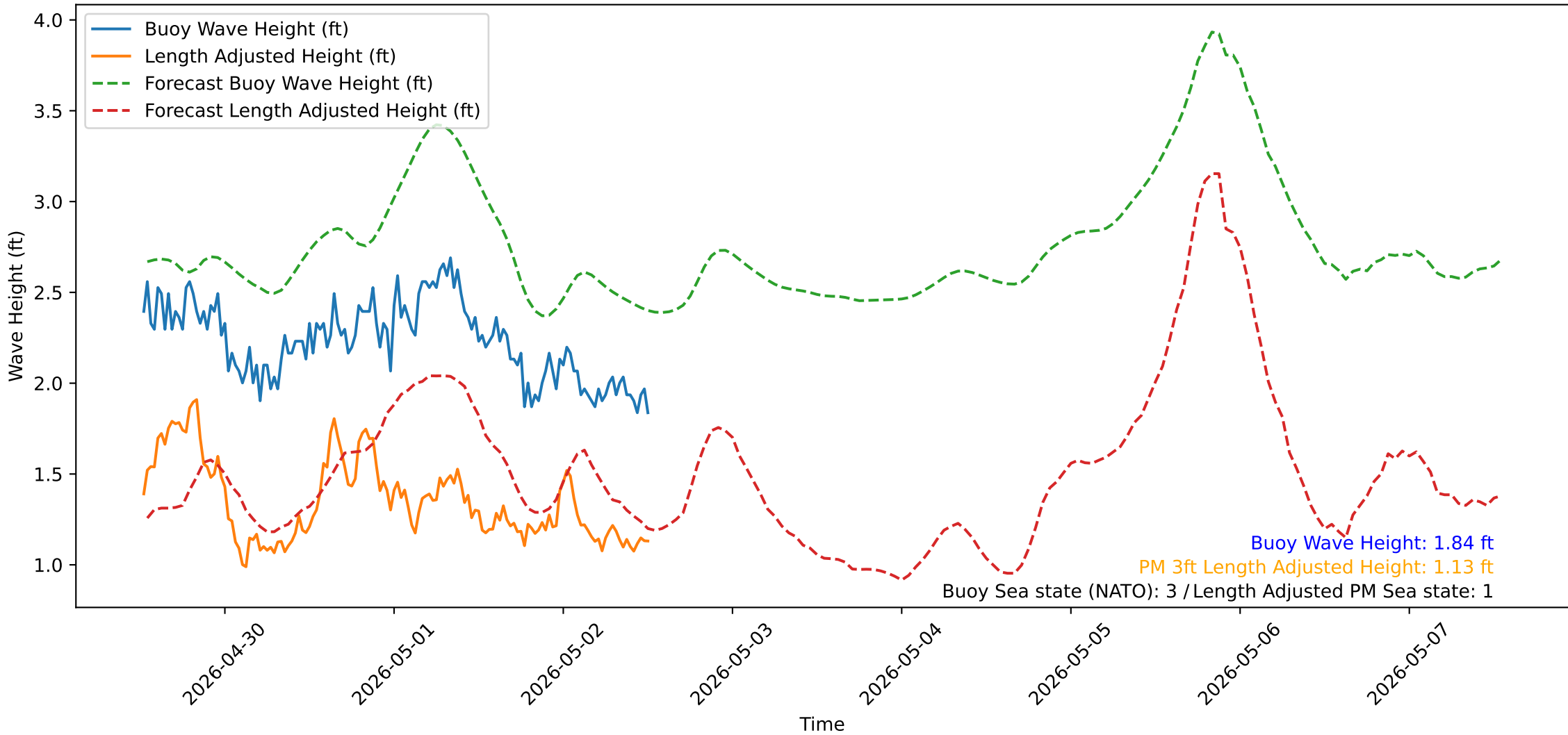
Wave Heights over Time for Oceanside Harbor at 2026-05-02 12:30:32
