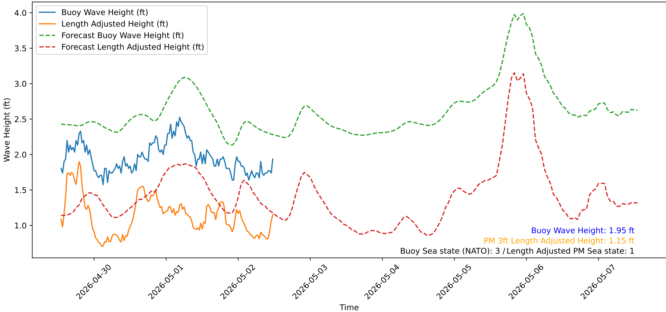
Wave Heights over Time for Red Beach at 2026-05-02 12:30:50
