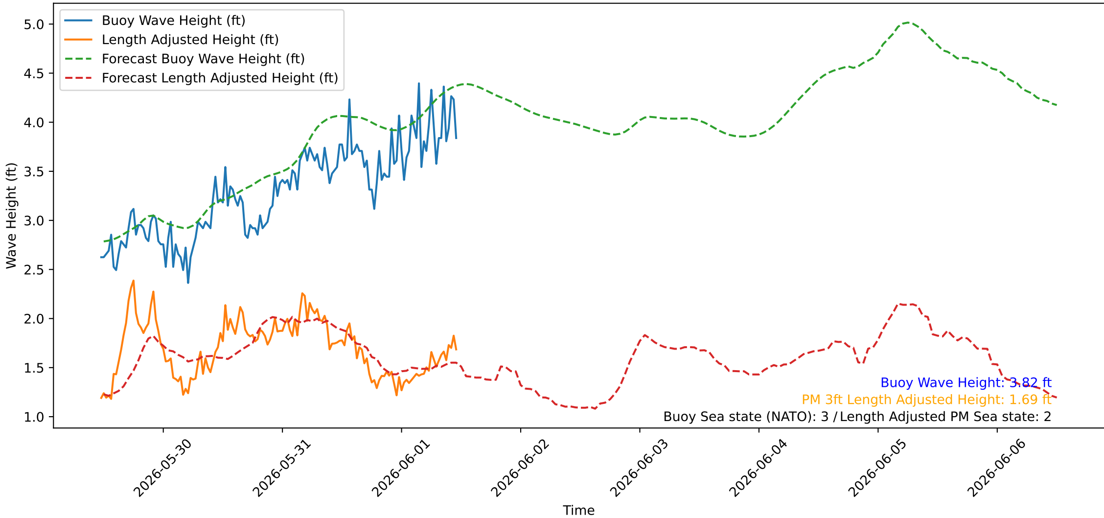
Wave Heights over Time for Oceanside Harbor at 2026-06-01 11:30:26
