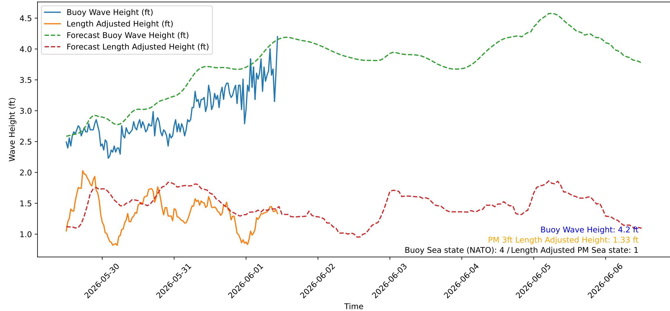
Wave Heights over Time for Red Beach at 2026-06-01 11:30:46
