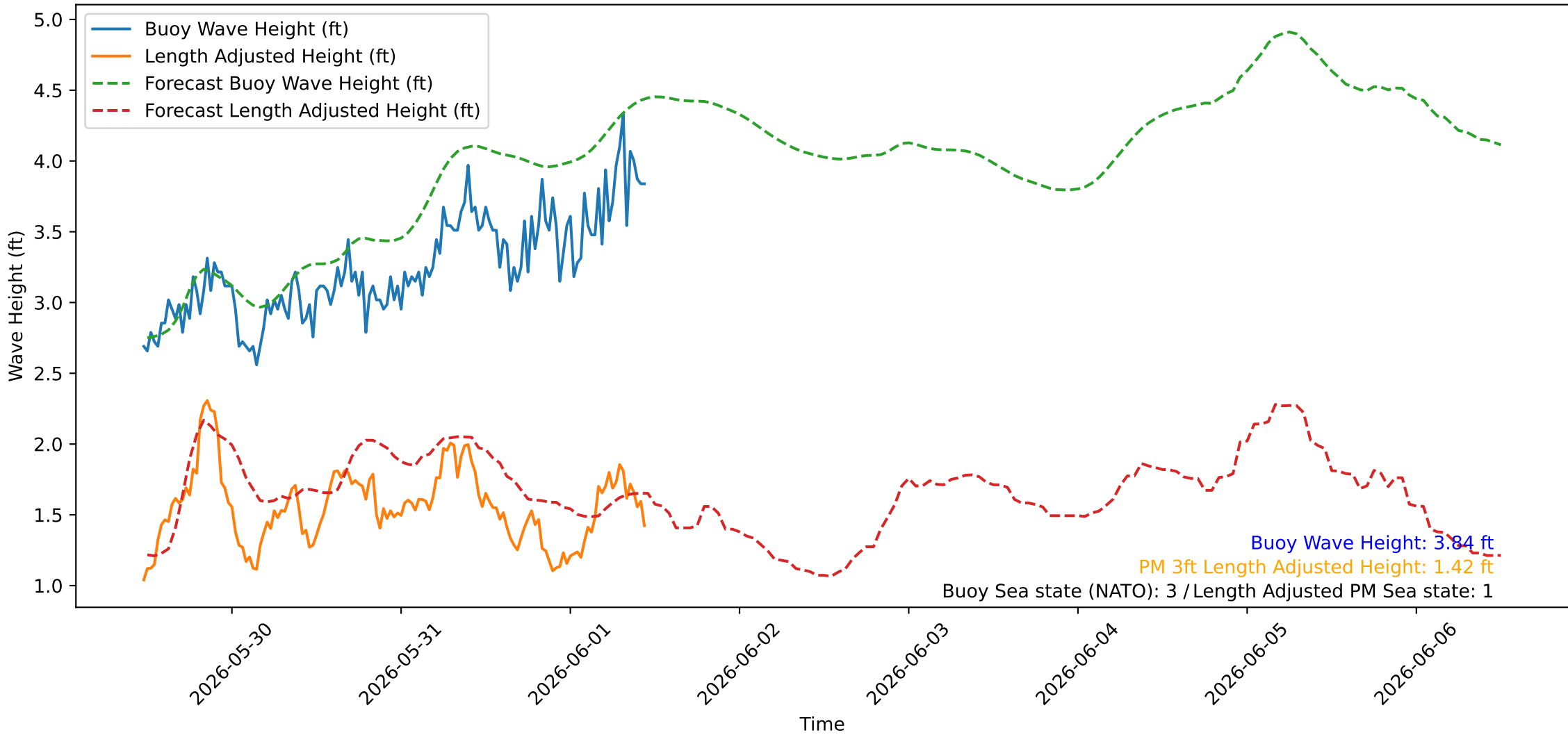
Wave Heights over Time for Green Beach at 2026-06-01 11:31:09
