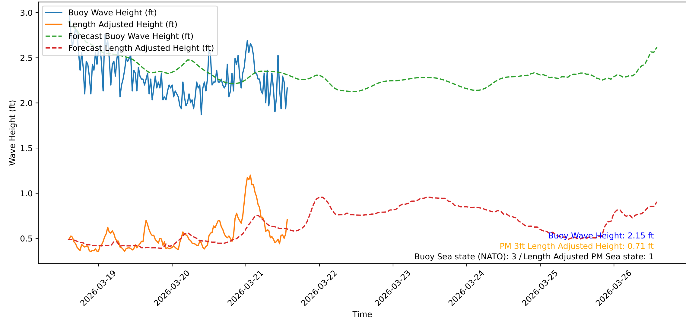
Wave Heights over Time for Red Beach at 2026-03-21 14:20:48
