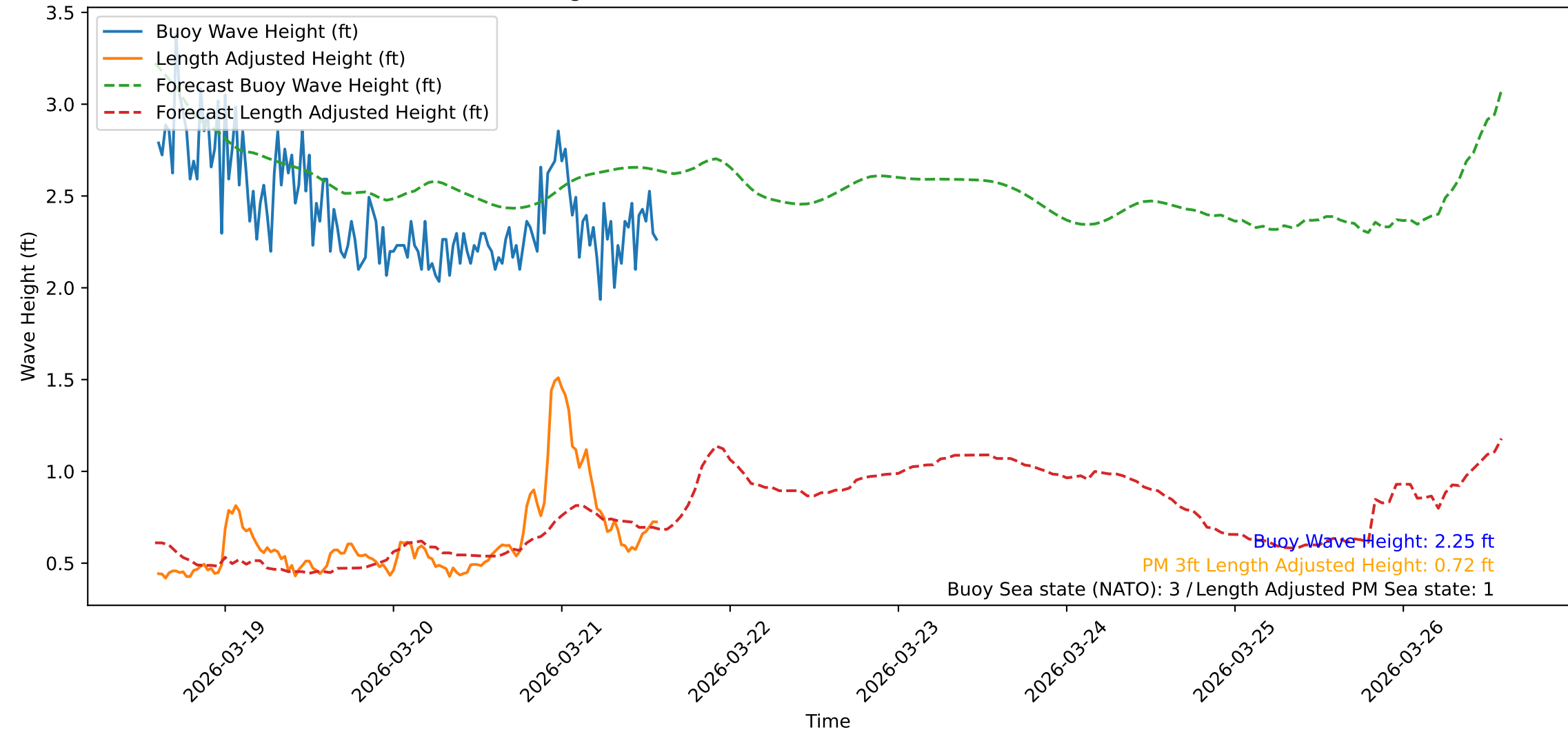
Wave Heights over Time for Green Beach at 2026-03-21 14:21:11
