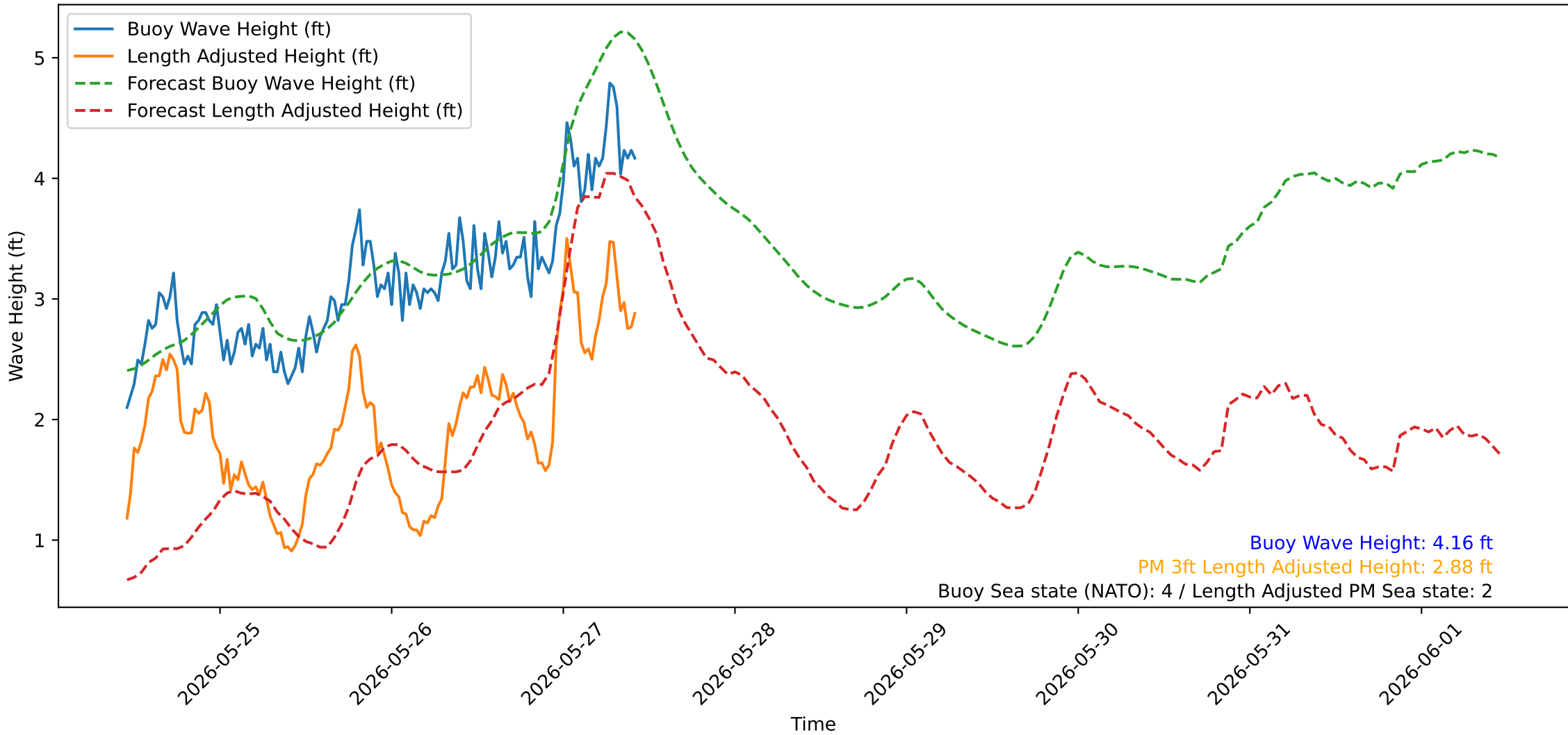
Wave Heights over Time for Red Beach at 2026-05-27 10:50:47
