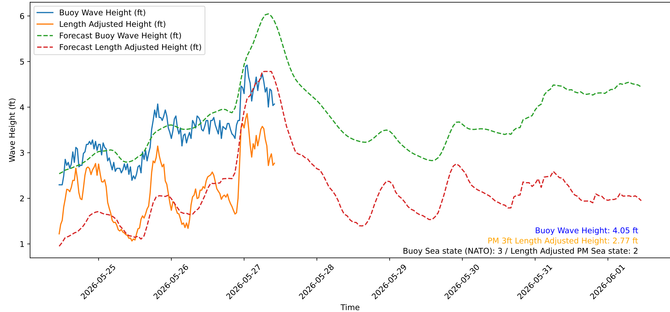
Wave Heights over Time for Green Beach at 2026-05-27 10:51:09
