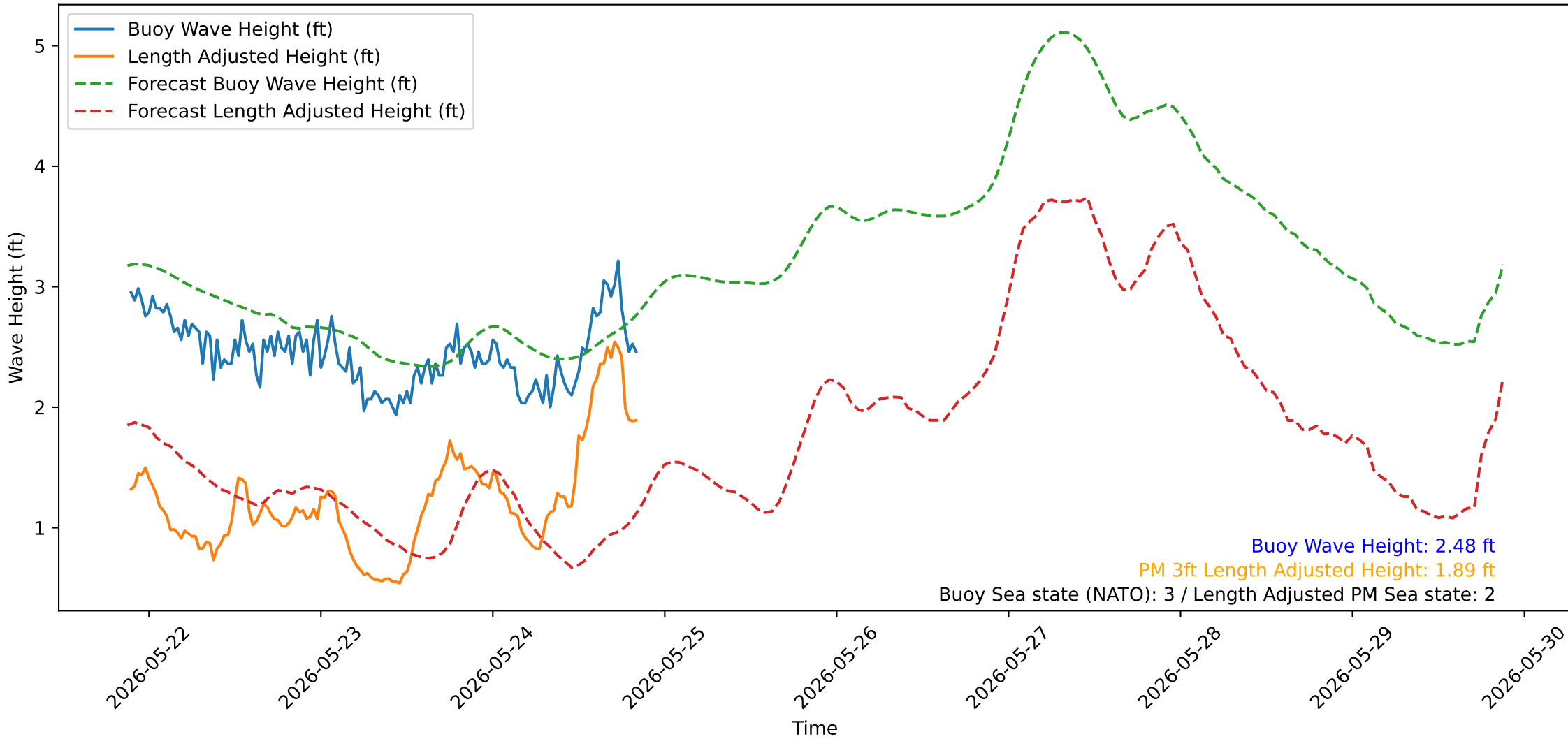
Wave Heights over Time for Red Beach at 2026-05-24 21:00:51
