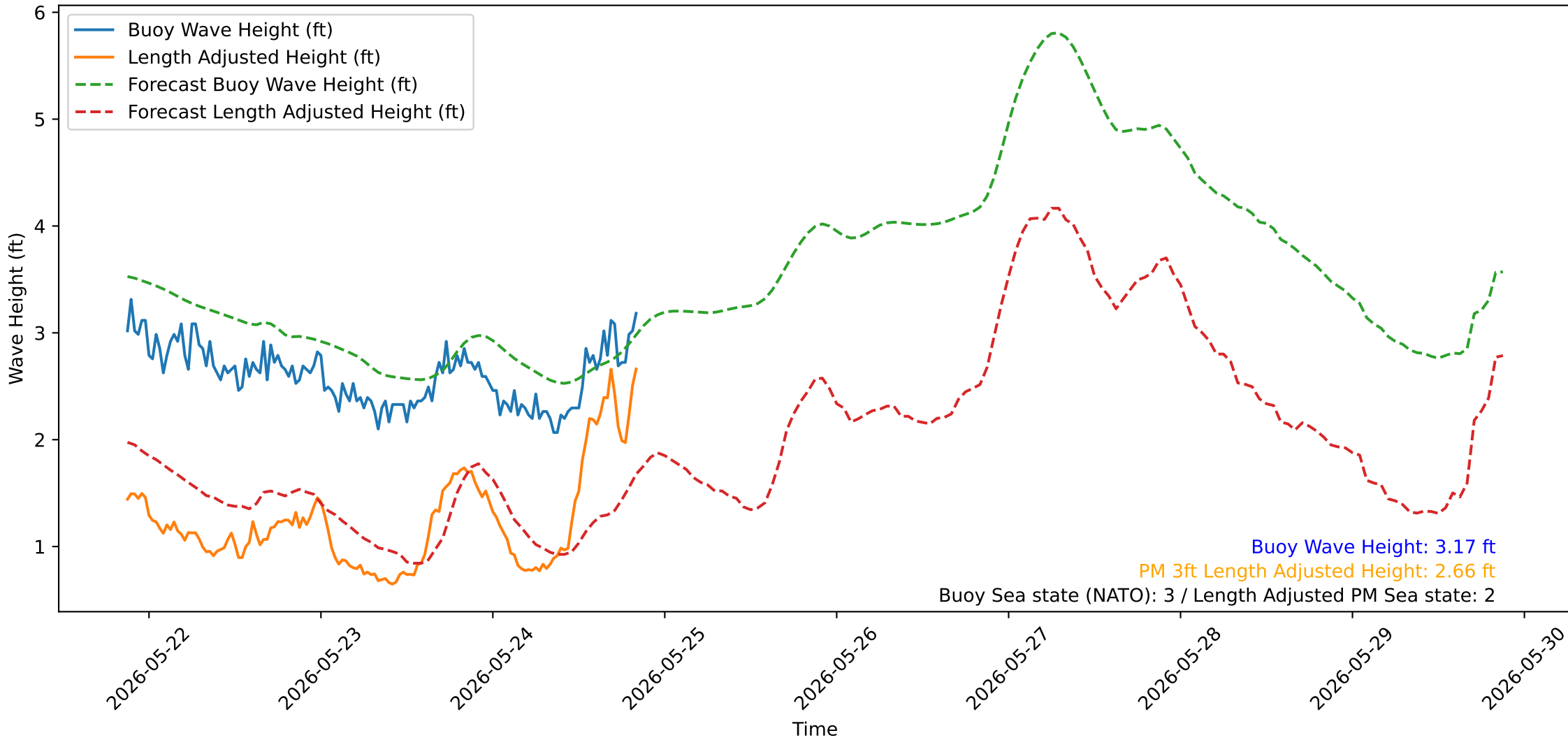
Wave Heights over Time for Green Beach at 2026-05-24 21:01:14
