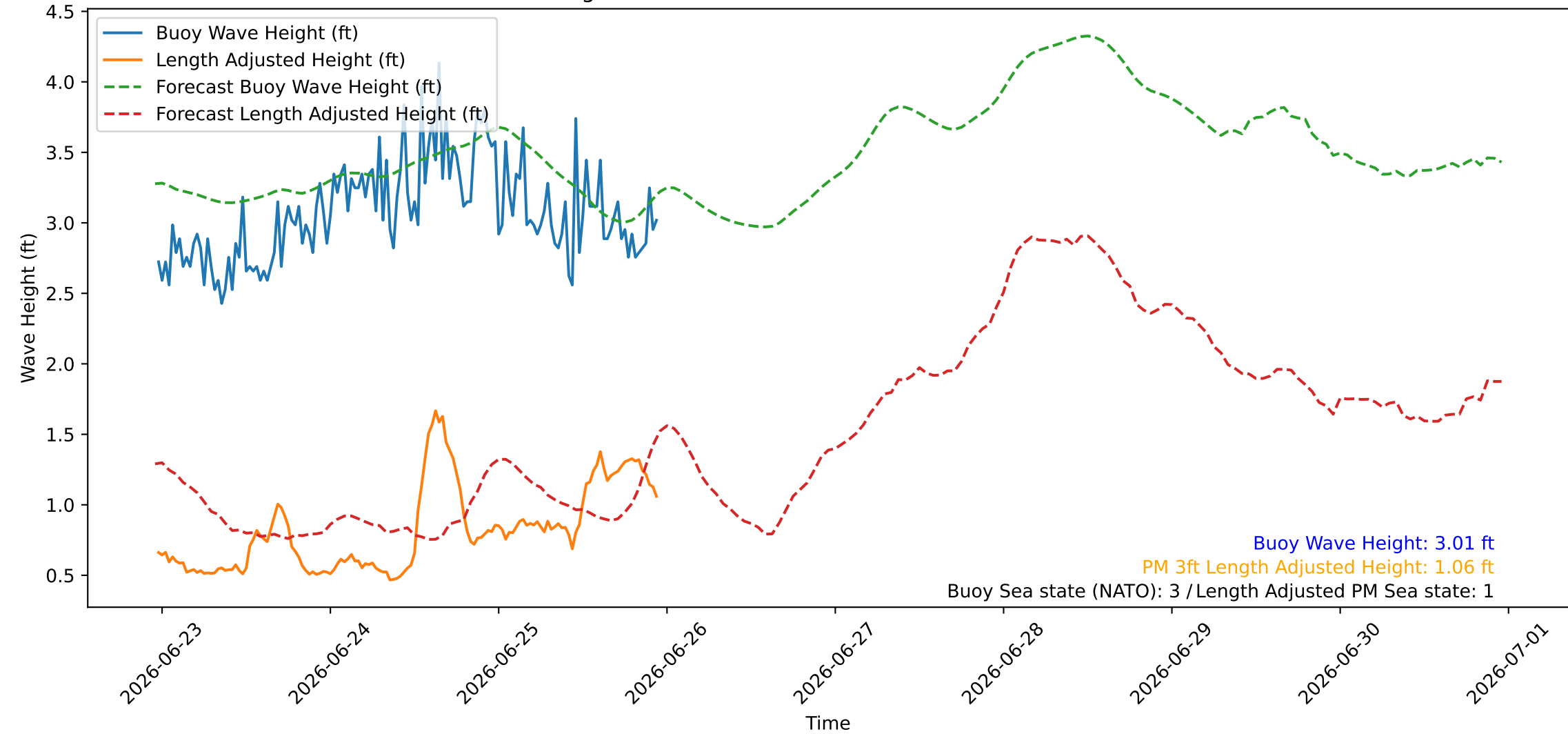
Wave Heights over Time for Red Beach at 2026-06-25 23:10:46
