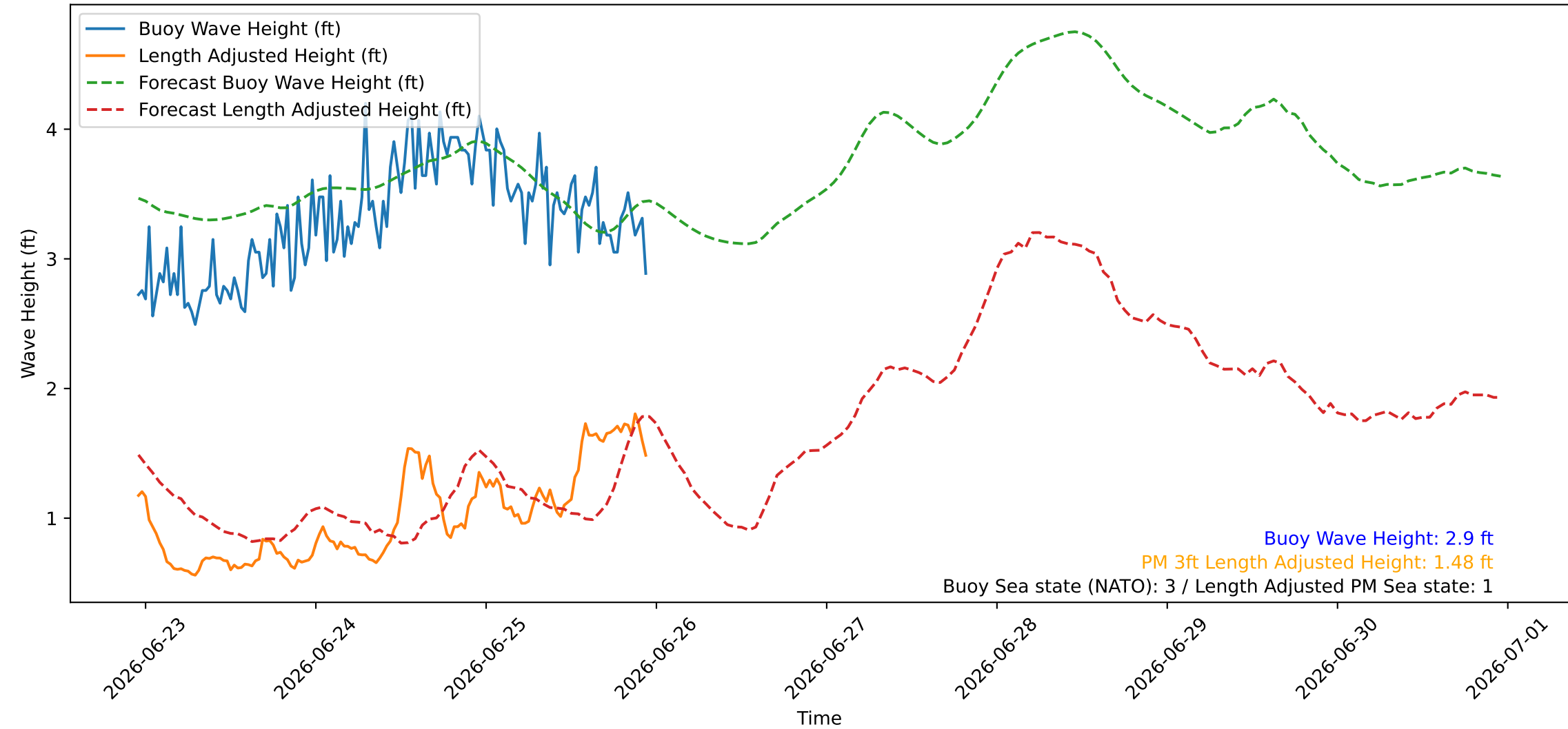
Wave Heights over Time for Green Beach at 2026-06-25 23:11:08
