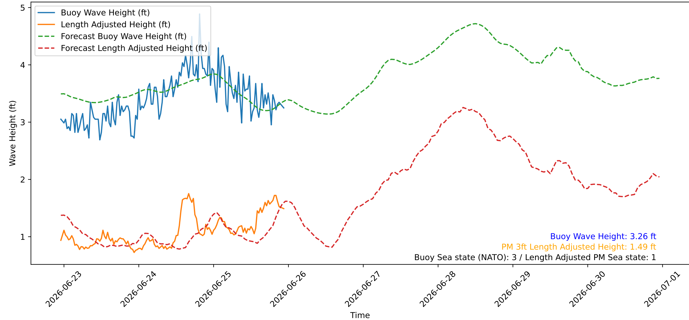
Wave Heights over Time for Oceanside Harbor at 2026-06-25 23:10:26
