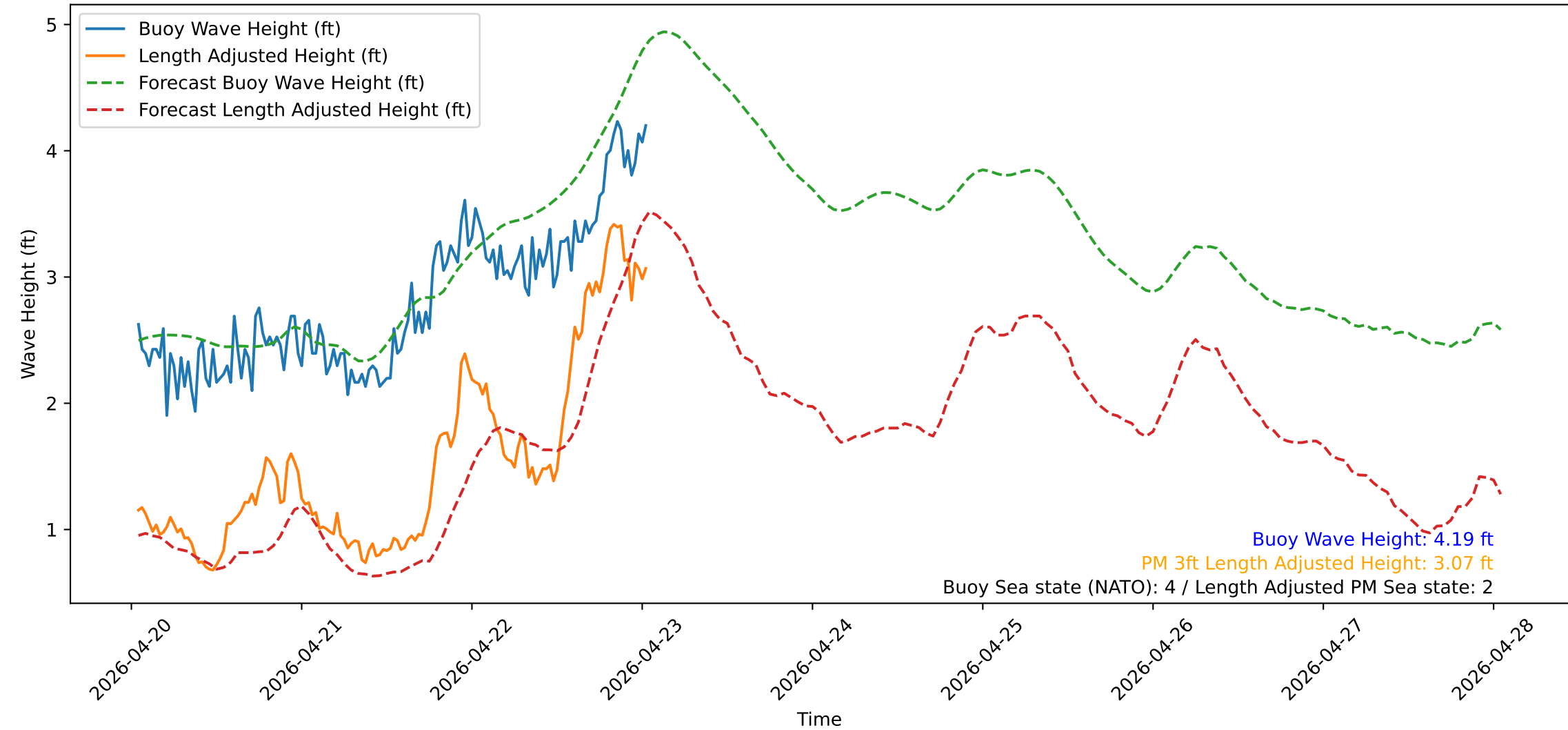
Wave Heights over Time for Oceanside Harbor at 2026-04-23 01:00:32
