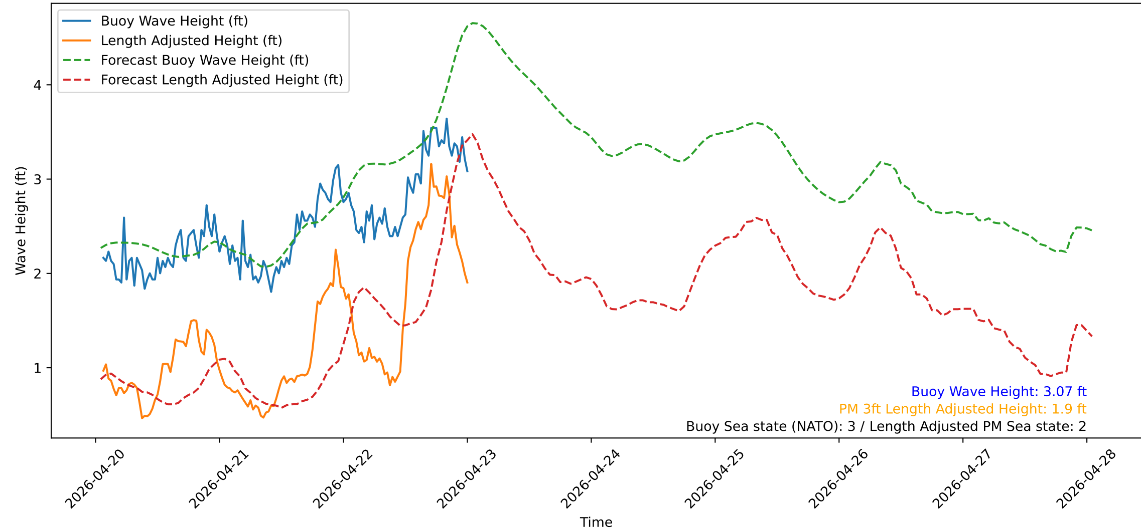
Wave Heights over Time for Red Beach at 2026-04-23 01:00:51
