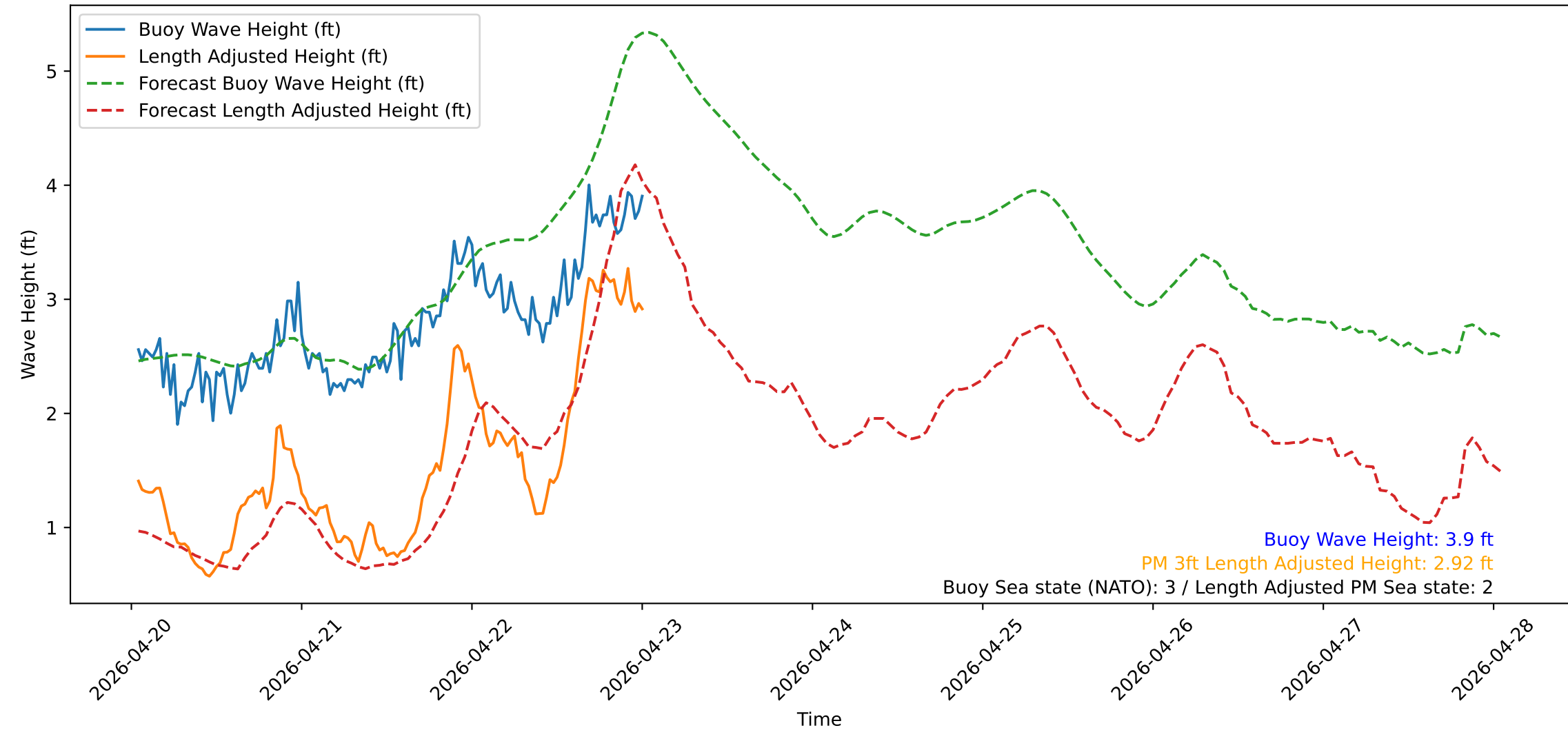
Wave Heights over Time for Green Beach at 2026-04-23 01:01:13
