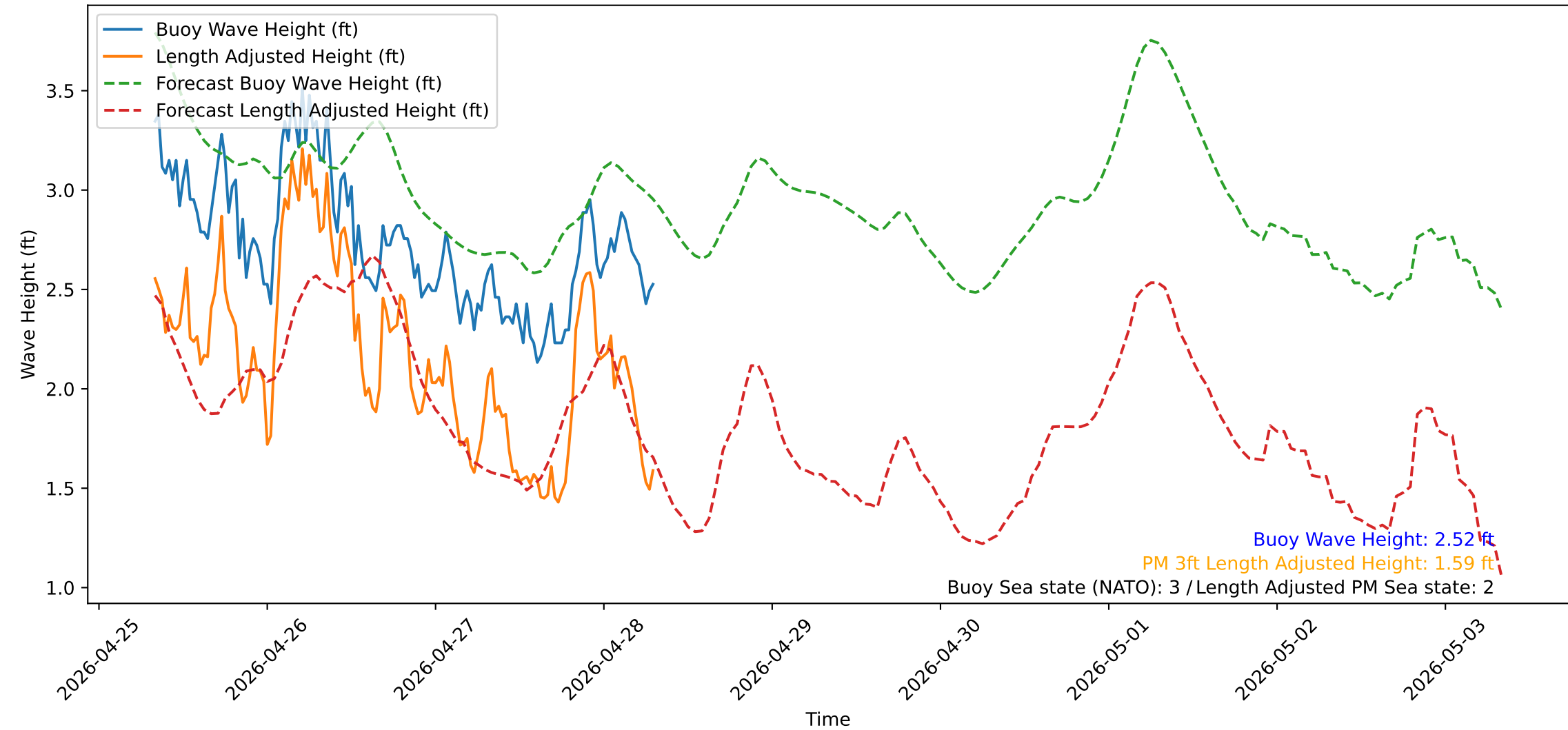
Wave Heights over Time for Green Beach at 2026-04-28 08:01:12
