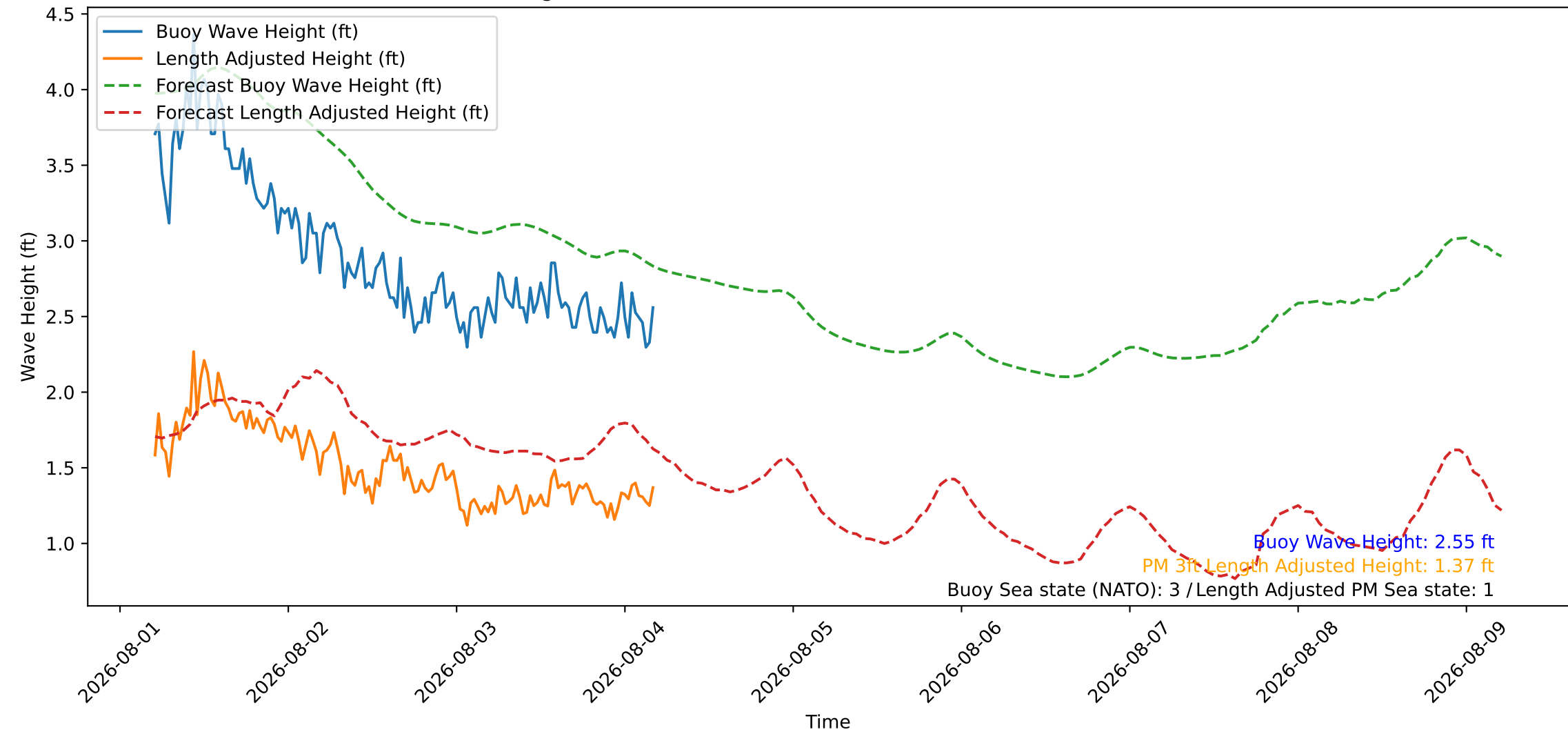
Wave Heights over Time for Oceanside Harbor at 2026-08-04 04:50:27
