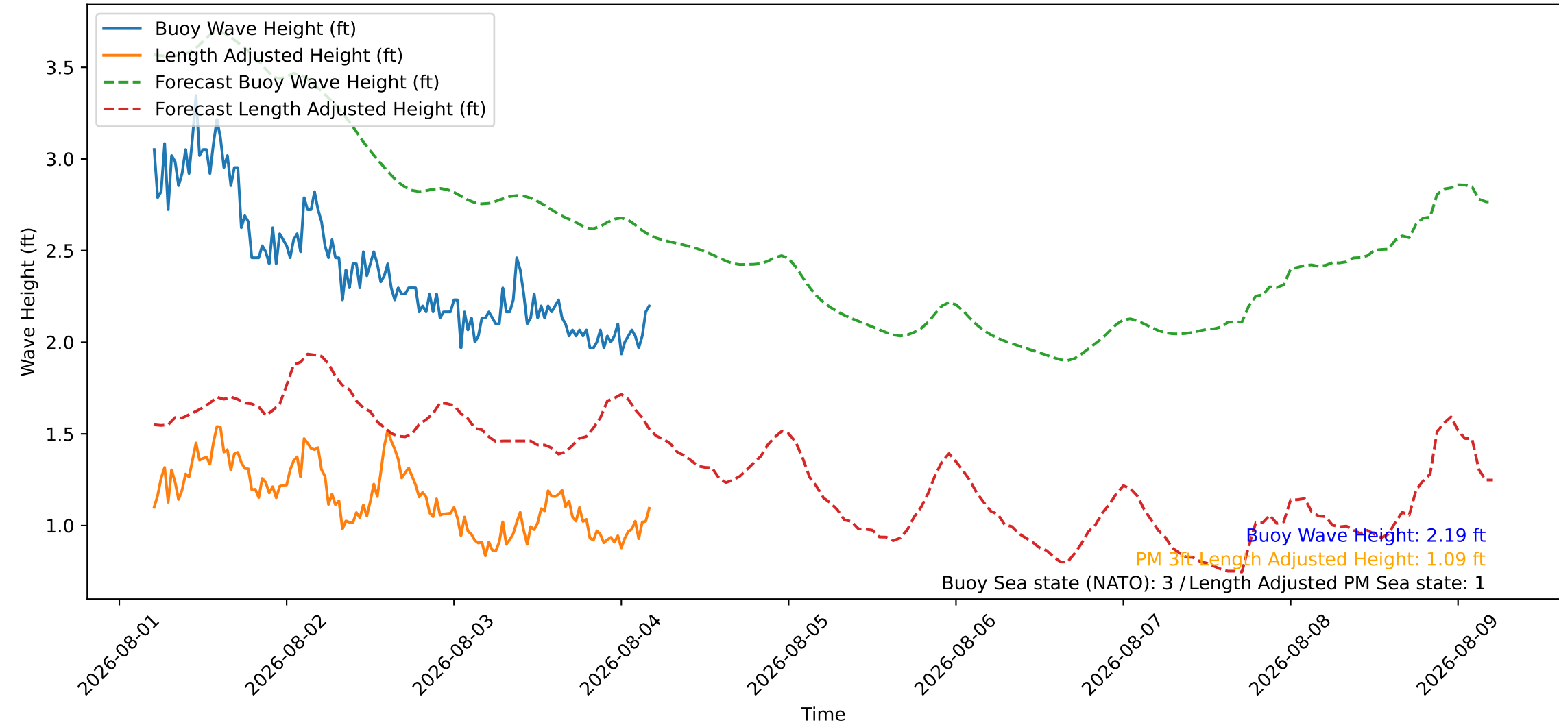
Wave Heights over Time for Red Beach at 2026-08-04 04:50:47
