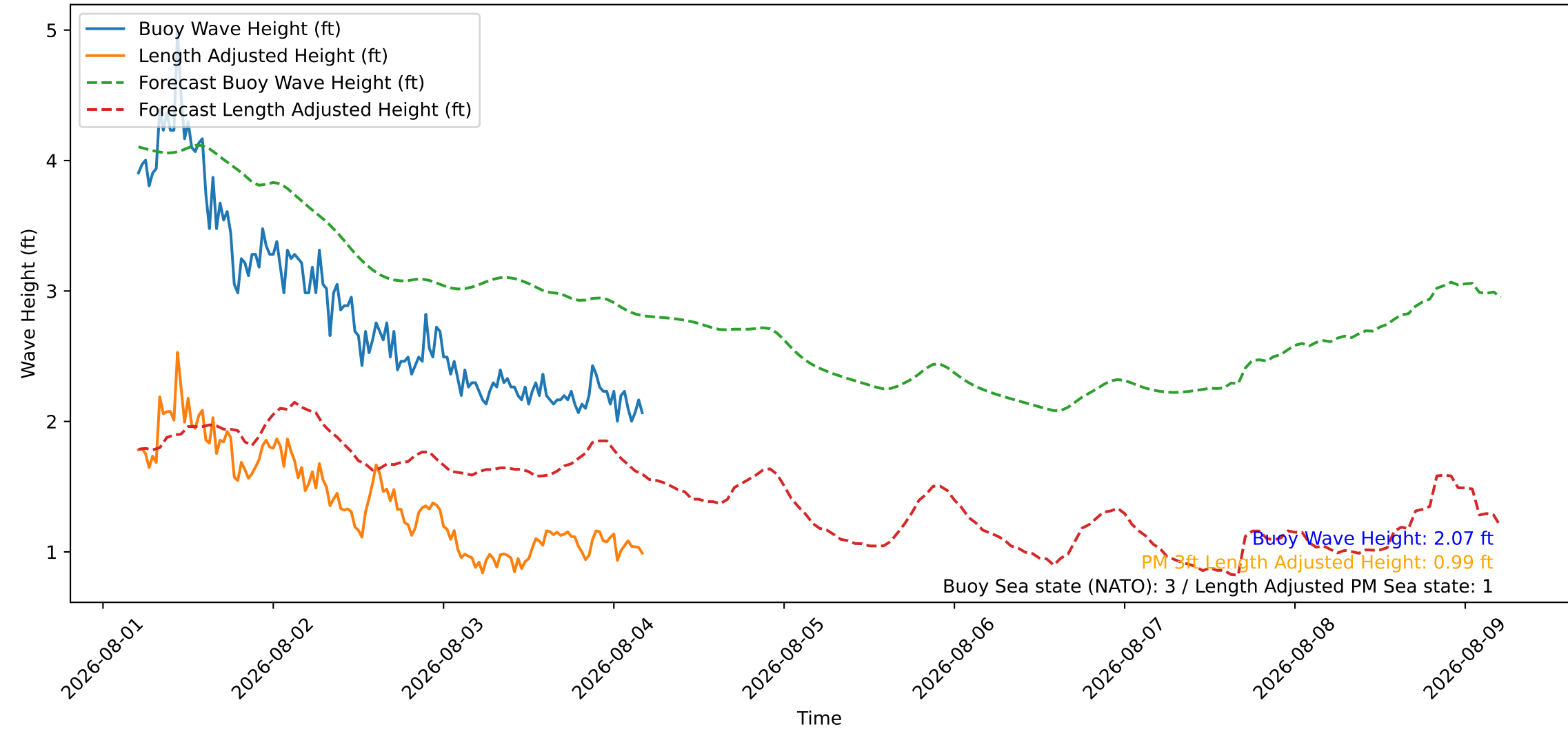
Wave Heights over Time for Green Beach at 2026-08-04 04:51:09
