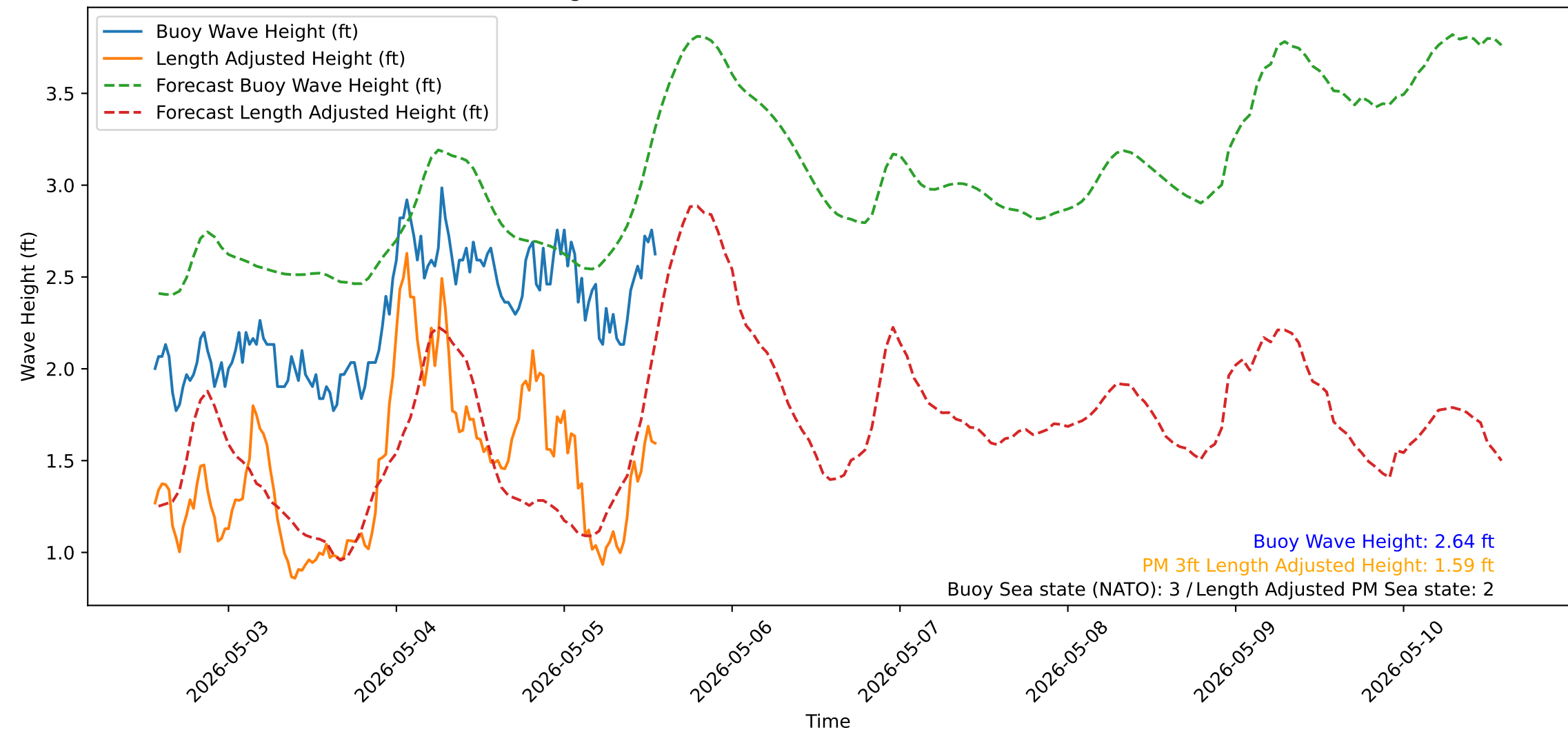
Wave Heights over Time for Green Beach at 2026-05-05 13:41:13
