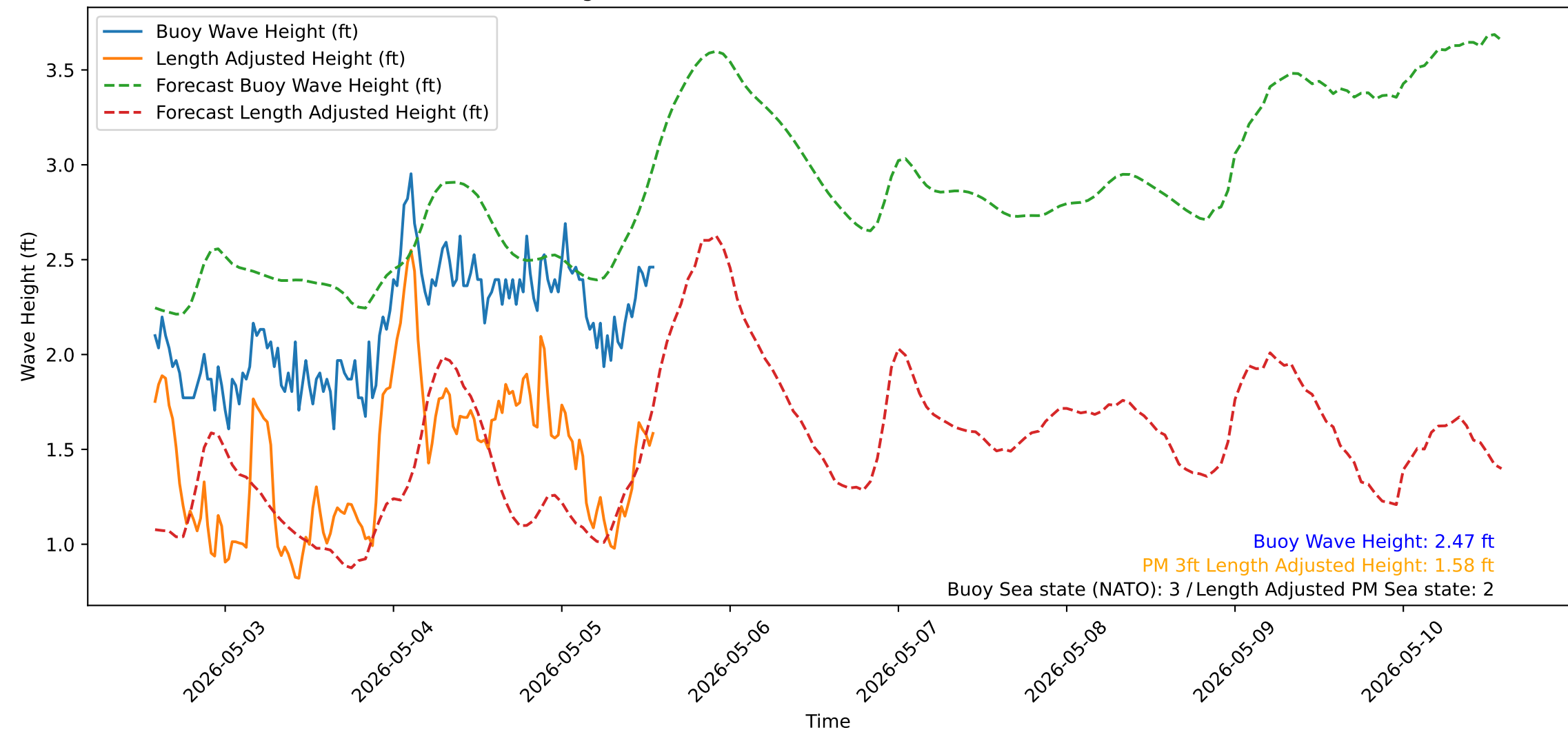
Wave Heights over Time for Red Beach at 2026-05-05 13:40:50
