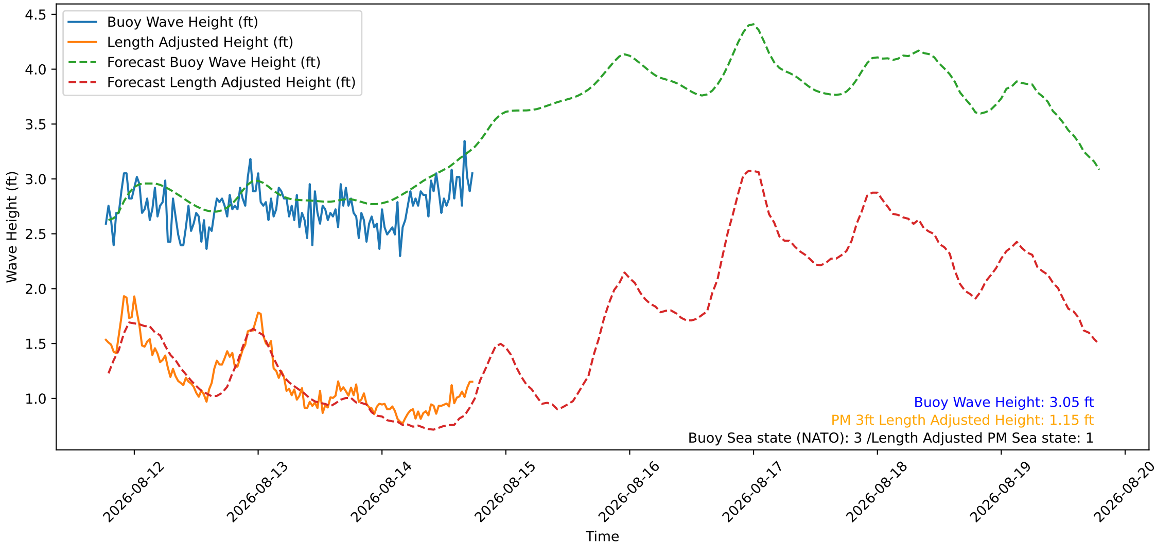
Wave Heights over Time for Oceanside Harbor at 2026-08-14 18:30:26
