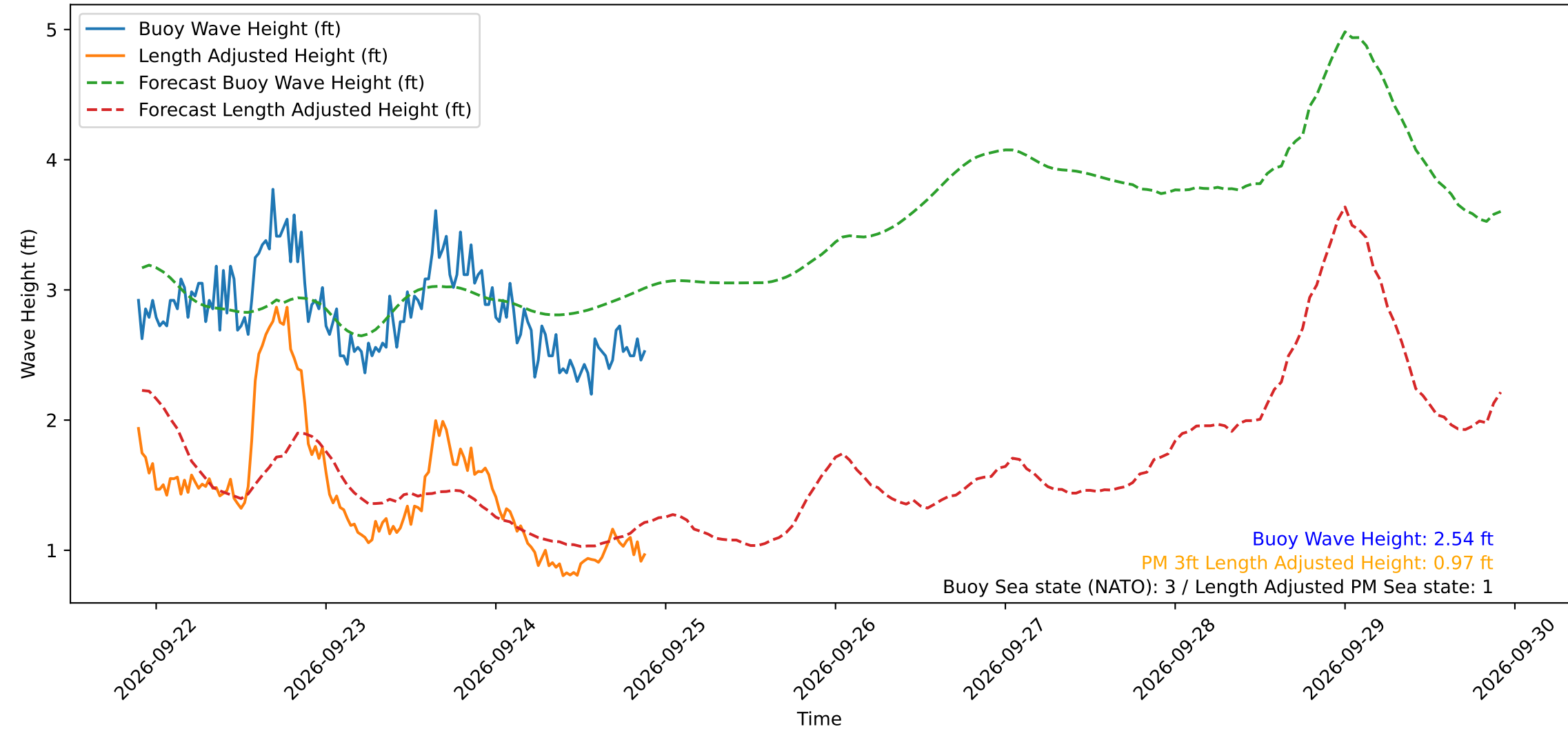
Wave Heights over Time for Oceanside Harbor at 2026-09-24 21:40:30
