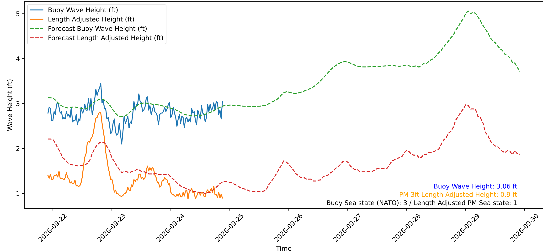
Wave Heights over Time for Green Beach at 2026-09-24 21:41:12
