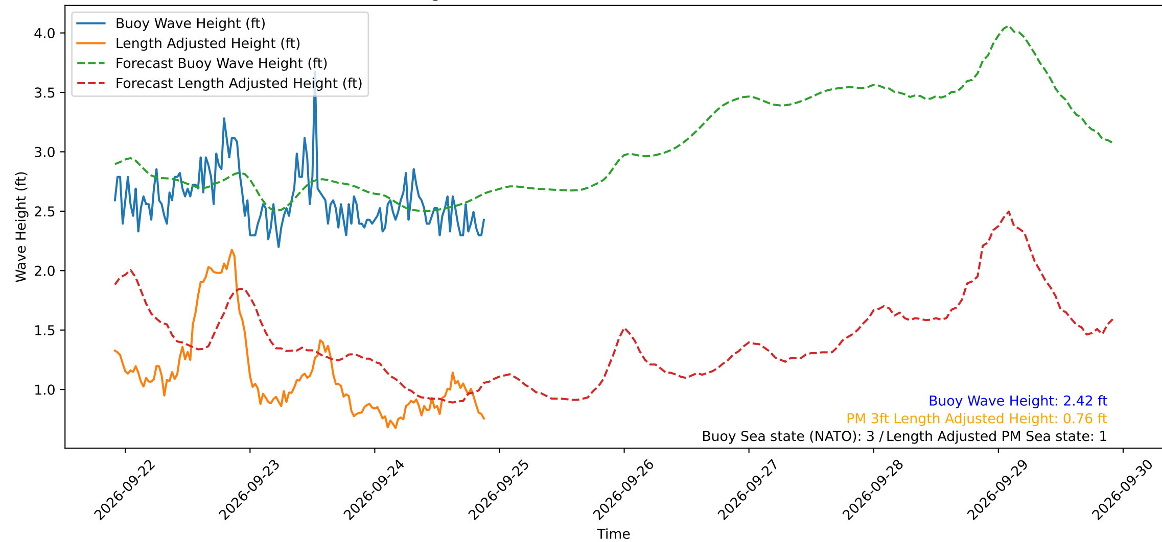
Wave Heights over Time for Red Beach at 2026-09-24 21:40:49
