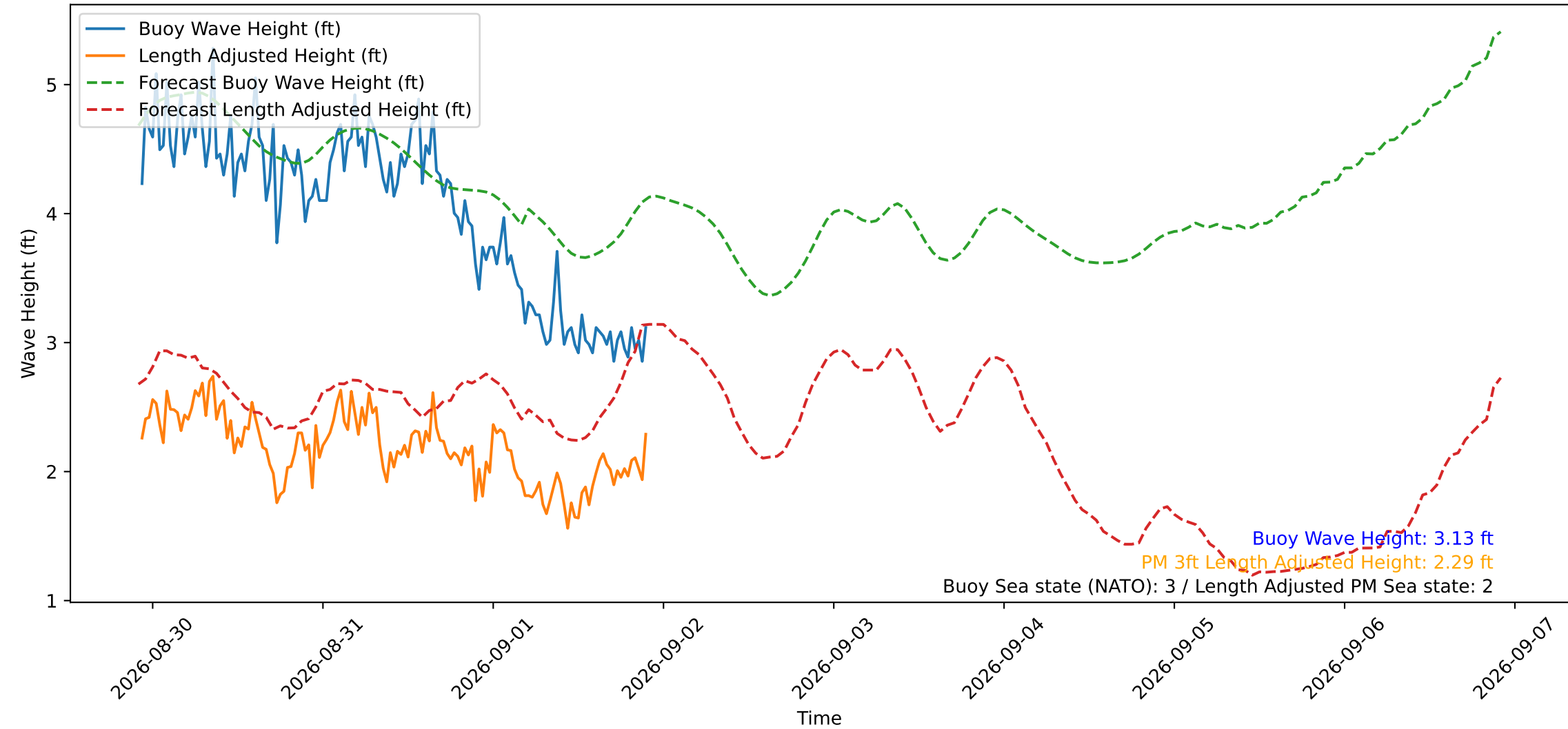
Wave Heights over Time for Oceanside Harbor at 2026-09-01 22:20:29
