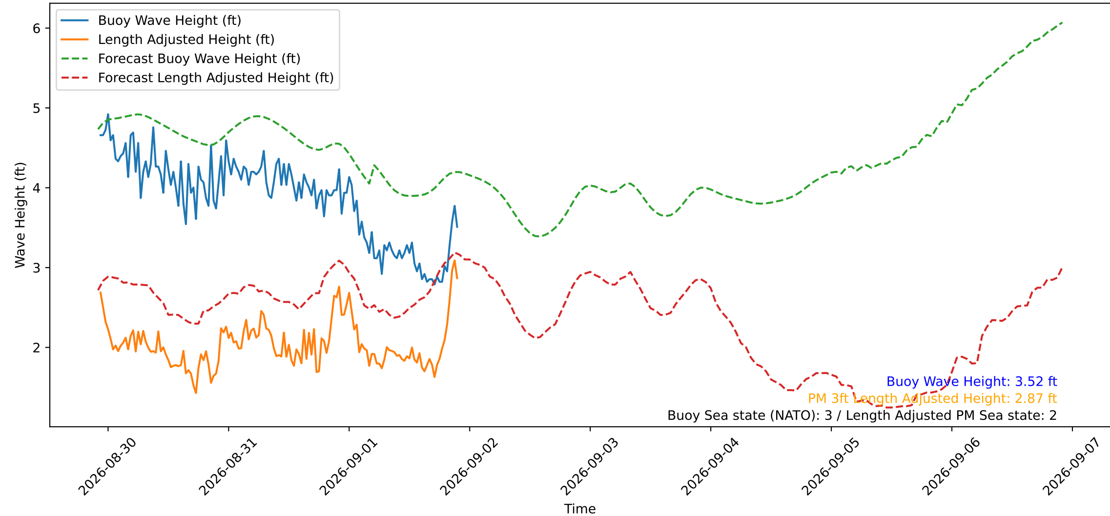
Wave Heights over Time for Green Beach at 2026-09-01 22:21:15
