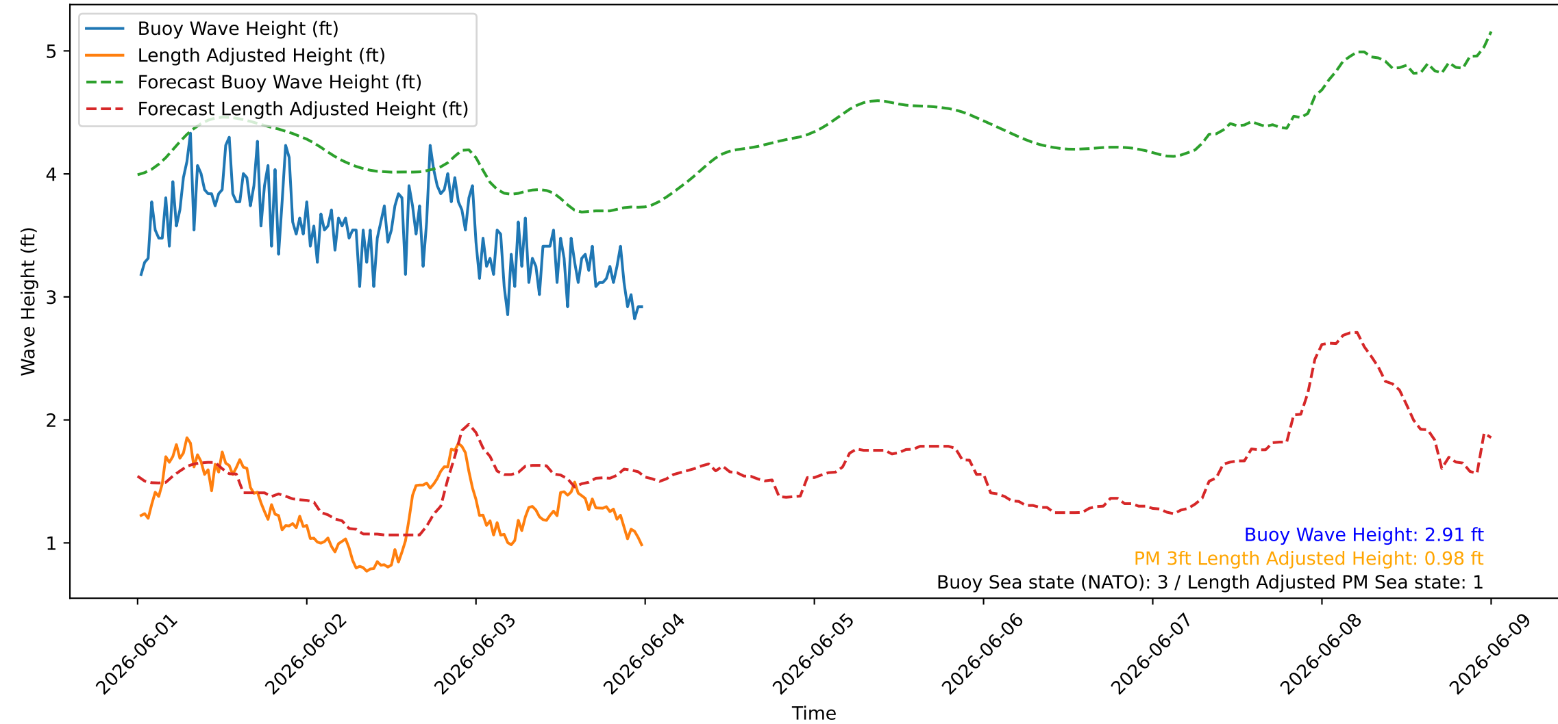
Wave Heights over Time for Green Beach at 2026-06-04 00:21:09
