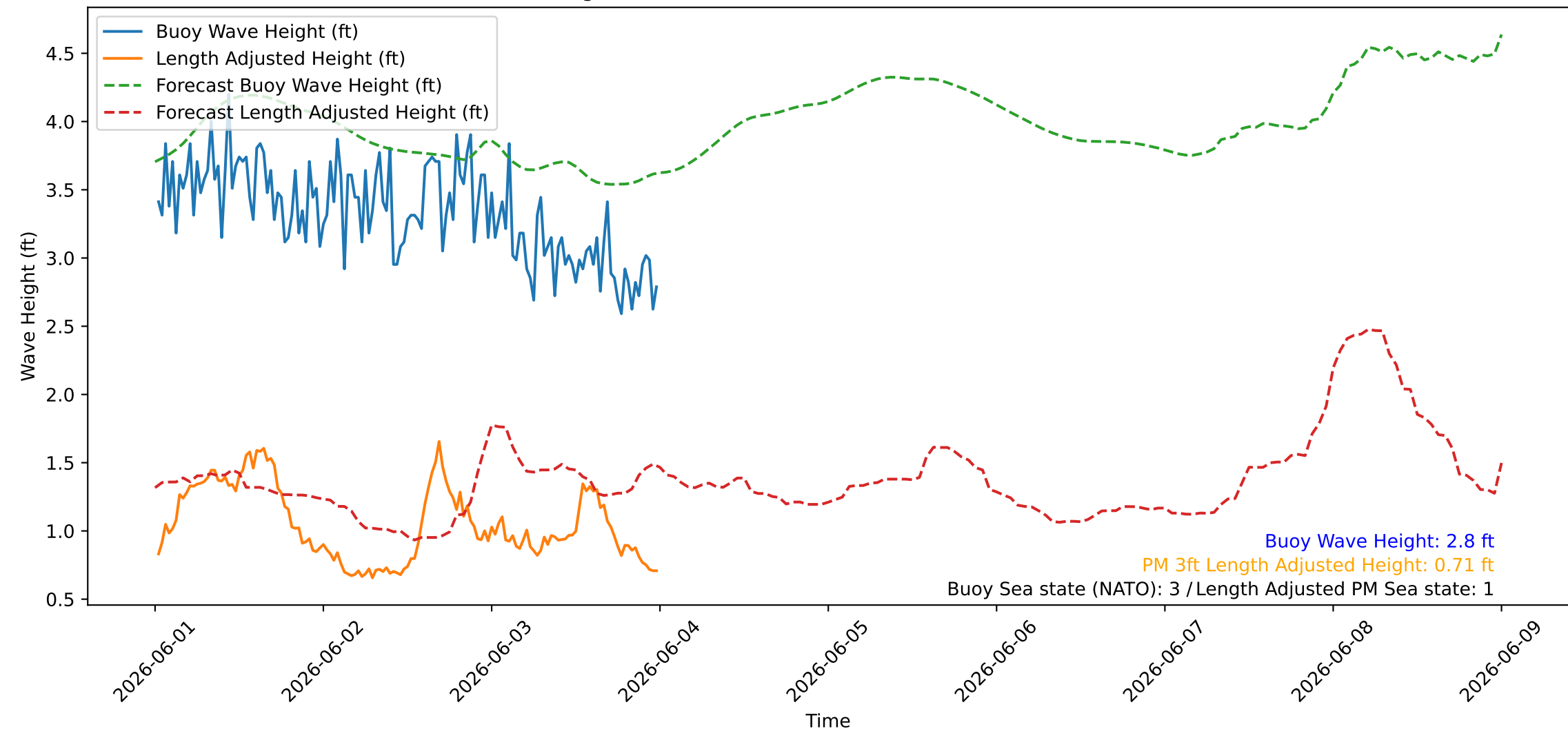
Wave Heights over Time for Red Beach at 2026-06-04 00:20:46
