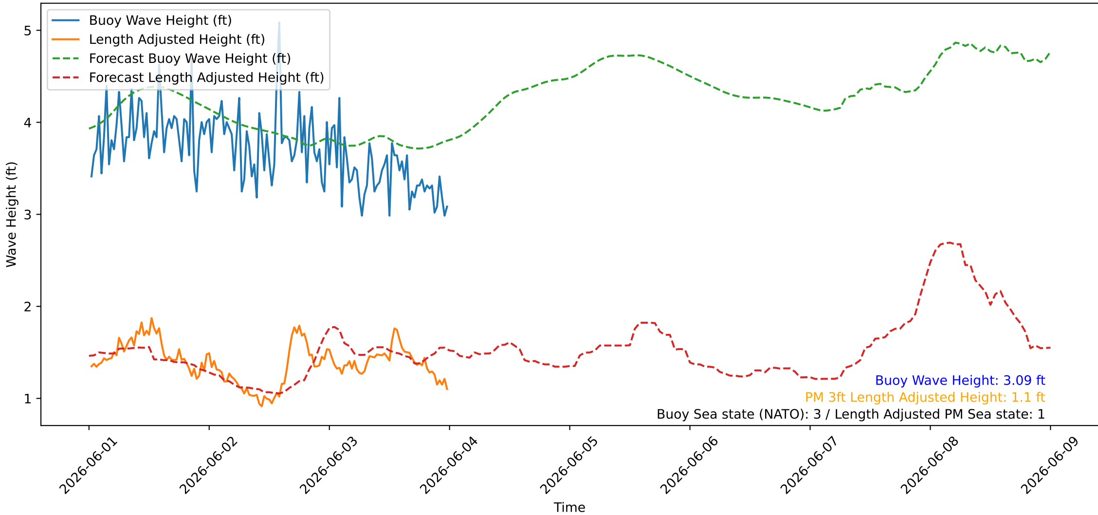
Wave Heights over Time for Oceanside Harbor at 2026-06-04 00:20:26
