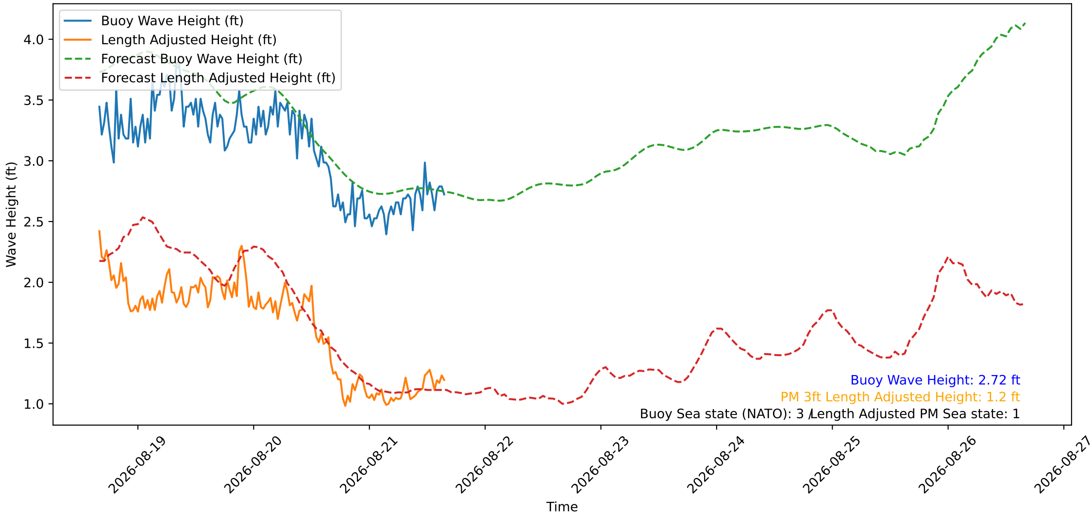
Wave Heights over Time for Oceanside Harbor at 2026-08-21 16:10:27
