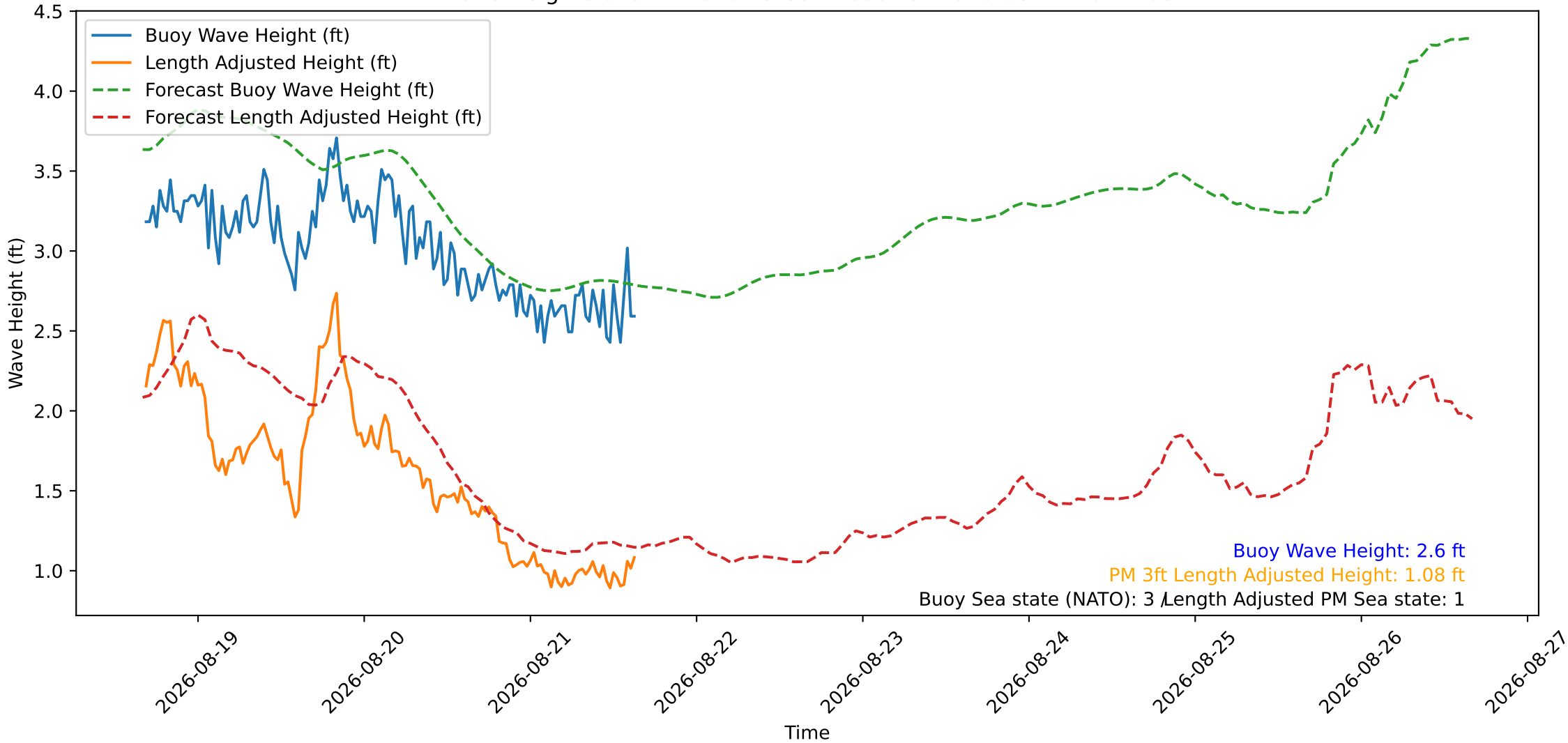
Wave Heights over Time for Green Beach at 2026-08-21 16:11:08
