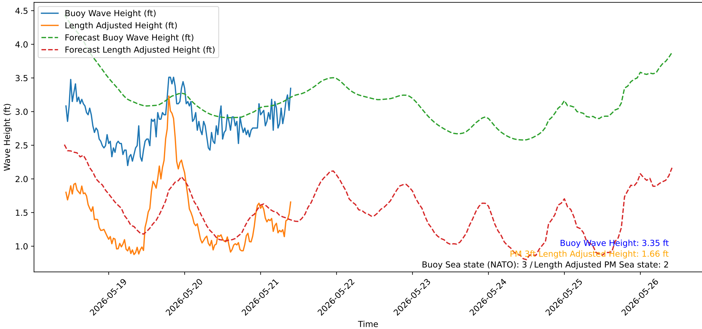
Wave Heights over Time for Oceanside Harbor at 2026-05-21 10:20:31
