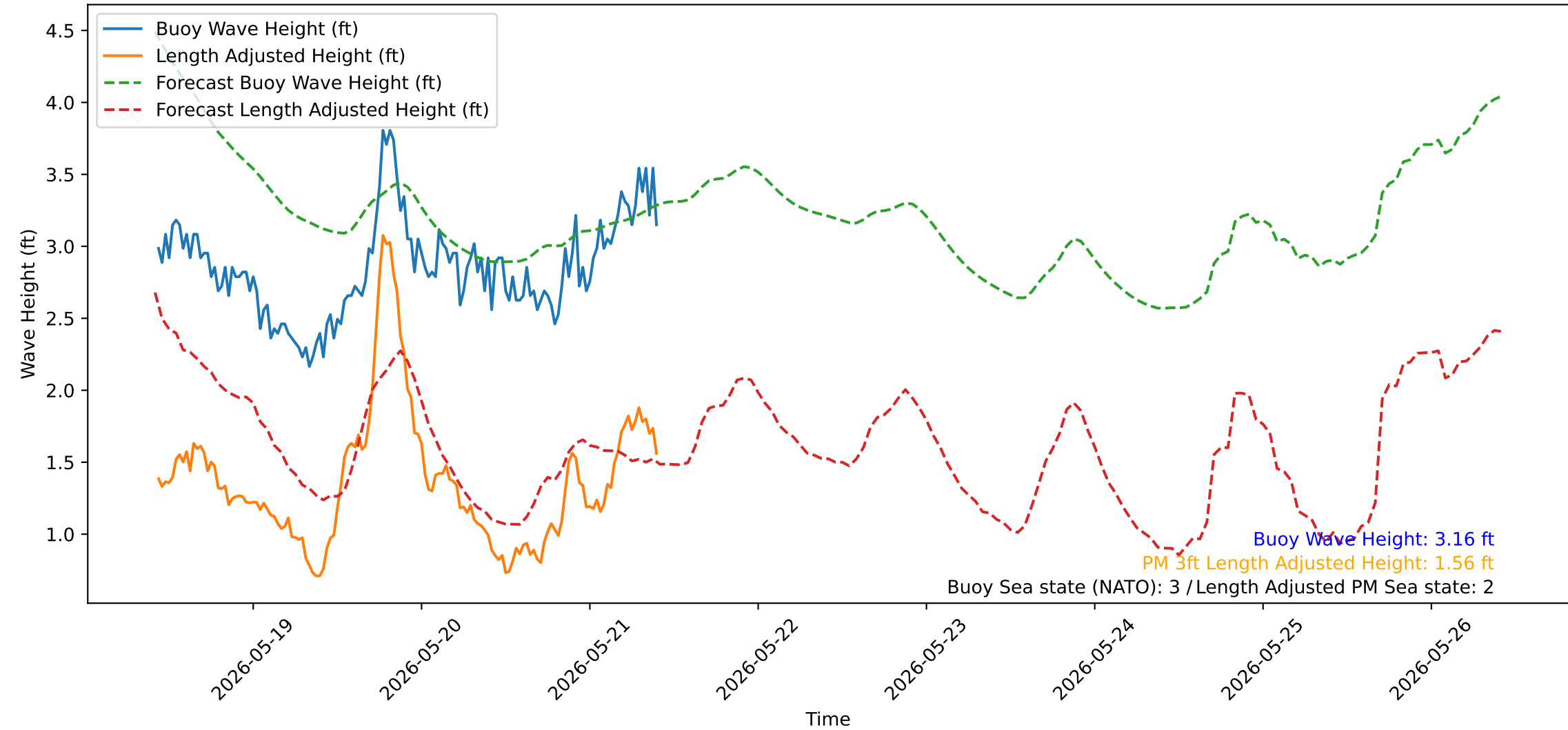
Wave Heights over Time for Green Beach at 2026-05-21 10:21:14
