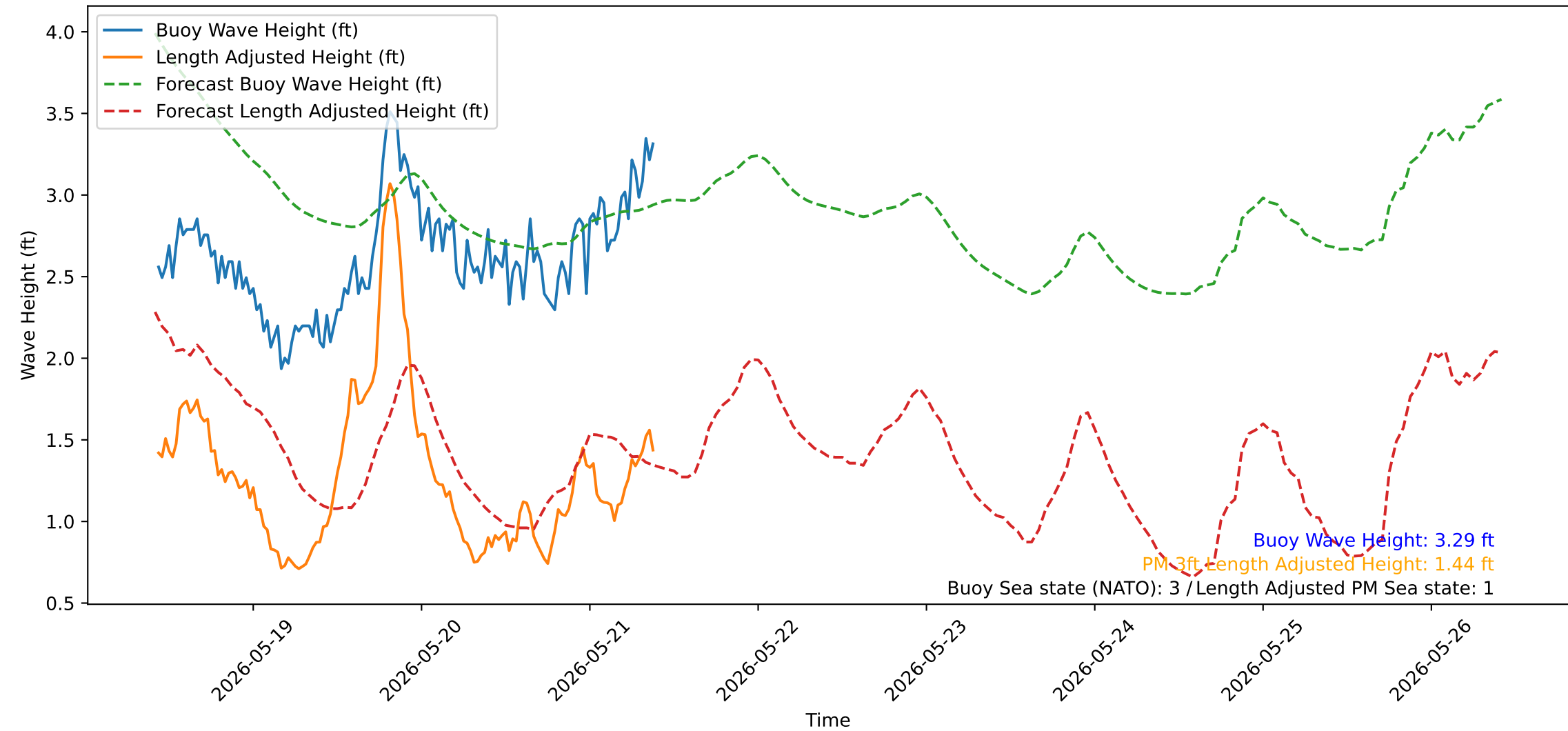
Wave Heights over Time for Red Beach at 2026-05-21 10:20:52
