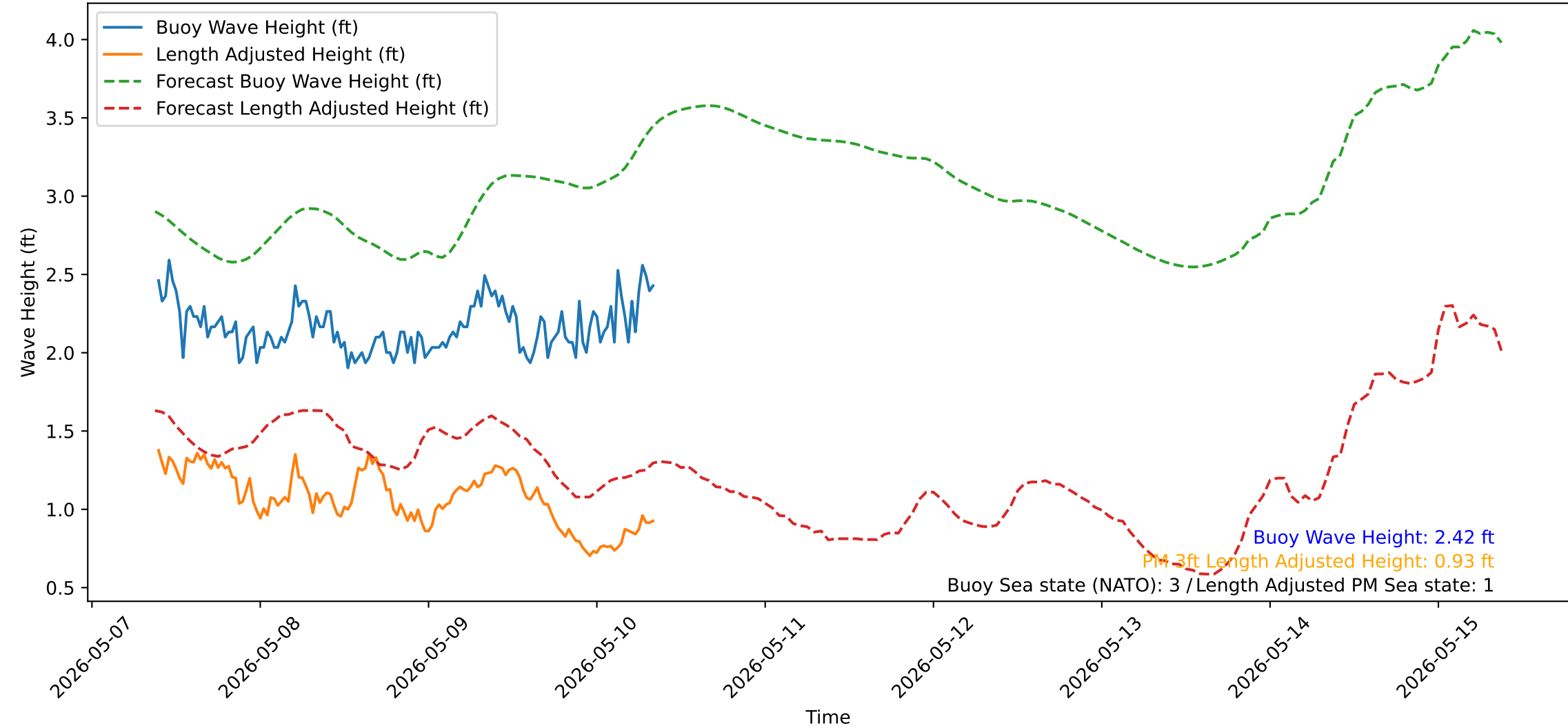
Wave Heights over Time for Red Beach at 2026-05-10 09:10:51
