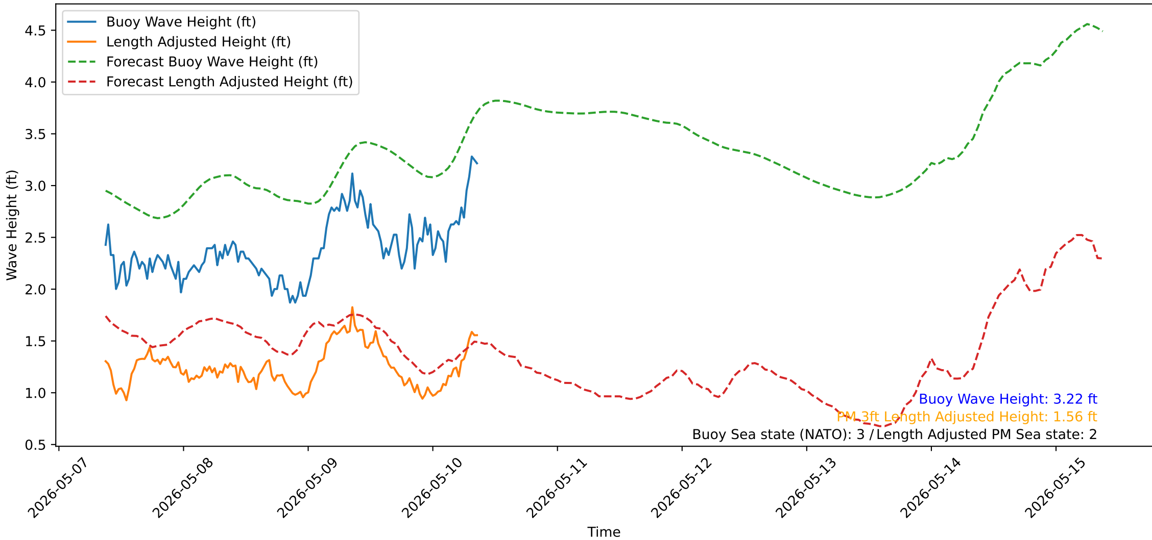
Wave Heights over Time for Oceanside Harbor at 2026-05-10 09:10:32
