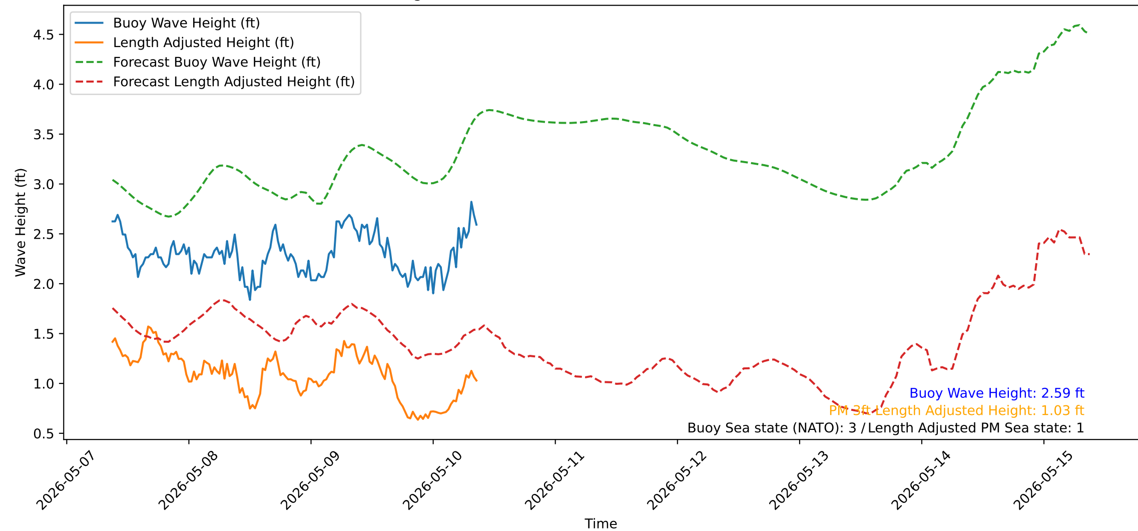
Wave Heights over Time for Green Beach at 2026-05-10 09:11:14
