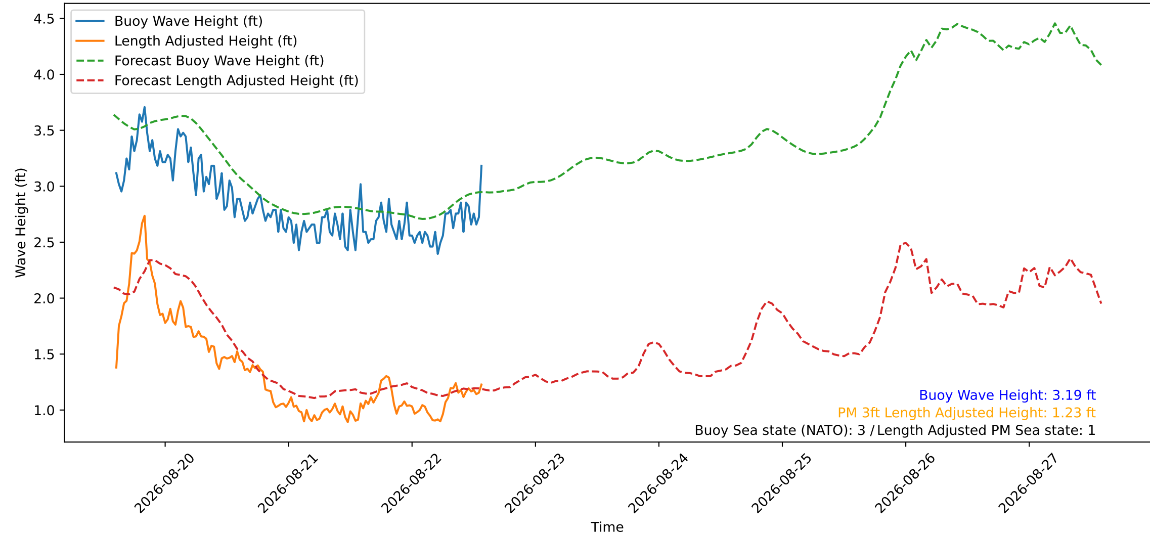
Wave Heights over Time for Green Beach at 2026-08-22 14:21:15
