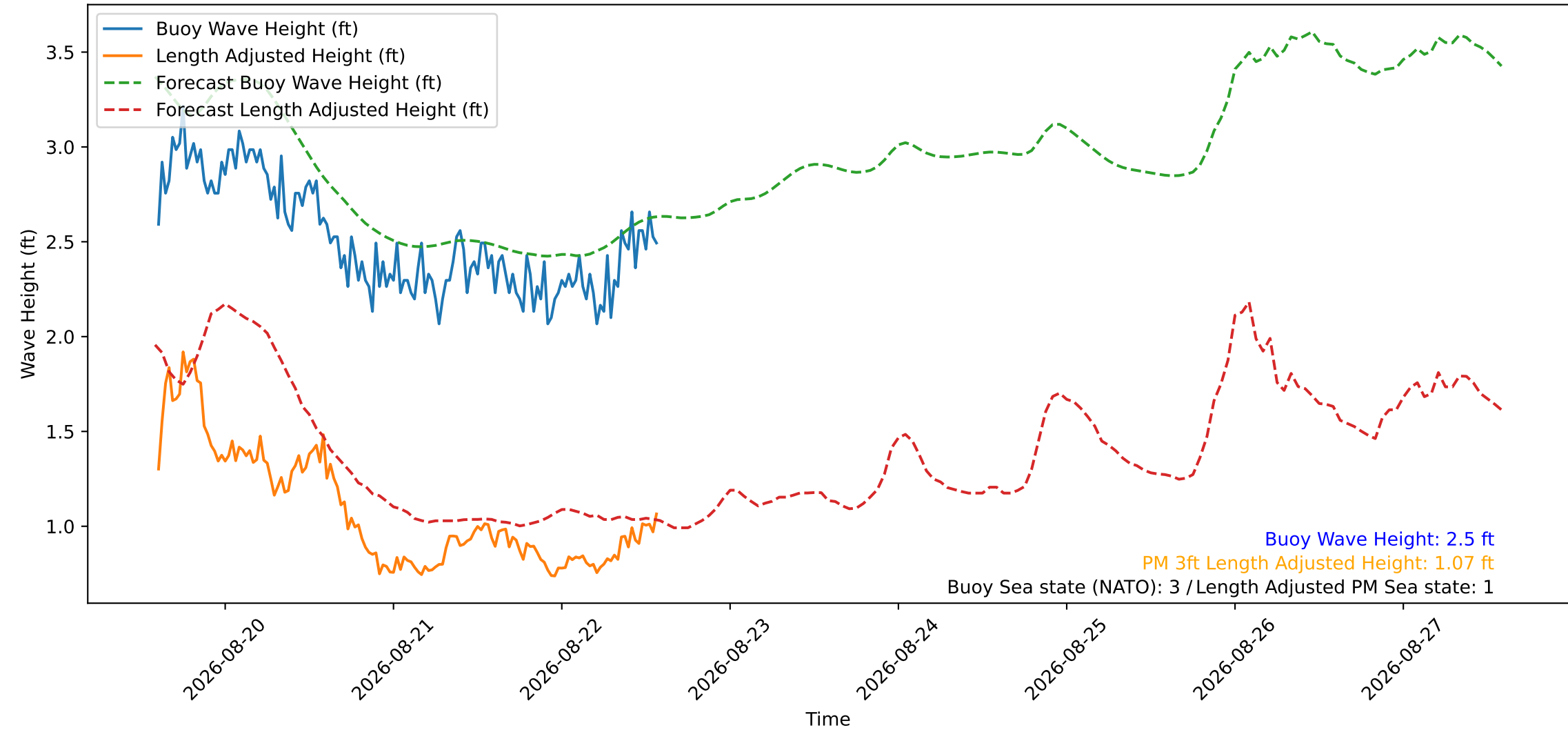
Wave Heights over Time for Red Beach at 2026-08-22 14:20:50
