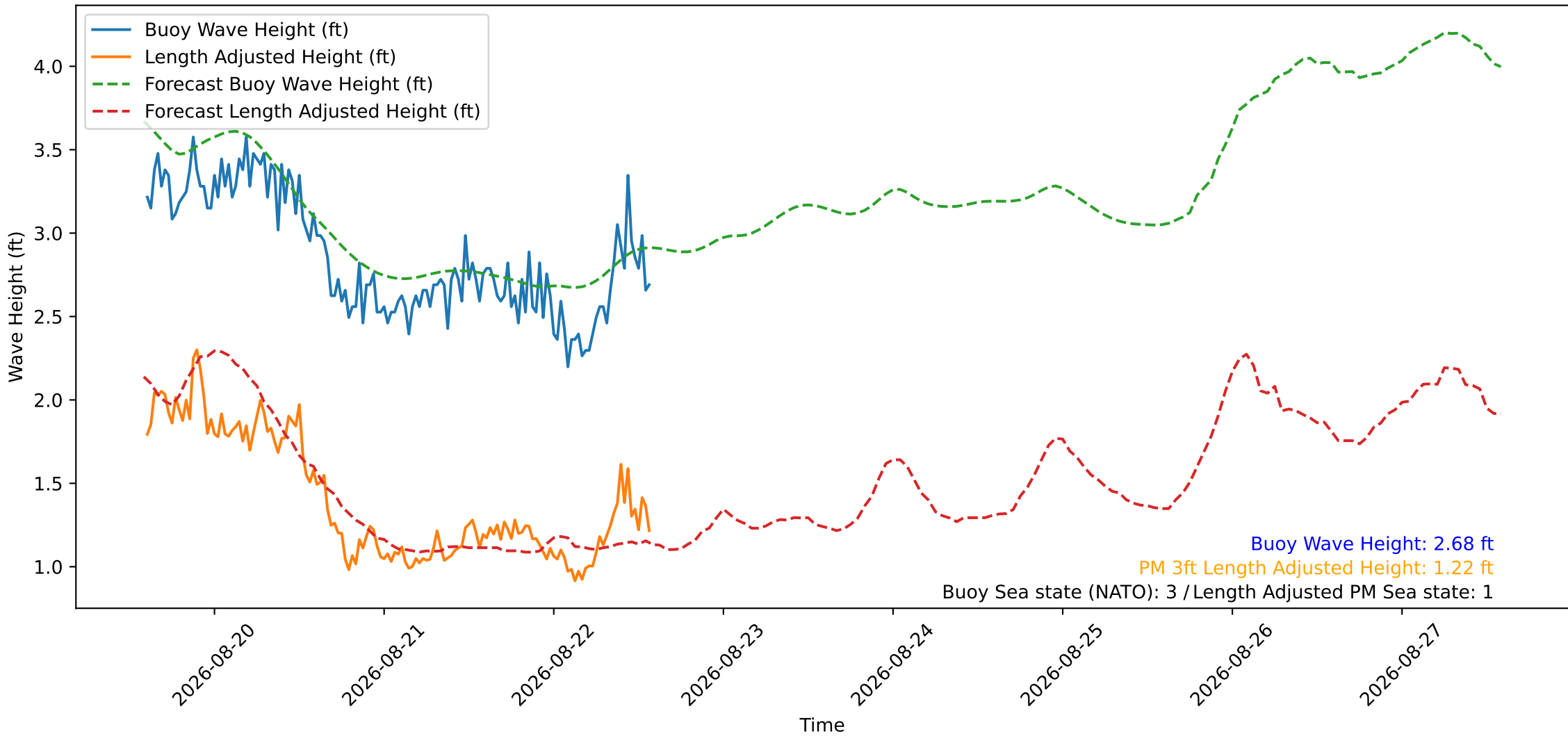
Wave Heights over Time for Oceanside Harbor at 2026-08-22 14:20:30
