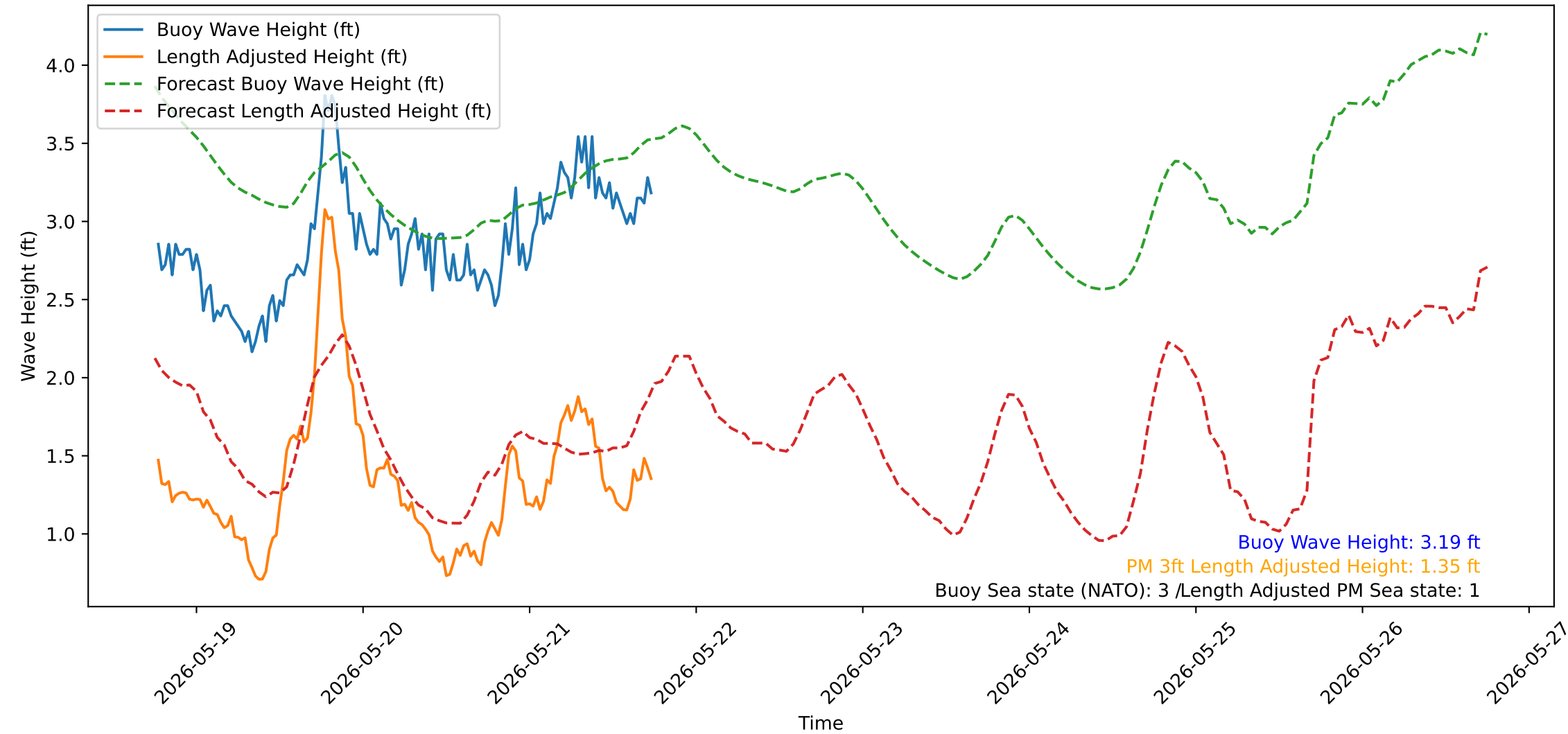
Wave Heights over Time for Green Beach at 2026-05-21 18:21:15
