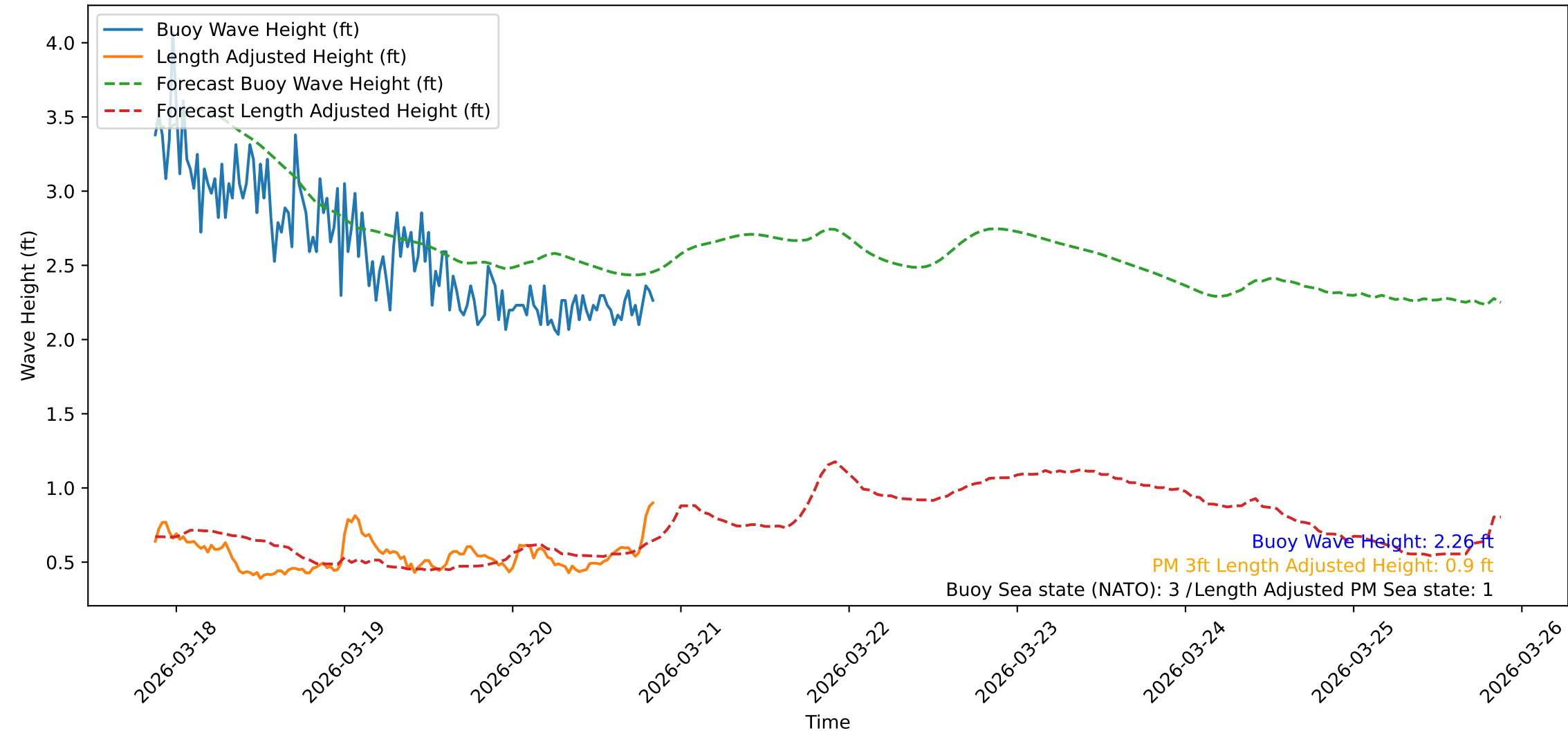
Wave Heights over Time for Green Beach at 2026-03-20 21:01:10
