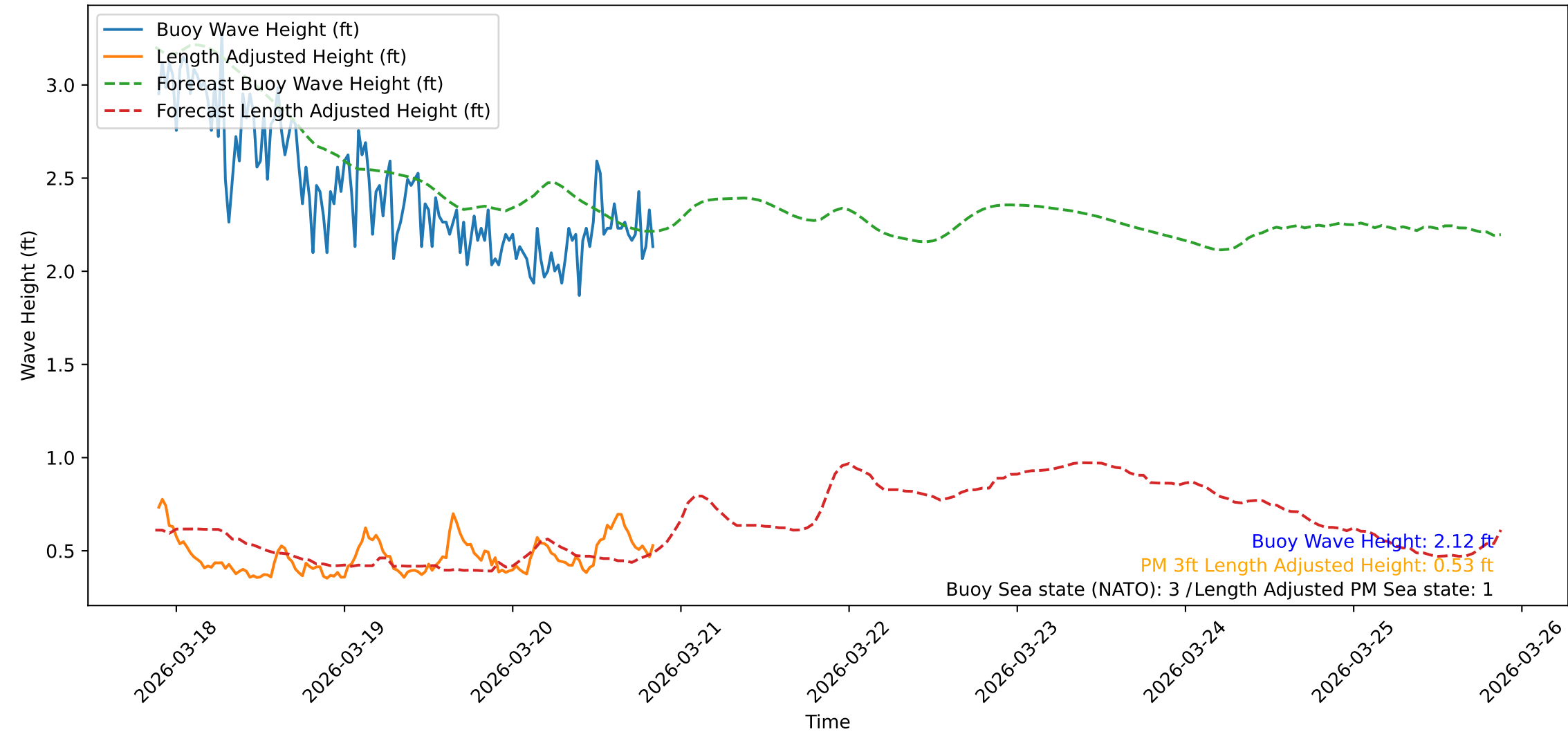
Wave Heights over Time for Red Beach at 2026-03-20 21:00:48
