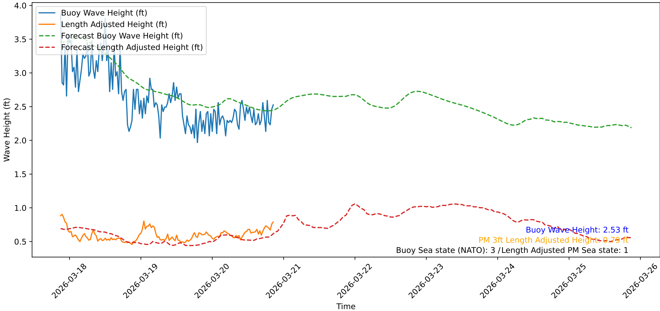
Wave Heights over Time for Oceanside Harbor at 2026-03-20 21:00:32
