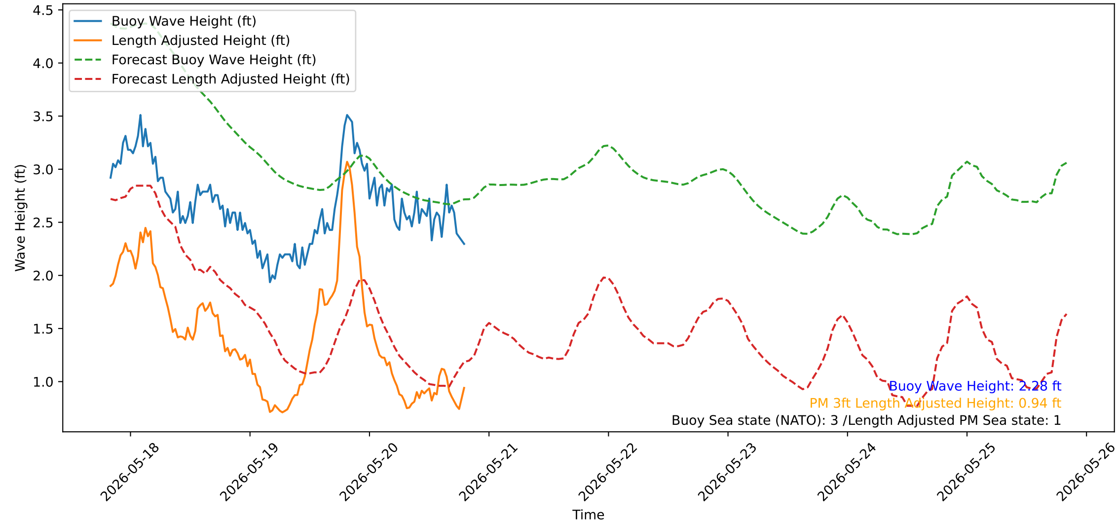
Wave Heights over Time for Red Beach at 2026-05-20 19:50:52
