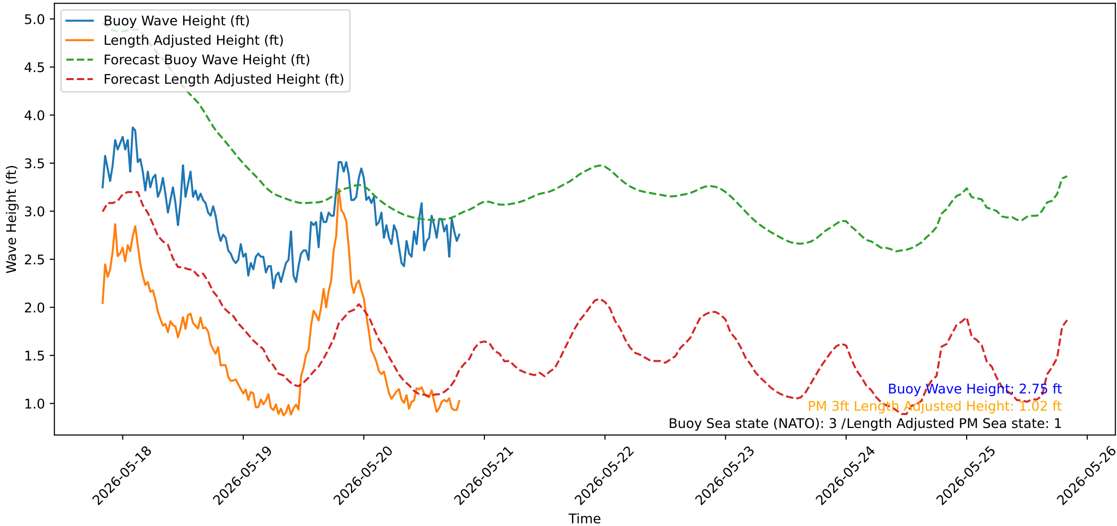
Wave Heights over Time for Oceanside Harbor at 2026-05-20 19:50:32
