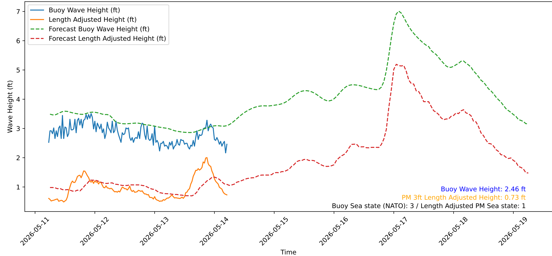
Wave Heights over Time for Green Beach at 2026-05-14 05:41:14
