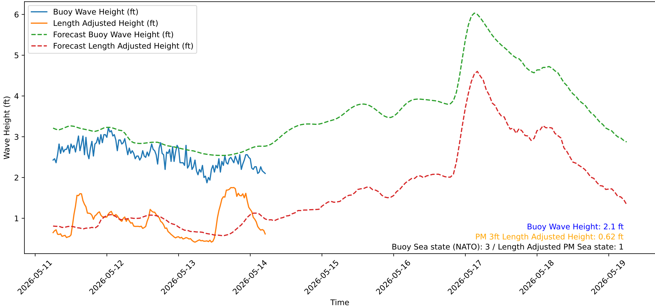
Wave Heights over Time for Red Beach at 2026-05-14 05:40:51
