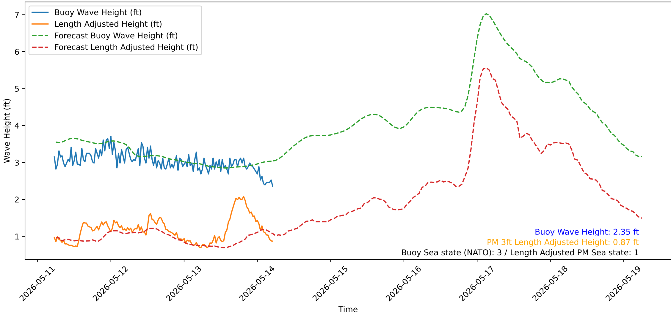
Wave Heights over Time for Oceanside Harbor at 2026-05-14 05:40:32
