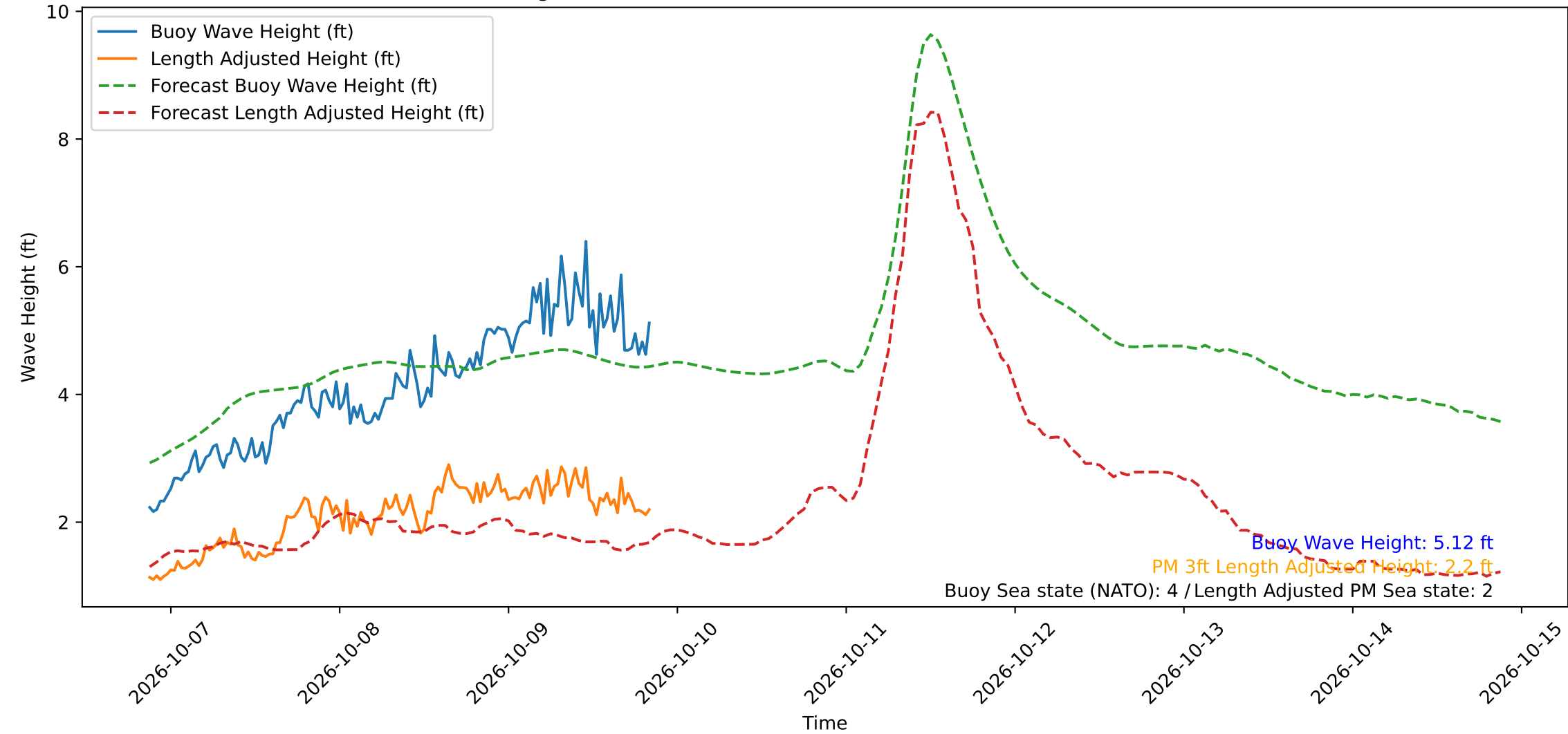
Wave Heights over Time for Oceanside Harbor at 2026-10-09 20:50:30
