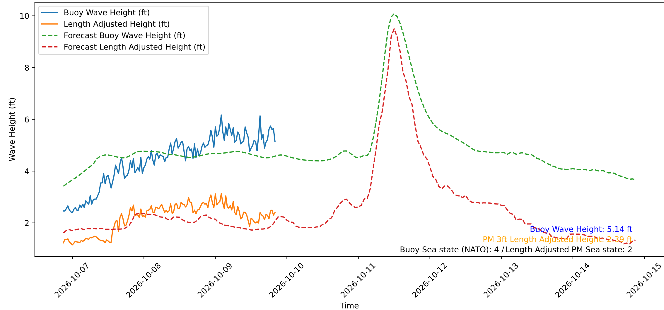
Wave Heights over Time for Green Beach at 2026-10-09 20:51:15
