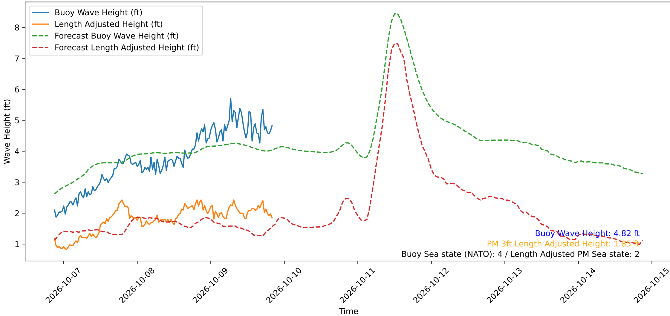
Wave Heights over Time for Red Beach at 2026-10-09 20:50:51
