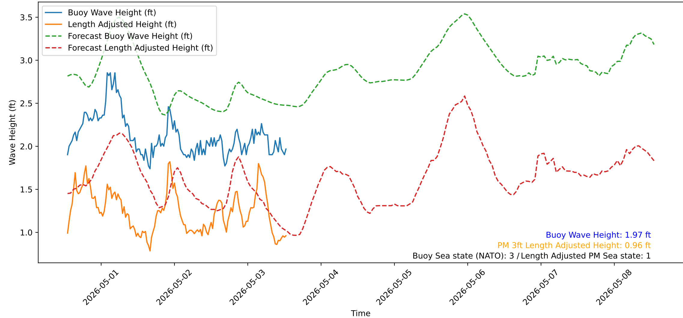
Wave Heights over Time for Green Beach at 2026-05-03 13:11:11
