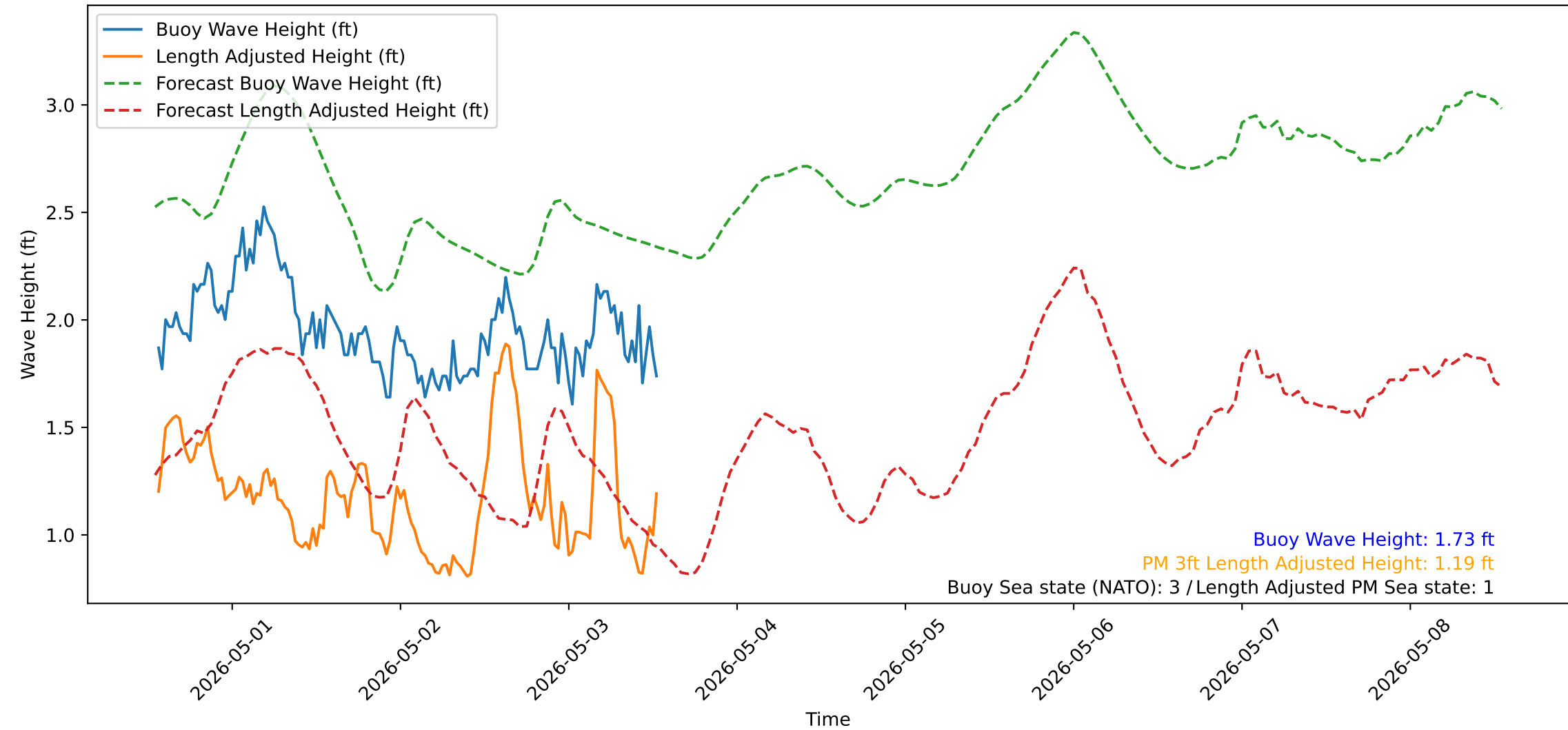
Wave Heights over Time for Red Beach at 2026-05-03 13:10:50
