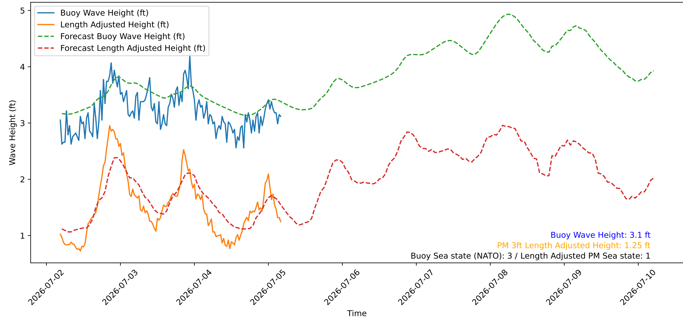
Wave Heights over Time for Green Beach at 2026-07-05 04:41:08
