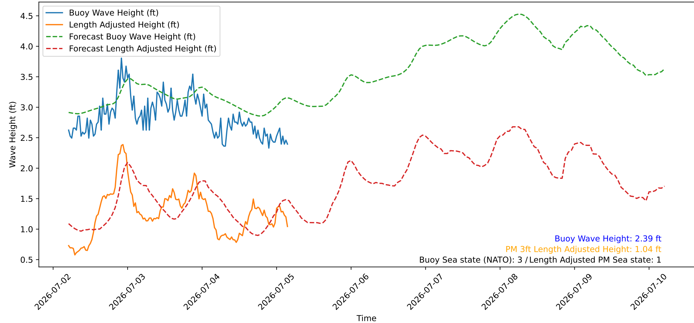
Wave Heights over Time for Red Beach at 2026-07-05 04:40:46
