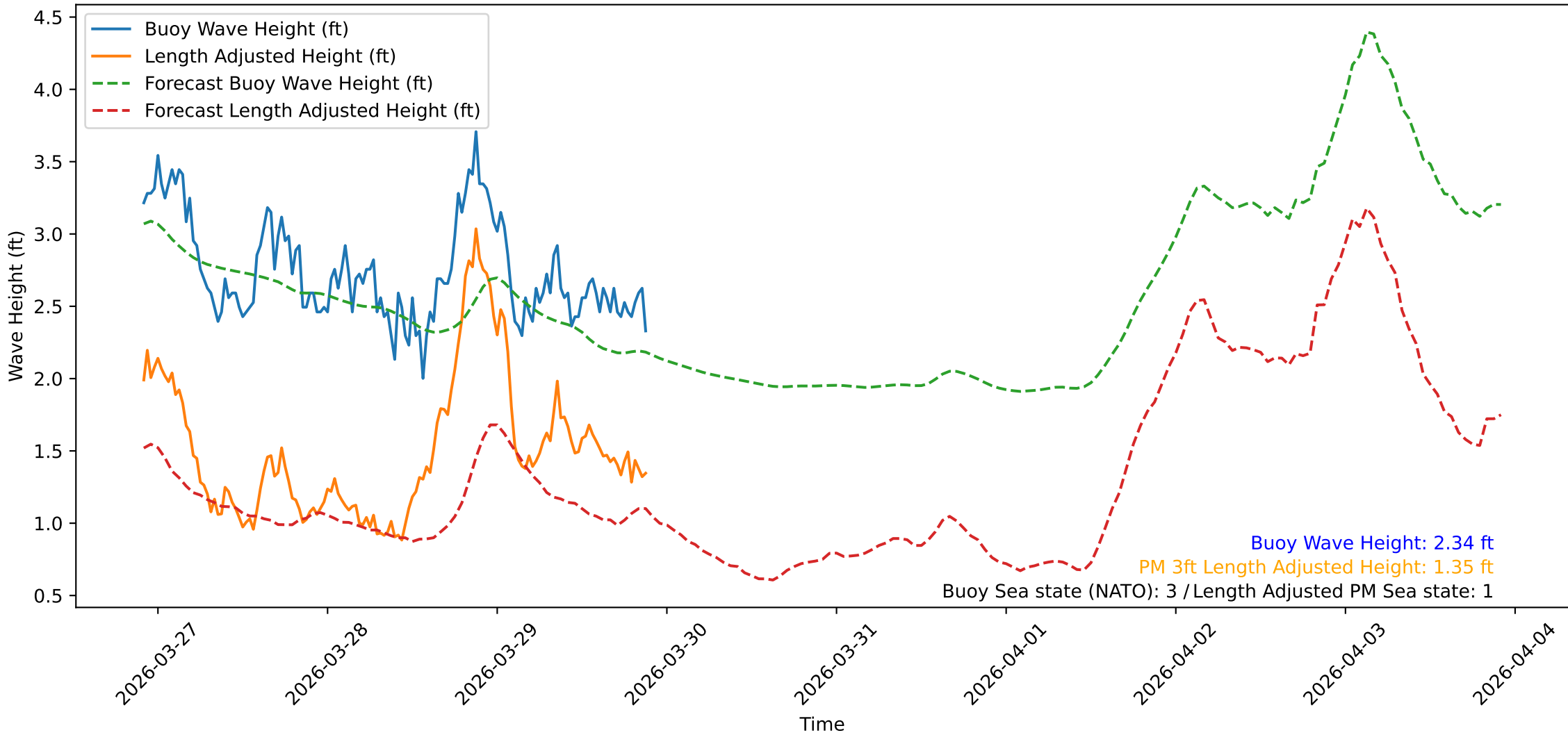
Wave Heights over Time for Green Beach at 2026-03-29 21:51:10
