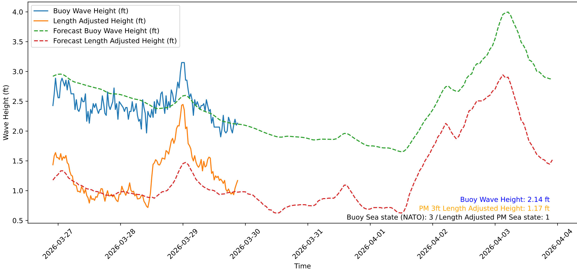
Wave Heights over Time for Oceanside Harbor at 2026-03-29 21:50:32
