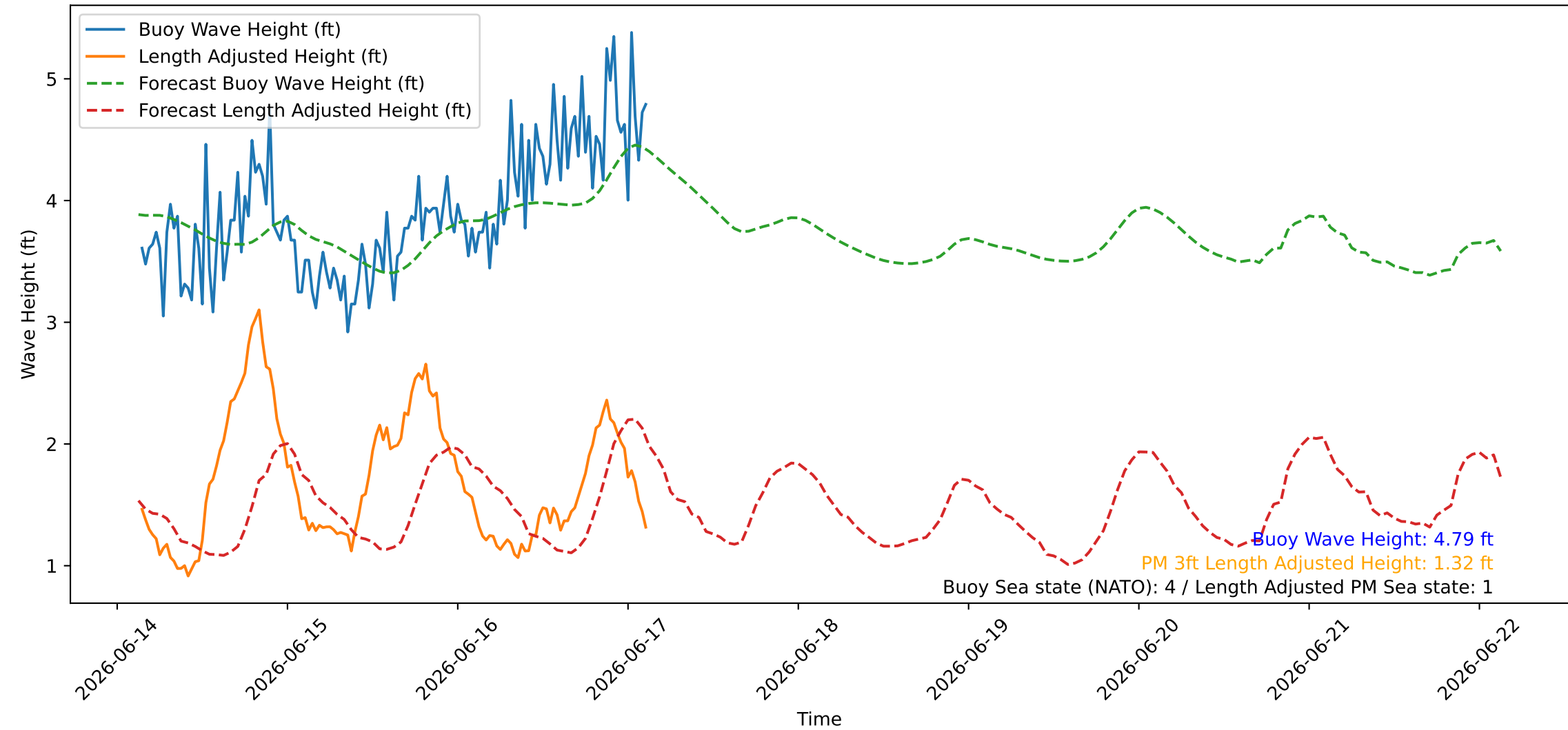
Wave Heights over Time for Red Beach at 2026-06-17 03:10:45
