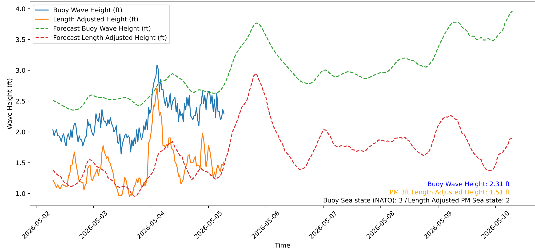
Wave Heights over Time for Oceanside Harbor at 2026-05-05 07:00:32
