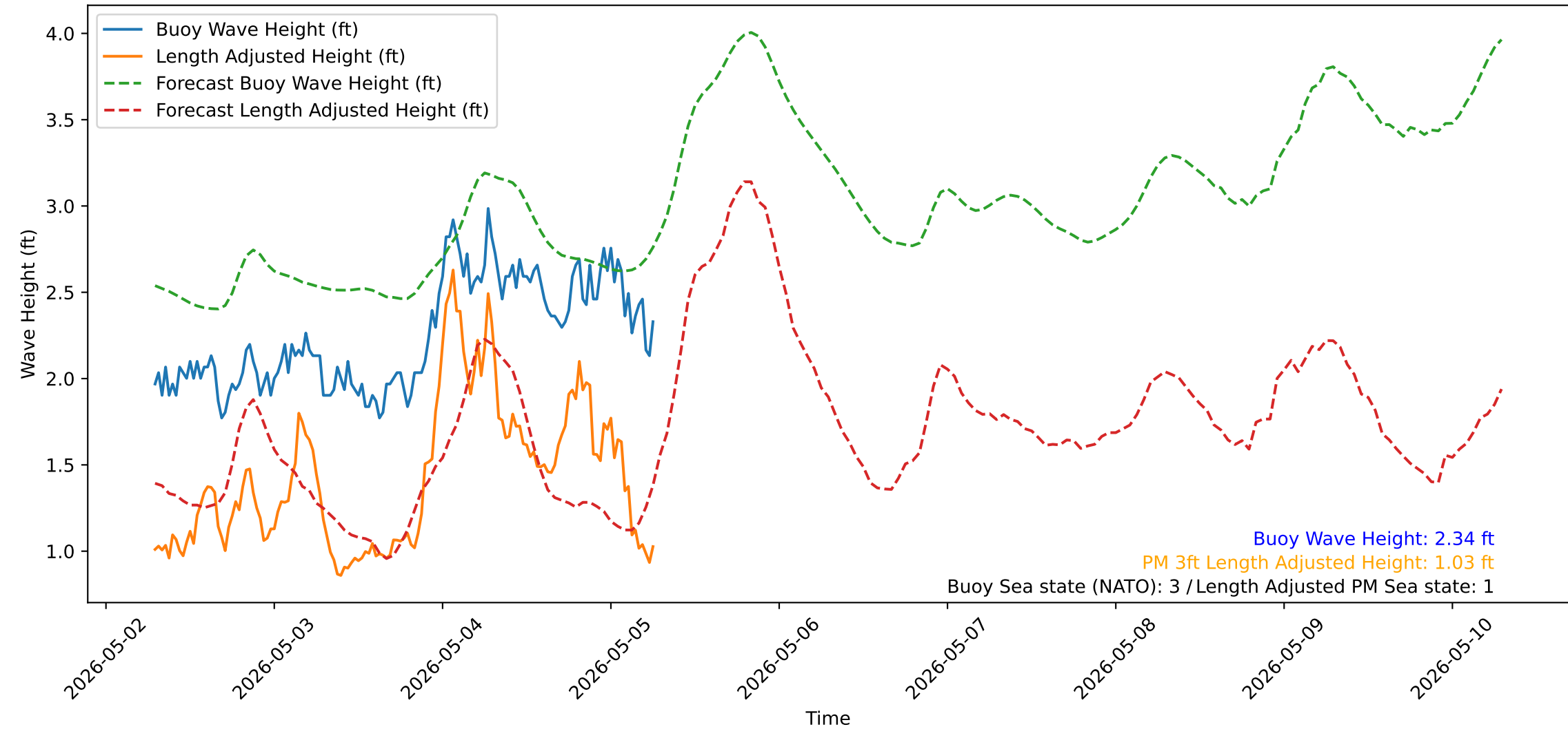
Wave Heights over Time for Green Beach at 2026-05-05 07:01:13
