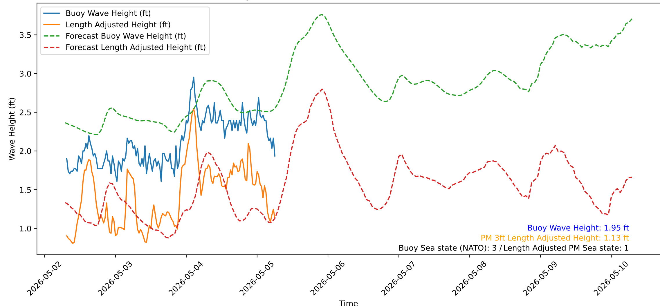
Wave Heights over Time for Red Beach at 2026-05-05 07:00:51
